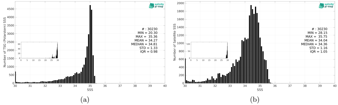
Figure 3: Histograms of SSS from TSG (Polarstern) (a) and SMOS SSS L4 v2 - Daily (BEC) (b) considering all match-up pairs per bins of 0.1 over the Arctic Ocean Pi-MEP region and for the full satellite product period.
