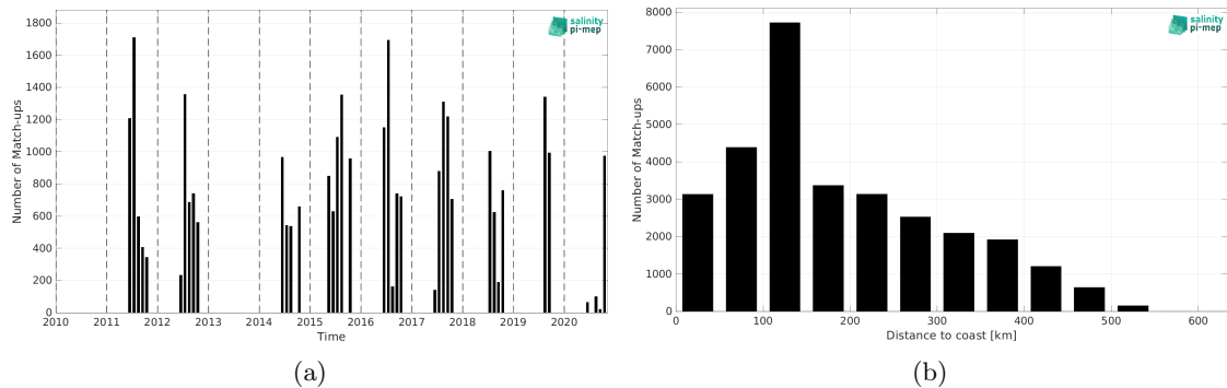
Figure 2: Number of match-ups between TSG (Polarstern) and SMOS SSS L4 v2 - Daily (BEC) SSS as a function of time (a) and as function of the distance to coast (b) over the Arctic Ocean Pi-MEP region and for the full satellite product period.
