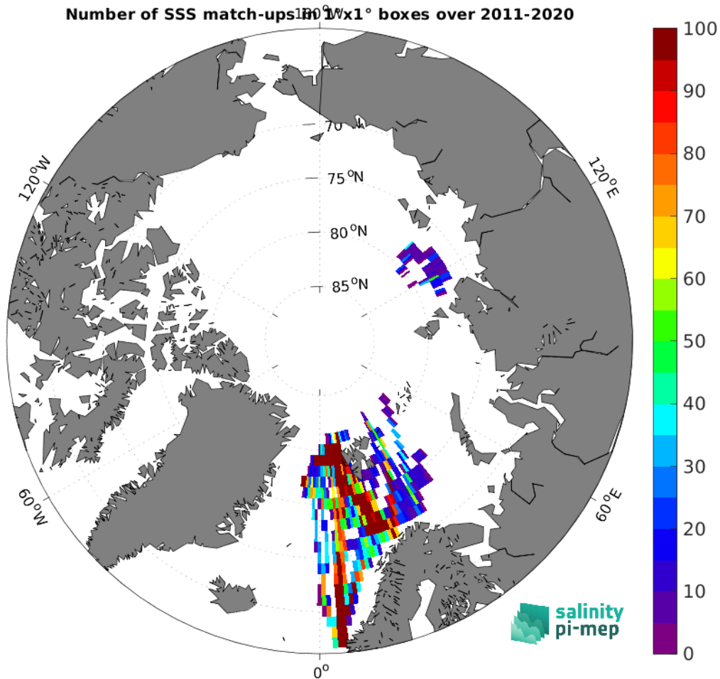
Figure 5: Number of SSS match-ups between TSG (Polarstern) SSS and the SMOS SSS L4 v2 - Daily (BEC) SSS product for the Arctic Ocean Pi-MEP region over 1^\circ \times 1^\circ boxes and for the full satellite product period.
