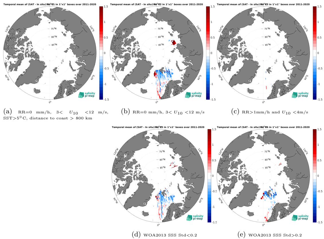
Figure 14: Temporal mean gridded over spatial boxes of size 1^\circ \times 1^\circ of \Delta SSS (SMOS SSS L4 v2 - Daily (BEC) - TSG (Polarstern)) for 5 different subdatasets corresponding to: RR=0 mm/h, 3 < U_{10} < 12 m/s, SST > 5°C, distance to coast > 800 km (a), RR=0 mm/h, 3 < U_{10} < 12 m/s (b), RR > 1mm/h and U_{10} < 4 m/s (c), WOA2013 SSS Std < 0.2 (d), WOA2013 SSS Std > 0.2 (e).
