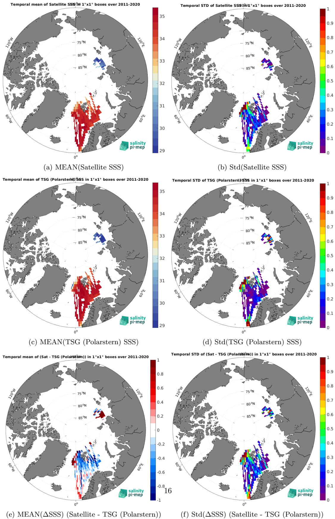
Figure 7: Temporal mean (left) and Std (right) of SSS from SMOS SSS L4 v2 - Daily (BEC) (top), TSG (Polarstern) (middle), and of \Delta SSS (Satellite - TSG (Polarstern)). Only match-up pairs are used to generate these maps.
