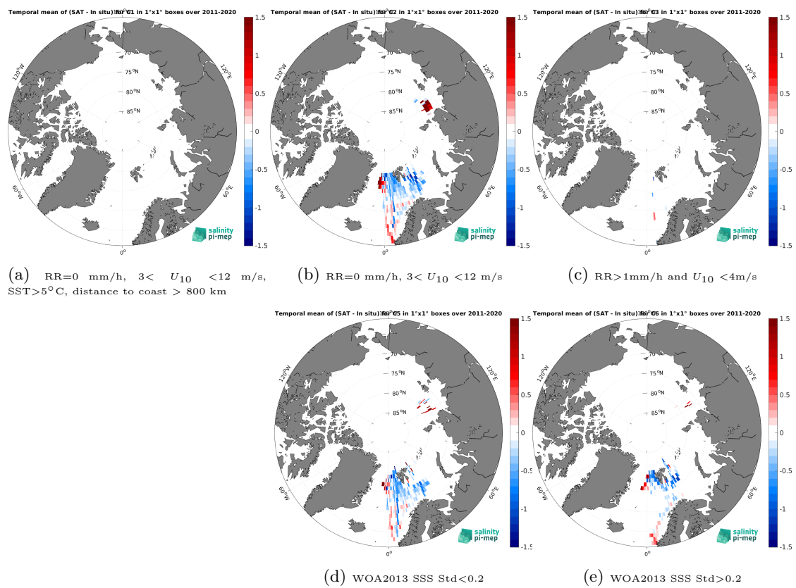
Figure 14: Temporal mean gridded over spatial boxes of size 1^\circ \times 1^\circ of \Delta\text{SSS} (SMOS SSS L4 v2 - Daily (BEC) - TSG (Polarstern)) for 5 different subdatasets corresponding to:RR=0 mm/h, 3 < U_{10} < 12 m/s, SST>5°C, distance to coast > 800 km (a), RR=0 mm/h, 3 < U_{10} < 12 m/s (b), RR>1mm/h and U_{10} < 4 m/s (c), WOA2013 SSS Std<0.2 (d), WOA2013 SSS Std>0.2 (e).
