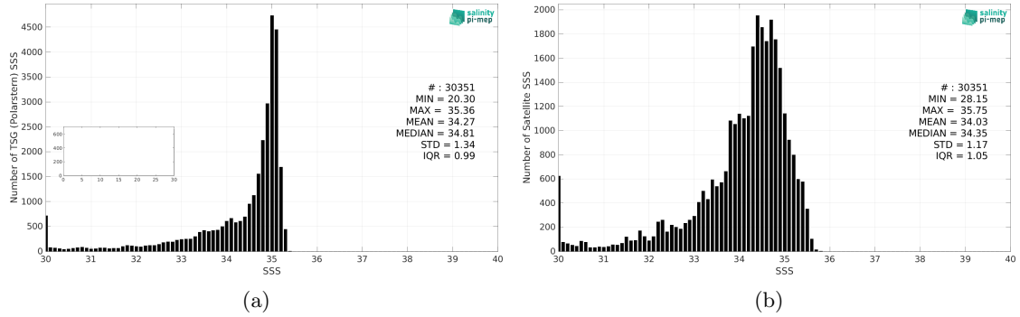
Figure 2: Histograms of SSS from TSG (Polarstern) (a) and SMOS SSS L4 v2 - Daily (BEC) (b) considering all match-up pairs per bins of 0.1 over the Arctic Ocean Pi-MEP region and for the full satellite product period.
