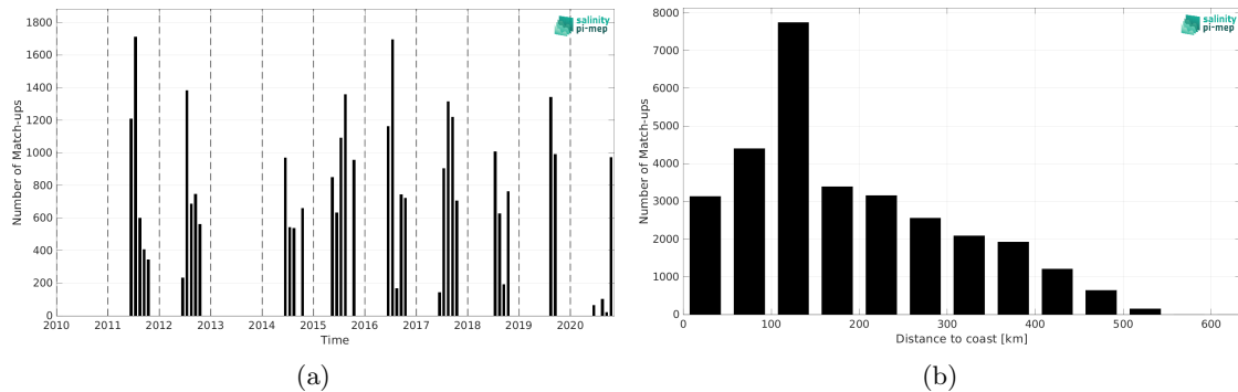
Figure 1: Number of match-ups between TSG (Polarstern) and SMOS SSS L4 v2 - Daily (BEC) SSS as a function of time (a) and as function of the distance to coast (b) over the Arctic Ocean Pi-MEP region and for the full satellite product period.
