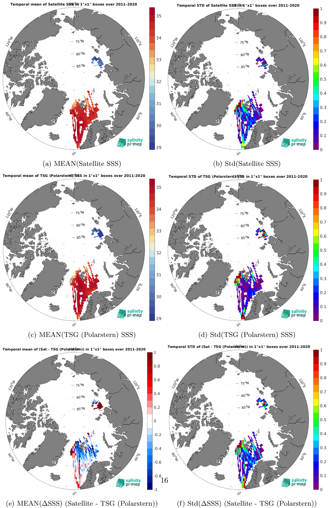
Figure 6: Temporal mean (left) and Std (right) of SSS from SMOS SSS L4 v2 - Daily (BEC) (top), TSG (Polarstern) (middle), and of \Delta SSS (Satellite - TSG (Polarstern)). Only match-up pairs are used to generate these maps.
