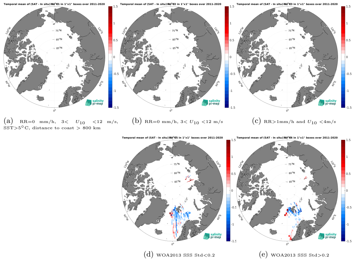
Figure 12: Temporal mean gridded over spatial boxes of size 1^{\circ}\times 1^{\circ} of \Delta\text{SSS} (SMOS SSS L4 v2 - Daily (BEC) - TSG (Polarstern)) for 5 different subdatasets corresponding to:RR=0 mm/h, 3 < U_{10} < 12 m/s, SST > 5^{\circ}\text{C} , distance to coast > 800 km (a), RR=0 mm/h, 3 < U_{10} < 12 m/s (b), RR > 1 mm/h and U_{10} < 4 m/s (c), WOA2013 SSS Std < 0.2 (d), WOA2013 SSS Std > 0.2 (e).
