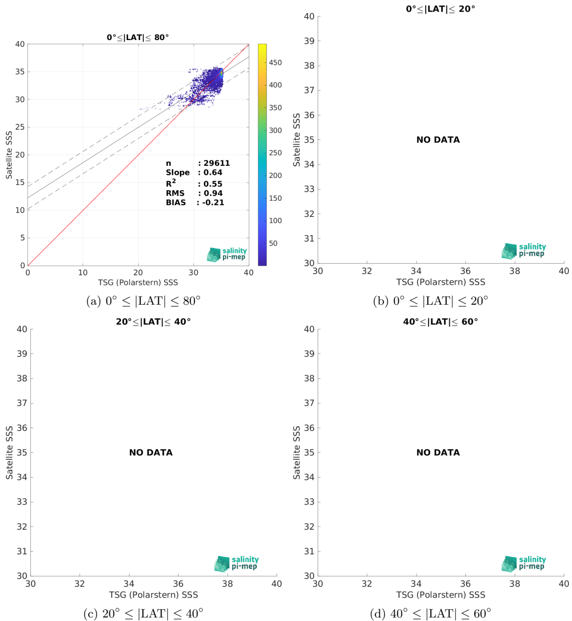
Figure 9: Contour maps of the concentration of SMOS SSS L4 v2 - Daily (BEC) SSS (y-axis) versus TSG (Polarstern) SSS (x-axis) at match-up pairs for different latitude bands. For each plot, the red line shows x=y . The black thin and dashed lines indicate a linear fit through the data cloud and the \pm 95\% confidence levels, respectively. The number match-up pairs n , the slope and R^2 coefficient of the linear fit, the root mean square (RMS) and the mean bias between satellite and in situ data are indicated for each latitude band in each plots.
