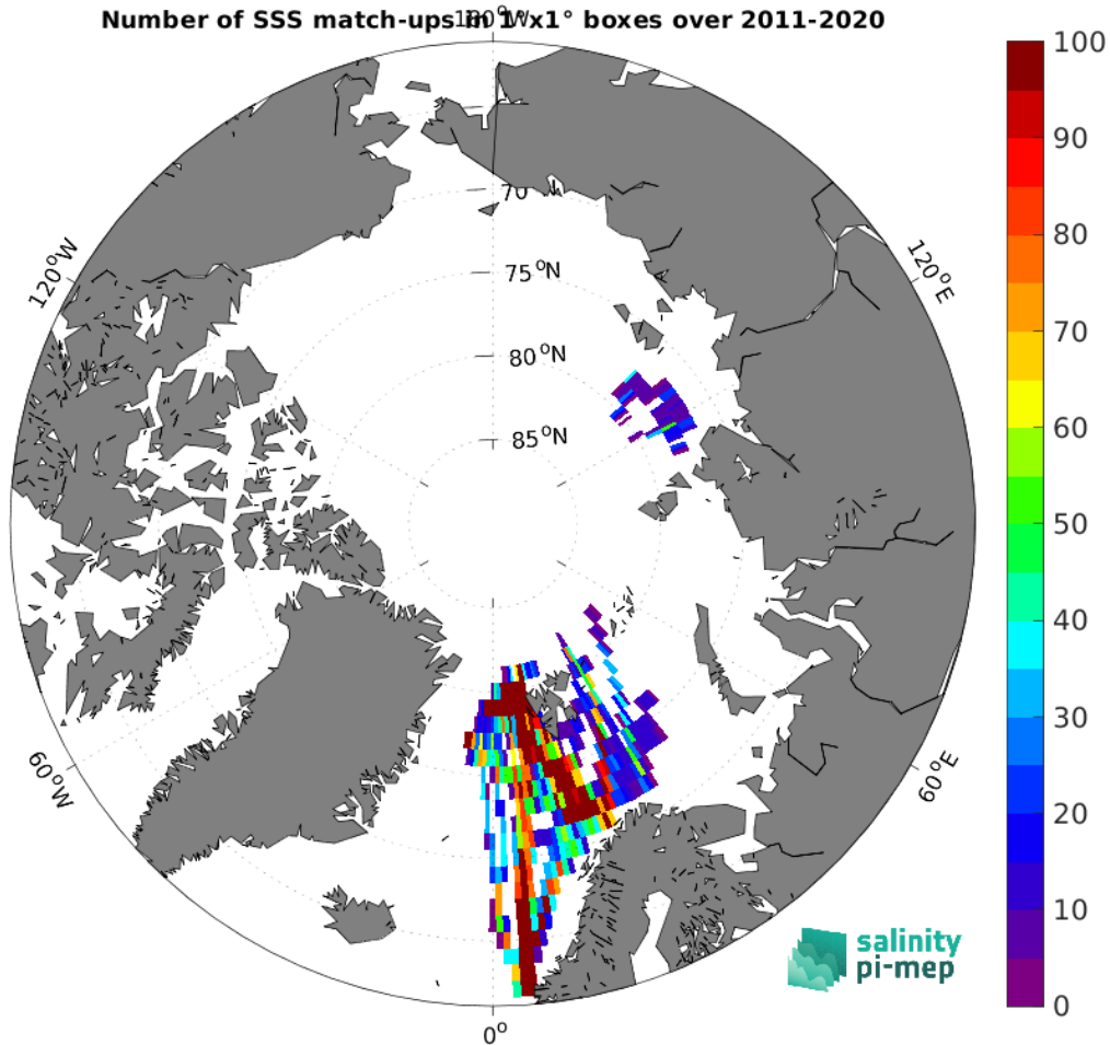
Figure 4: Number of SSS match-ups between TSG (Polarstern) SSS and the SMOS SSS L4 v2 - Daily (BEC) SSS product for the Arctic Ocean Pi-MEP region over 1^\circ \times 1^\circ boxes and for the full satellite product period.
