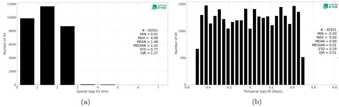
Figure 5: Histograms of the spatial (a) and temporal (b) lags between the location/time of the TSG (Polarstern) measurement and the date of the corresponding SMOS SSS L4 v2 - Daily (BEC) SSS pixel.
