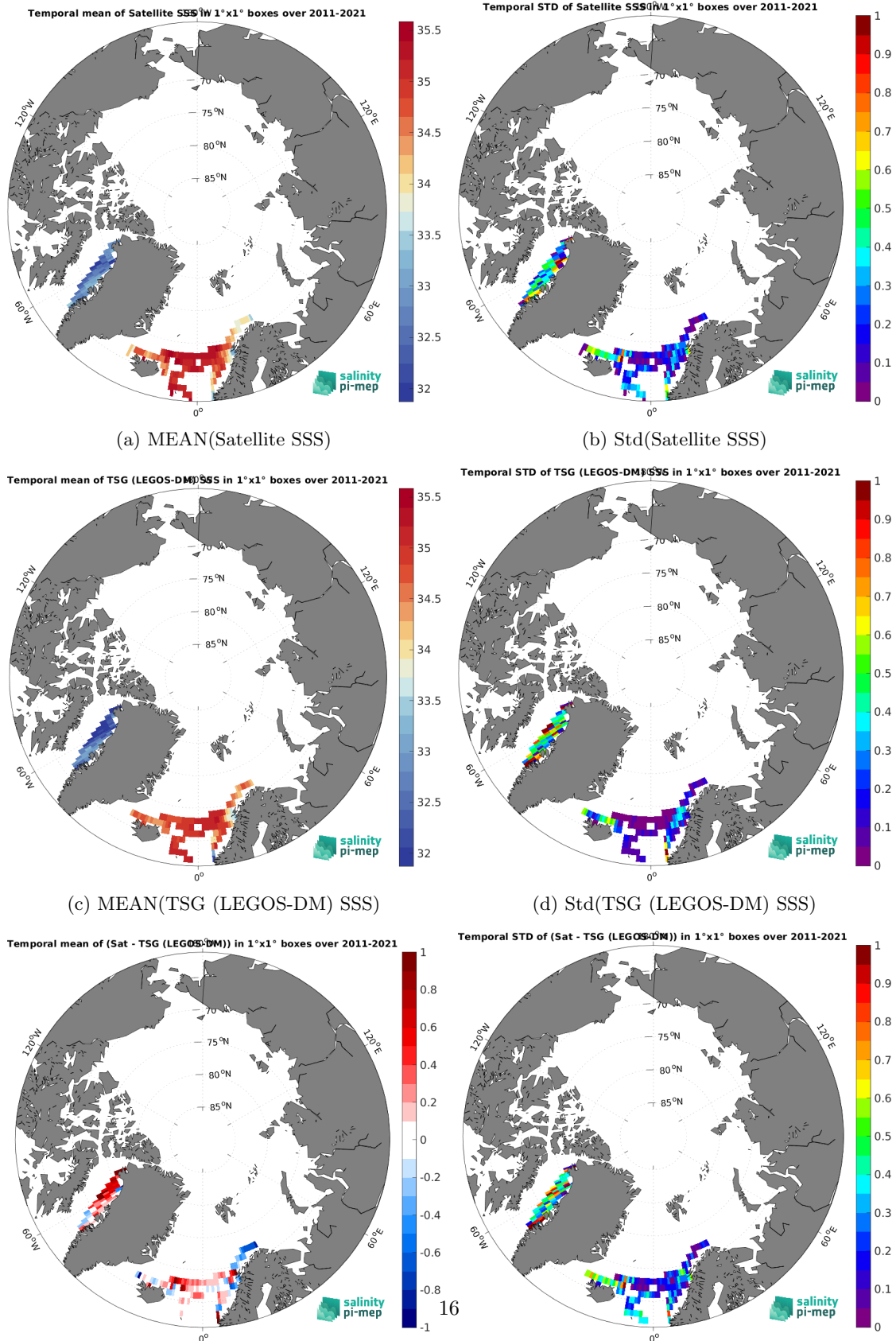
(e) MEAN( \Delta SSS) (Satellite - TSG (LEGOS-DM)) (f) Std( \Delta SSS) (Satellite - TSG (LEGOS-DM)) Figure 7: Temporal mean (left) and Std (right) of SSS from SMOS SSS L4 v2 - Daily (BEC) (top), TSG (LEGOS-DM) (middle), and of \Delta SSS (Satellite - TSG (LEGOS-DM)). Only match-up pairs are used to generate these maps.
