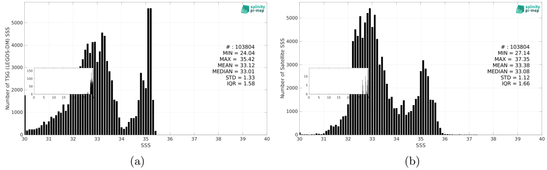
Figure 3: Histograms of SSS from TSG (LEGOS-DM) (a) and SMOS SSS L4 v2 - Daily (BEC) (b) considering all match-up pairs per bins of 0.1 over the Arctic Ocean Pi-MEP region and for the full satellite product period.
