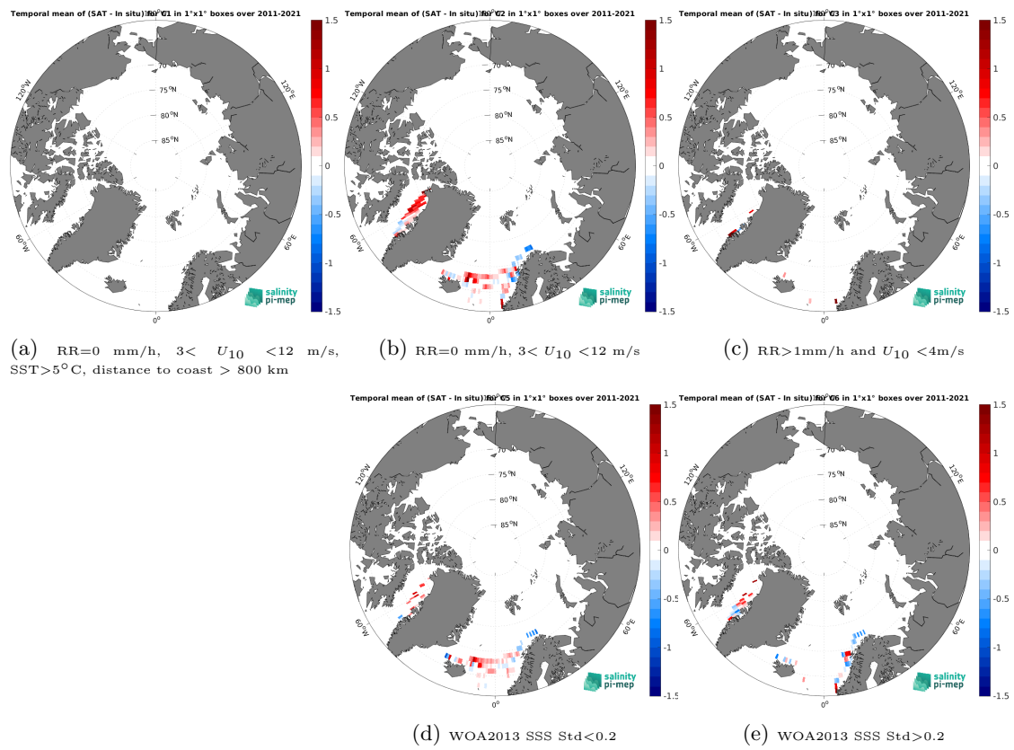
Figure 14: Temporal mean gridded over spatial boxes of size 1^\circ \times 1^\circ of \Delta SSS (SMOS SSS L4 v2 - Daily (BEC) - TSG (LEGOS-DM)) for 5 different subdatasets corresponding to:RR=0 mm/h, 3 < U_{10} < 12 m/s, SST>5°C, distance to coast > 800 km (a), RR=0 mm/h, 3 < U_{10} < 12 m/s (b), RR>1mm/h and U_{10} < 4 m/s (c), WOA2013 SSS Std<0.2 (d), WOA2013 SSS Std>0.2 (e).
