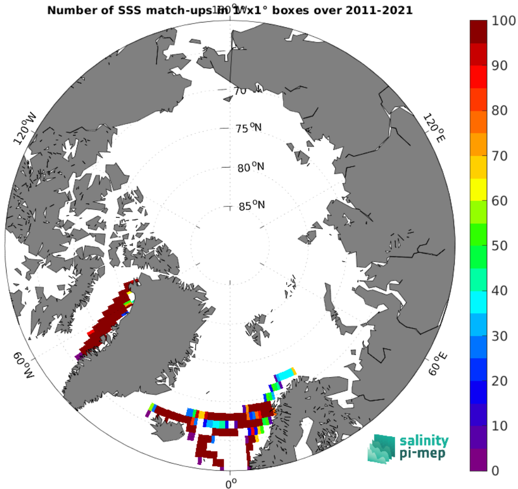
Figure 5: Number of SSS match-ups between TSG (LEGOS-DM) SSS and the SMOS SSS L4 v2 - Daily (BEC) SSS product for the Arctic Ocean Pi-MEP region over 1^\circ \times 1^\circ boxes and for the full satellite product period.
