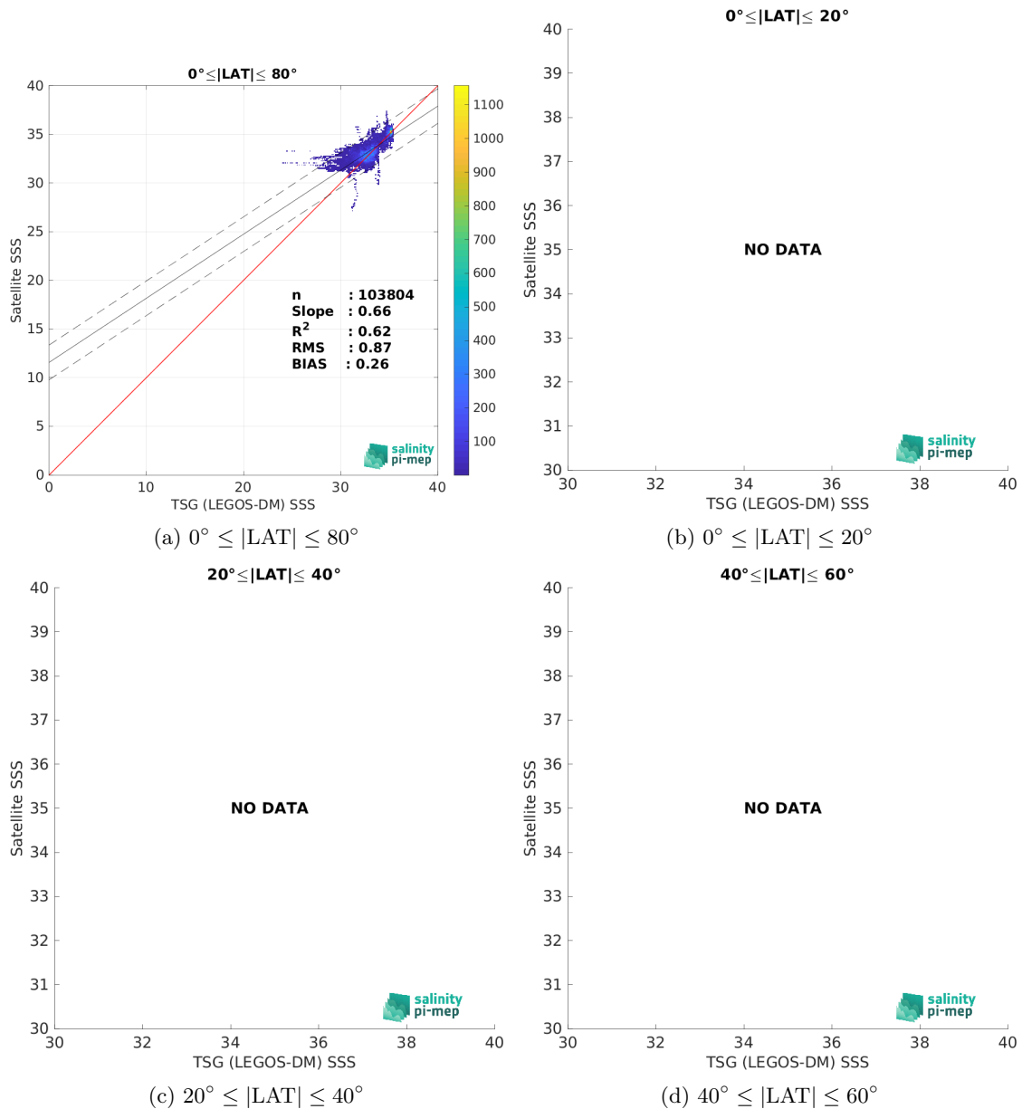
Figure 10: Contour maps of the concentration of SMOS SSS L4 v2 - Daily (BEC) SSS (y-axis) versus TSG (LEGOS-DM) SSS (x-axis) at match-up pairs for different latitude bands. For each plot, the red line shows x=y . The black thin and dashed lines indicate a linear fit through the data cloud and the \pm 95\% confidence levels, respectively. The number match-up pairs n , the slope and R^2 coefficient of the linear fit, the root mean square (RMS) and the mean bias between satellite and in situ data are indicated for each latitude band in each plots.
