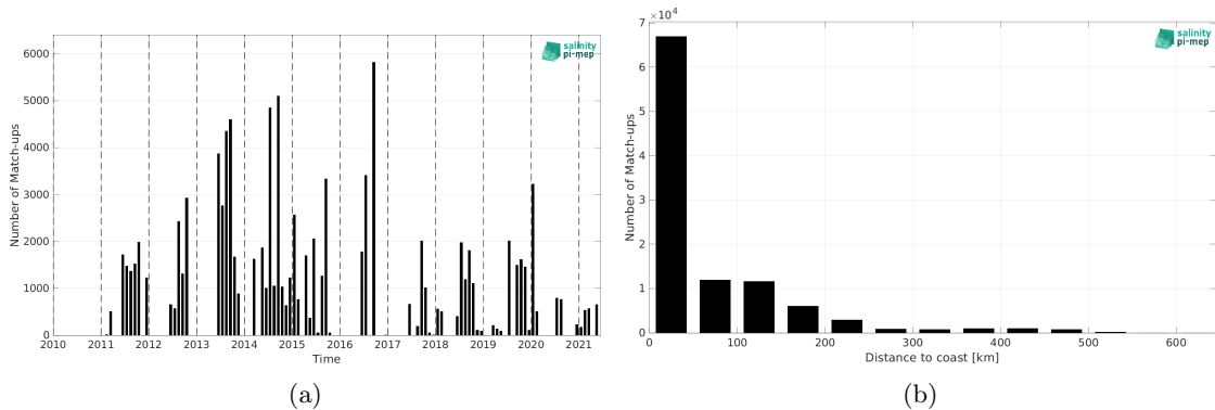
Figure 2: Number of match-ups between TSG (LEGOS-DM) and SMOS SSS L4 v2 - Daily (BEC) SSS as a function of time (a) and as function of the distance to coast (b) over the Arctic Ocean Pi-MEP region and for the full satellite product period.
