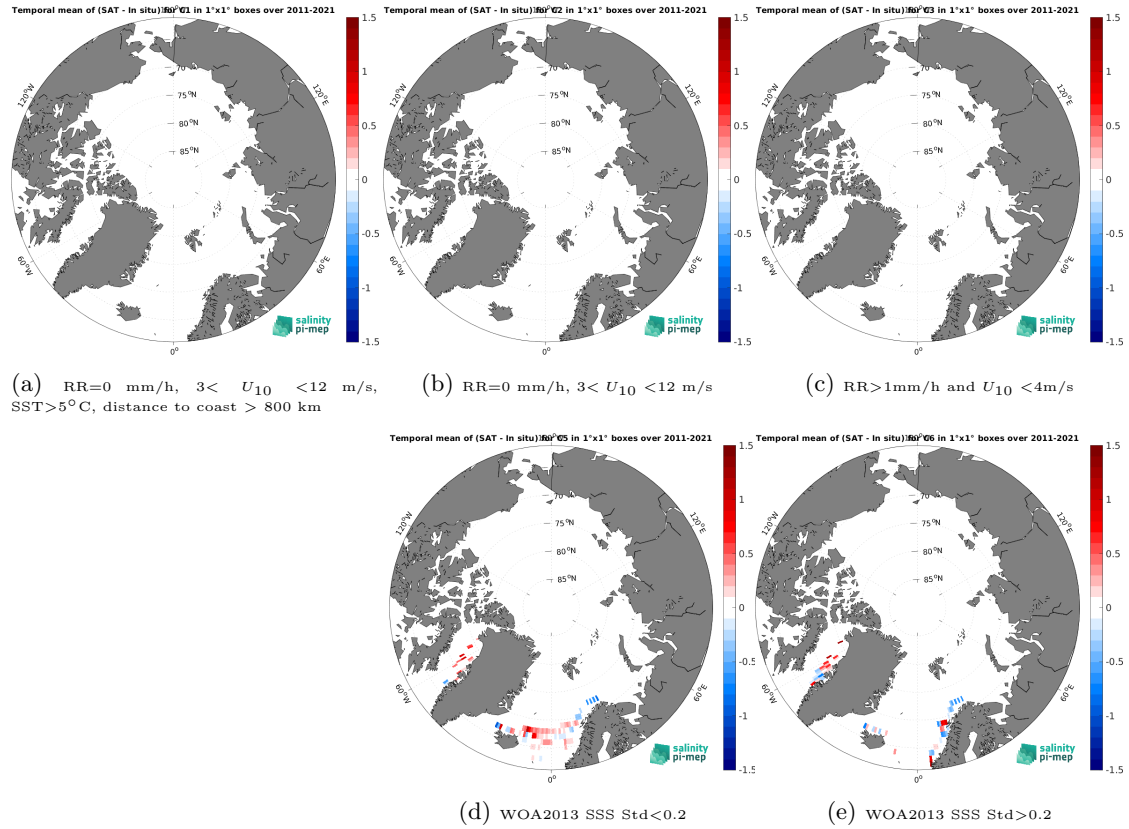
Figure 12: Temporal mean gridded over spatial boxes of size 1^{\circ}\times 1^{\circ} of \Delta\text{SSS} (SMOS SSS L4 v2 - Daily (BEC) - TSG (LEGOS-DM)) for 5 different subdatasets corresponding to:RR=0 mm/h, 3 < U_{10} < 12 m/s, SST > 5^{\circ}\text{C} , distance to coast > 800 km (a), RR=0 mm/h, 3 < U_{10} < 12 m/s (b), RR > 1 mm/h and U_{10} < 4 m/s (c), WOA2013 SSS Std < 0.2 (d), WOA2013 SSS Std > 0.2 (e).
