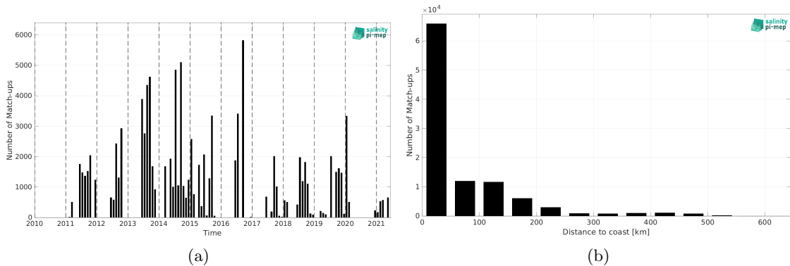
Figure 1: Number of match-ups between TSG (LEGOS-DM) and SMOS SSS L4 v2 - Daily (BEC) SSS as a function of time (a) and as function of the distance to coast (b) over the Arctic Ocean Pi-MEP region and for the full satellite product period.
