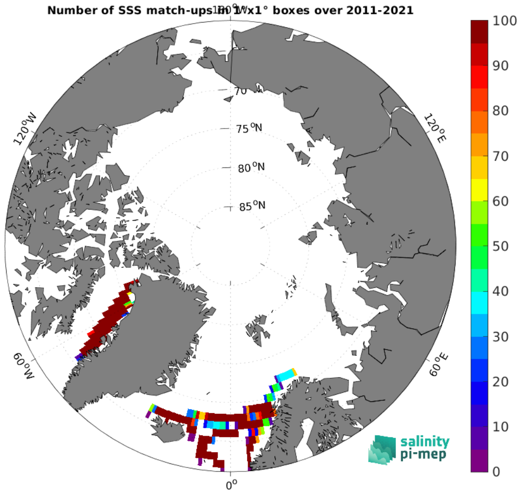
Figure 4: Number of SSS match-ups between TSG (LEGOS-DM) SSS and the SMOS SSS L4 v2 - Daily (BEC) SSS product for the Arctic Ocean Pi-MEP region over 1^\circ \times 1^\circ boxes and for the full satellite product period.
