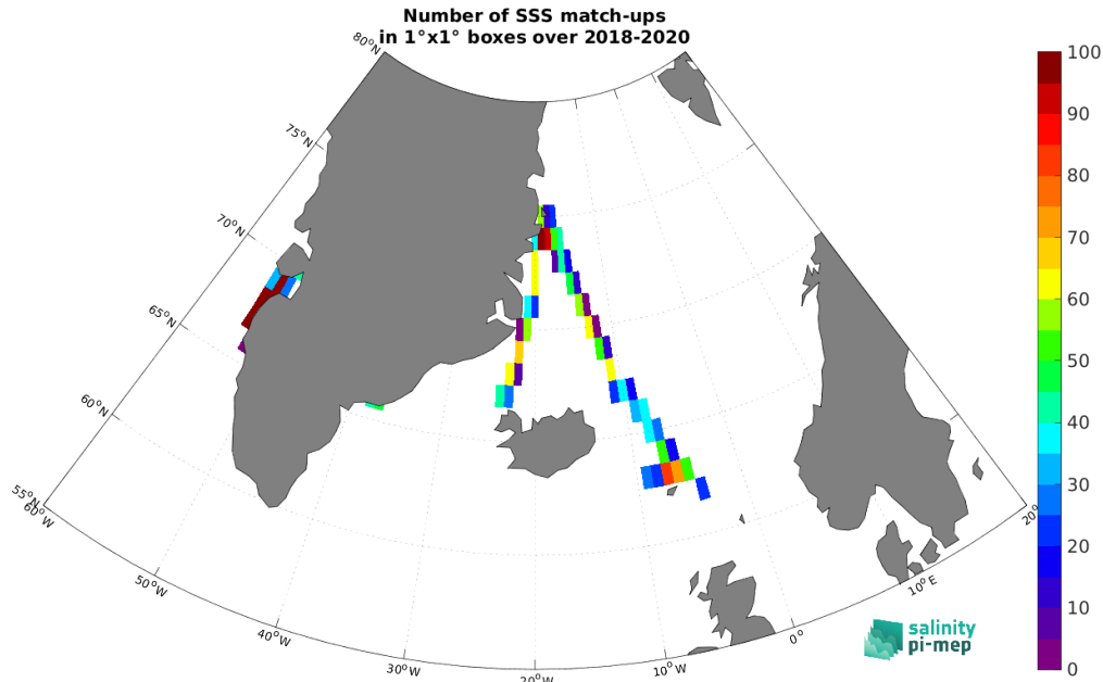
Figure 5: Number of SSS match-ups between TSG (Lauge-Koch) SSS and the SMOS SSS L4 v2 - Daily (BEC) SSS product for the Arctic Ocean Pi-MEP region over 1^\circ \times 1^\circ boxes and for the full satellite product period.
