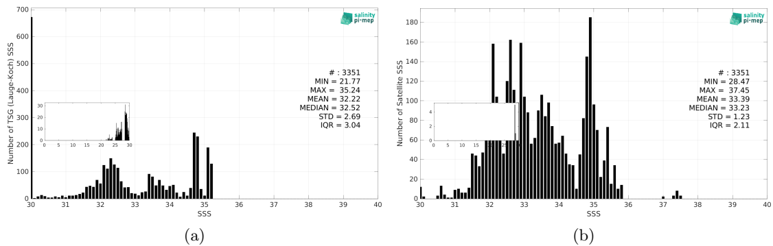
Figure 3: Histograms of SSS from TSG (Lauge-Koch) (a) and SMOS SSS L4 v2 - Daily (BEC) (b) considering all match-up pairs per bins of 0.1 over the Arctic Ocean Pi-MEP region and for the full satellite product period.
