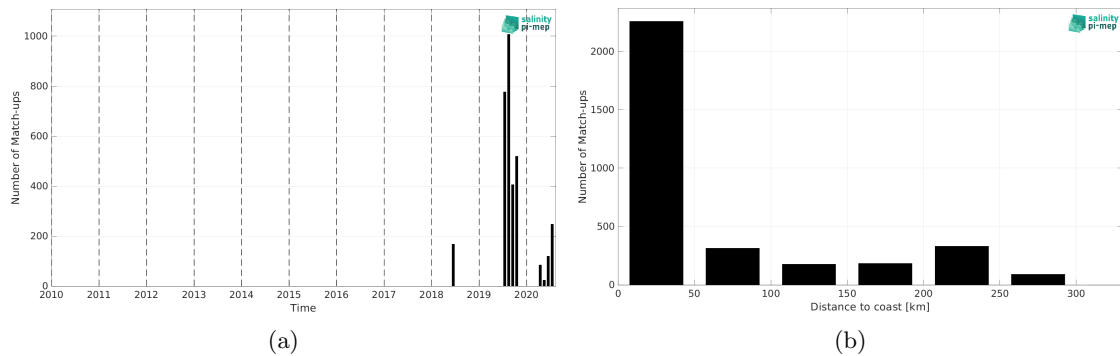
Figure 2: Number of match-ups between TSG (Lauge-Koch) and SMOS SSS L4 v2 - Daily (BEC) SSS as a function of time (a) and as function of the distance to coast (b) over the Arctic Ocean Pi-MEP region and for the full satellite product period.
