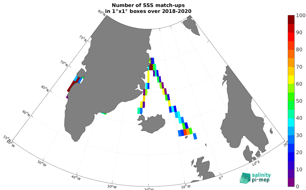
Figure 4: Number of SSS match-ups between TSG (Lauge-Koch) SSS and the SMOS SSS L4 v2 - Daily (BEC) SSS product for the Arctic Ocean Pi-MEP region over 1^\circ \times 1^\circ boxes and for the full satellite product period.
