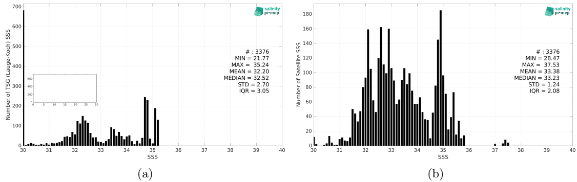
Figure 2: Histograms of SSS from TSG (Lauge-Koch) (a) and SMOS SSS L4 v2 - Daily (BEC) (b) considering all match-up pairs per bins of 0.1 over the Arctic Ocean Pi-MEP region and for the full satellite product period.
