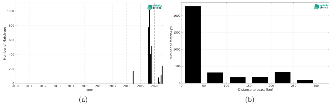
Figure 1: Number of match-ups between TSG (Lauge-Koch) and SMOS SSS L4 v2 - Daily (BEC) SSS as a function of time (a) and as function of the distance to coast (b) over the Arctic Ocean Pi-MEP region and for the full satellite product period.
