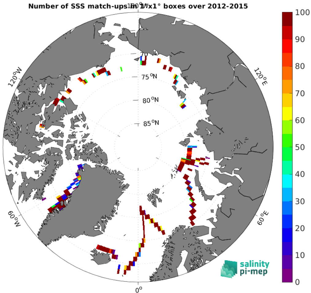
Figure 5: Number of SSS match-ups between TSG (GOSUD-Sailing-ship) SSS and the SMOS SSS L4 v2 - Daily (BEC) SSS product for the Arctic Ocean Pi-MEP region over 1^\circ \times 1^\circ boxes and for the full satellite product period.
