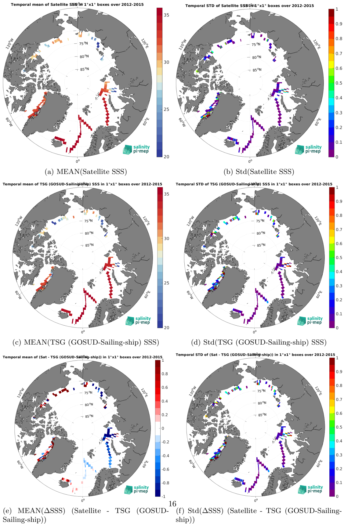
Figure 7: Temporal mean (left) and Std (right) of SSS from SMOS SSS L4 v2 - Daily (BEC) (top), TSG (GOSUD-Sailing-ship) (middle), and of \Delta SSS (Satellite - TSG (GOSUD-Sailing-ship)). Only match-up pairs are used to generate these maps.
