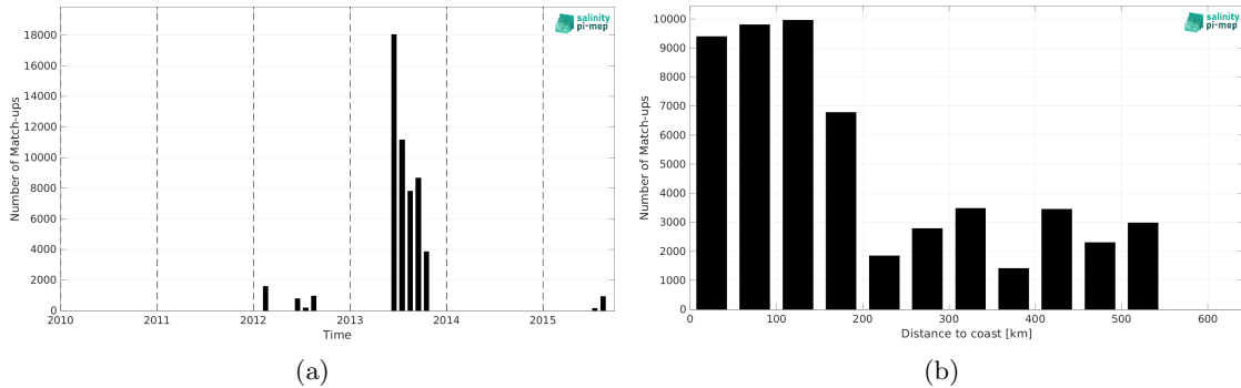
Figure 2: Number of match-ups between TSG (GOSUD-Sailing-ship) and SMOS SSS L4 v2 - Daily (BEC) SSS as a function of time (a) and as function of the distance to coast (b) over the Arctic Ocean Pi-MEP region and for the full satellite product period.
