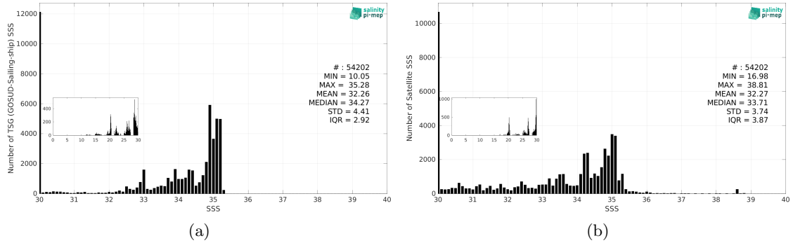
Figure 3: Histograms of SSS from TSG (GOSUD-Sailing-ship) (a) and SMOS SSS L4 v2 - Daily (BEC) (b) considering all match-up pairs per bins of 0.1 over the Arctic Ocean Pi-MEP region and for the full satellite product period.
