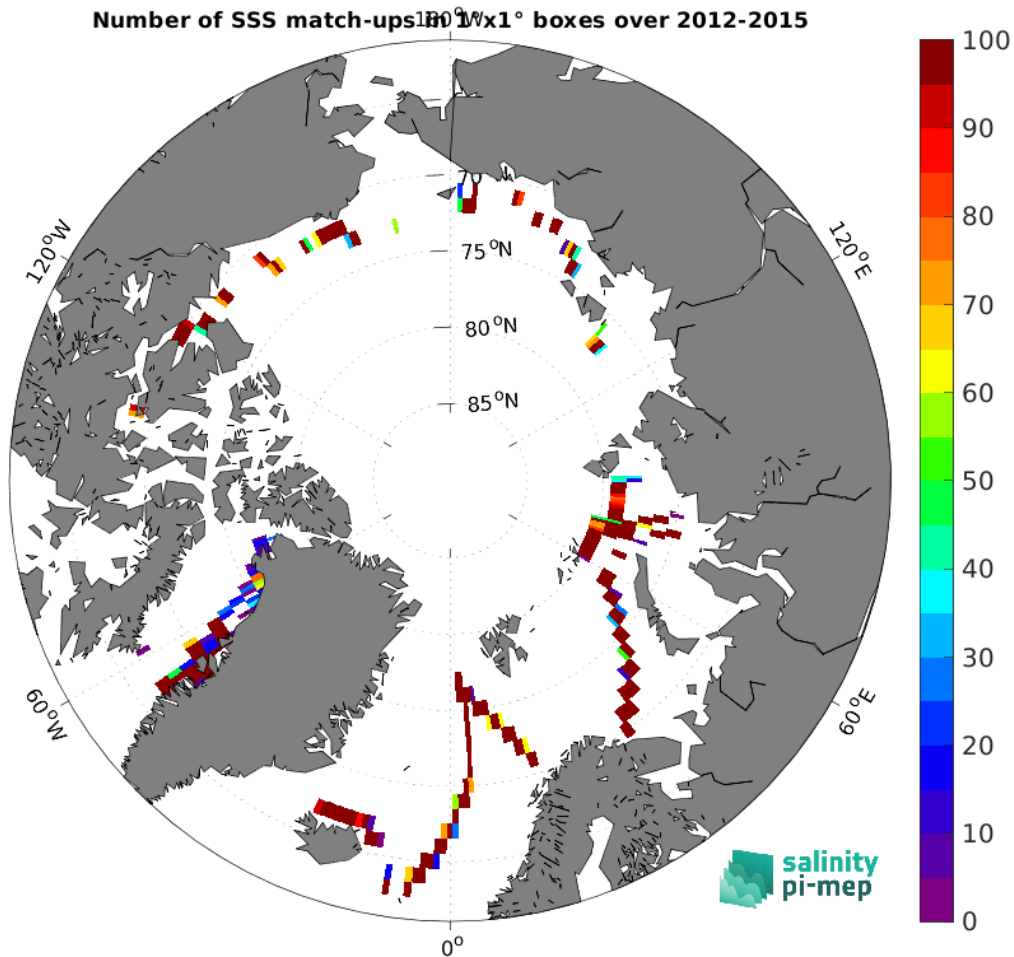
Figure 4: Number of SSS match-ups between TSG (GOSUD-Sailing-ship) SSS and the SMOS SSS L4 v2 - Daily (BEC) SSS product for the Arctic Ocean Pi-MEP region over 1^\circ \times 1^\circ boxes and for the full satellite product period.
