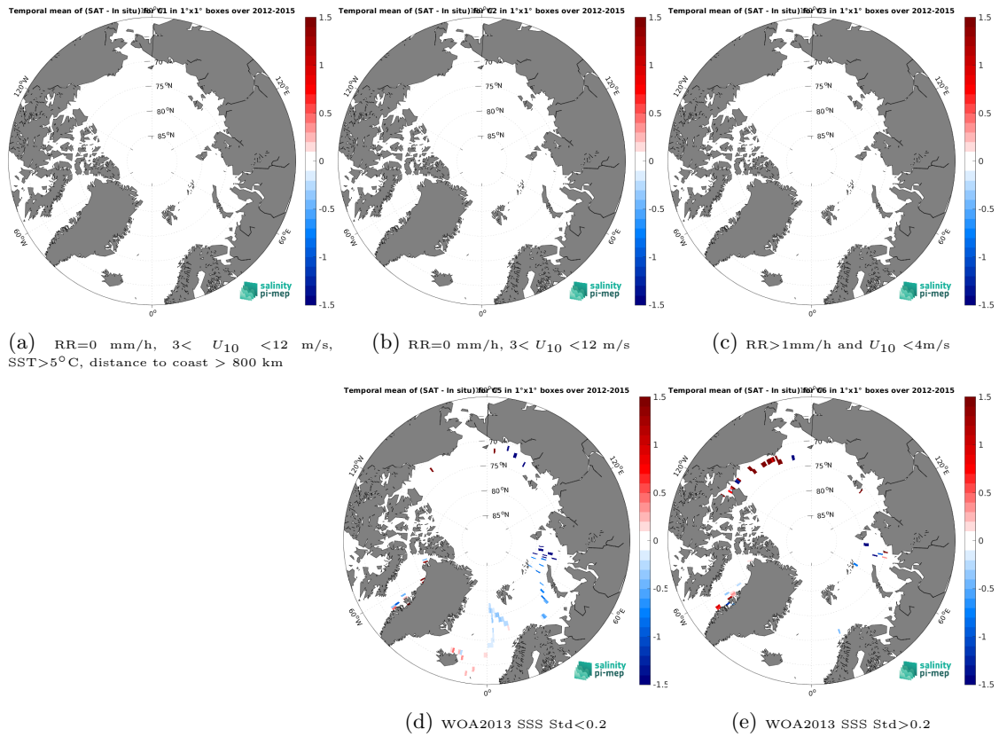
Figure 12: Temporal mean gridded over spatial boxes of size 1^\circ \times 1^\circ of \Delta\text{SSS} (SMOS SSS L4 v2 - Daily (BEC) - TSG (GOSUD-Sailing-ship)) for 5 different subdatasets corresponding to: RR=0 mm/h, 3 < U_{10} < 12 m/s, SST > 5^\circ\text{C} , distance to coast > 800 km (a), RR=0 mm/h, 3 < U_{10} < 12 m/s (b), RR > 1 mm/h and U_{10} < 4 m/s (c), WOA2013 SSS Std < 0.2 (d), WOA2013 SSS Std > 0.2 (e).
