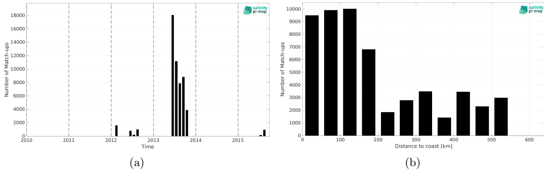
Figure 1: Number of match-ups between TSG (GOSUD-Sailing-ship) and SMOS SSS L4 v2 - Daily (BEC) SSS as a function of time (a) and as function of the distance to coast (b) over the Arctic Ocean Pi-MEP region and for the full satellite product period.
