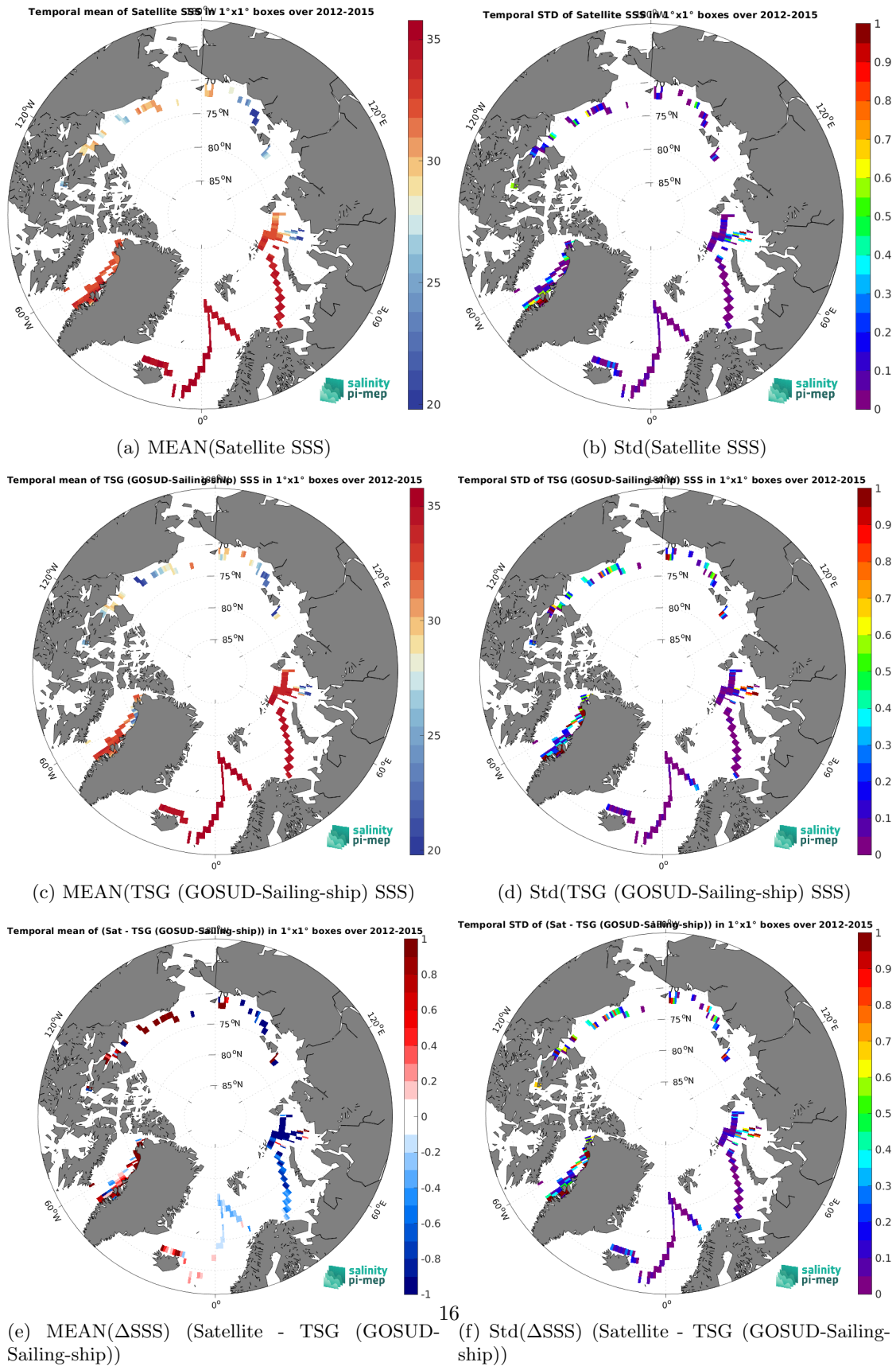
Figure 6: Temporal mean (left) and Std (right) of SSS from SMOS SSS L4 v2 - Daily (BEC) (top), TSG (GOSUD-Sailing-ship) (middle), and of \Delta SSS (Satellite - TSG (GOSUD-Sailing-ship)). Only match-up pairs are used to generate these maps.
