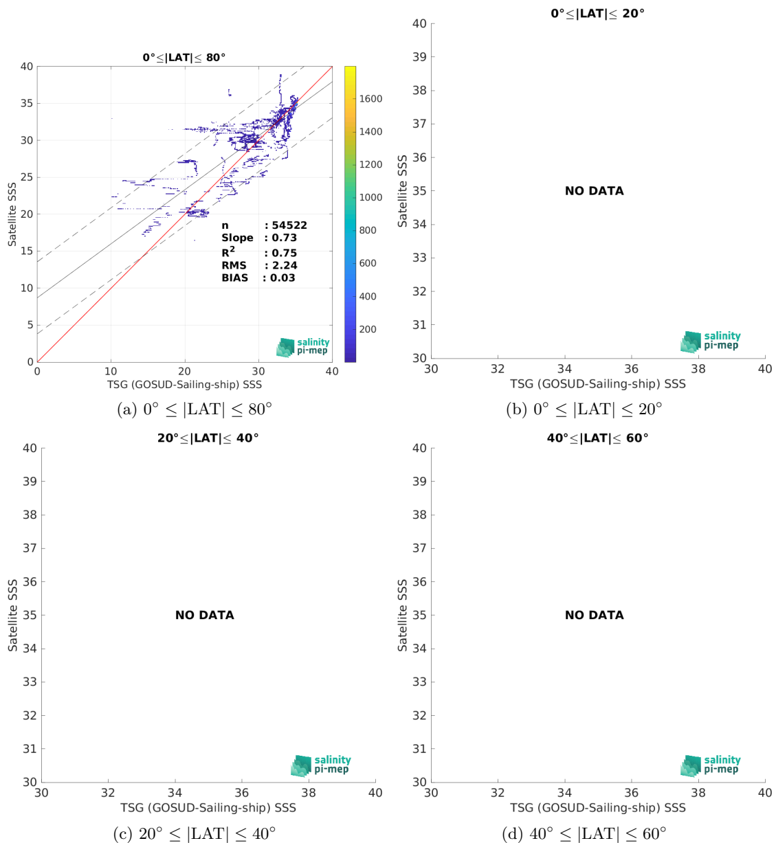
Figure 9: Contour maps of the concentration of SMOS SSS L4 v2 - Daily (BEC) SSS (y-axis) versus TSG (GOSUD-Sailing-ship) SSS (x-axis) at match-up pairs for different latitude bands. For each plot, the red line shows x=y . The black thin and dashed lines indicate a linear fit through the data cloud and the \pm 95\% confidence levels, respectively. The number match-up pairs n , the slope and R^2 coefficient of the linear fit, the root mean square (RMS) and the mean bias between satellite and in situ data are indicated for each latitude band in each plots.
