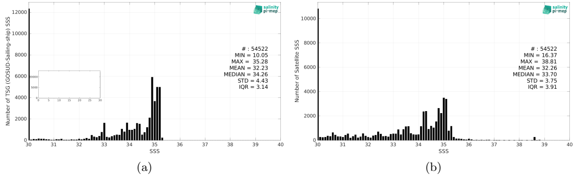
Figure 2: Histograms of SSS from TSG (GOSUD-Sailing-ship) (a) and SMOS SSS L4 v2 - Daily (BEC) (b) considering all match-up pairs per bins of 0.1 over the Arctic Ocean Pi-MEP region and for the full satellite product period.
