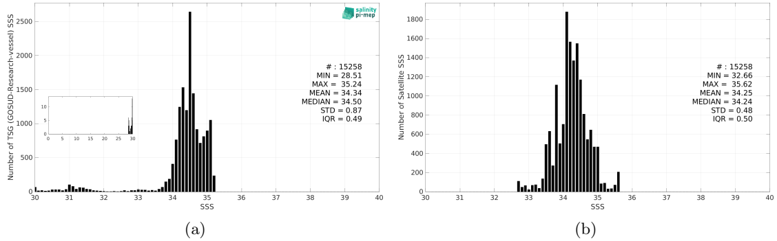
Figure 3: Histograms of SSS from TSG (GOSUD-Research-vessel) (a) and SMOS SSS L4 v2 - Daily (BEC) (b) considering all match-up pairs per bins of 0.1 over the Arctic Ocean Pi-MEP region and for the full satellite product period.
