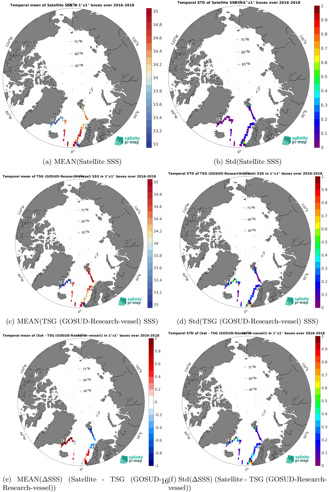
Figure 6: Temporal mean (left) and Std (right) of SSS from SMOS SSS L4 v2 - Daily (BEC) (top), TSG (GOSUD-Research-vessel) (middle), and of \Delta SSS (Satellite - TSG (GOSUD-Research-vessel)). Only match-up pairs are used to generate these maps.
