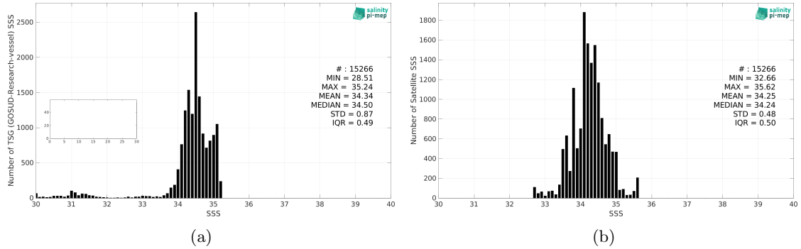
Figure 2: Histograms of SSS from TSG (GOSUD-Research-vessel) (a) and SMOS SSS L4 v2 - Daily (BEC) (b) considering all match-up pairs per bins of 0.1 over the Arctic Ocean Pi-MEP region and for the full satellite product period.
