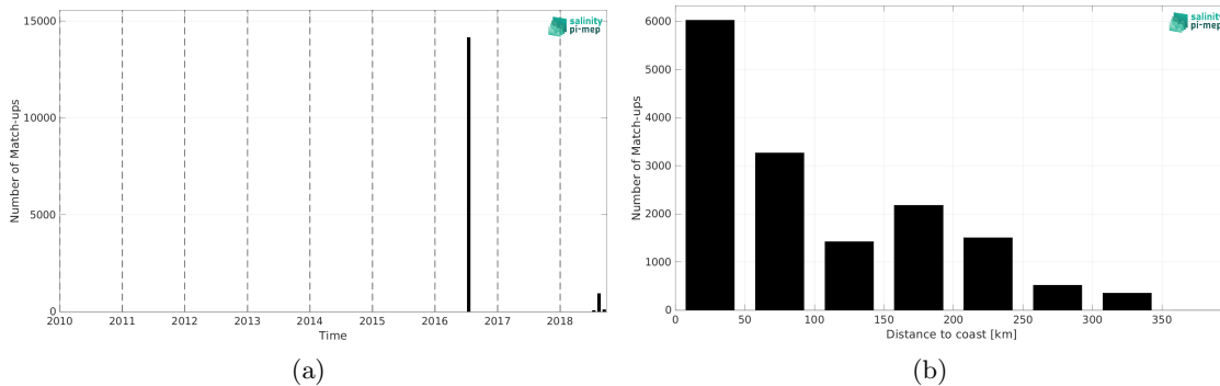
Figure 1: Number of match-ups between TSG (GOSUD-Research-vessel) and SMOS SSS L4 v2 - Daily (BEC) SSS as a function of time (a) and as function of the distance to coast (b) over the Arctic Ocean Pi-MEP region and for the full satellite product period.
