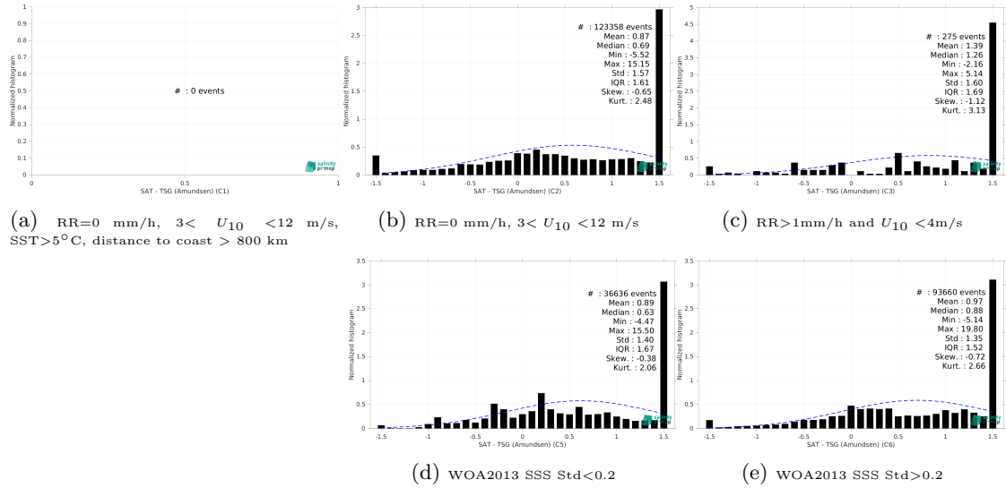
Figure 15: Normalized histogram of \Delta SSS (SMOS SSS L4 v2 - Daily (BEC) - TSG (Amundsen)) for 5 different subdatasets corresponding to: RR=0 mm/h, 3 < U_{10} < 12 m/s, SST > 5°C, distance to coast > 800 km (a), RR=0 mm/h, 3 < U_{10} < 12 m/s (b), RR > 1mm/h and U_{10} < 4 m/s (c), WOA2013 SSS Std < 0.2 (d), WOA2013 SSS Std > 0.2 (e).
