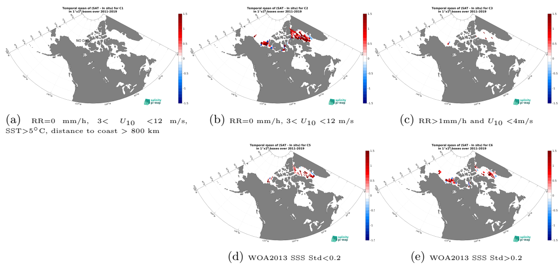
Figure 14: Temporal mean gridded over spatial boxes of size 1^\circ \times 1^\circ of \Delta SSS (SMOS SSS L4 v2 - Daily (BEC) - TSG (Amundsen)) for 5 different subdatasets corresponding to: RR=0 mm/h, 3 < U_{10} < 12 m/s, SST > 5°C, distance to coast > 800 km (a), RR=0 mm/h, 3 < U_{10} < 12 m/s (b), RR > 1mm/h and U_{10} < 4 m/s (c), WOA2013 SSS Std < 0.2 (d), WOA2013 SSS Std > 0.2 (e).
