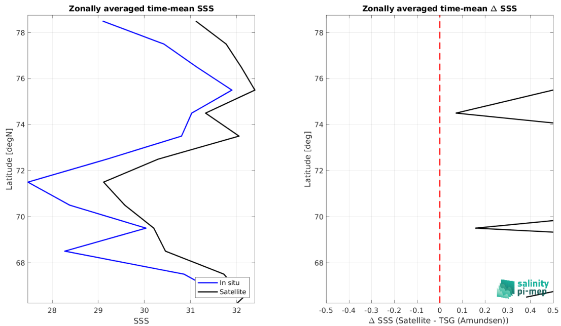
Figure 9: Left panel: Zonal mean SSS from SMOS SSS L4 v2 - Daily (BEC) satellite product (black) and from TSG (Amundsen) (blue). Right panel: Zonal mean of \Delta SSS (Satellite - TSG (Amundsen)) for all the collected Pi-MEP match-up pairs estimated over the full satellite product period.
