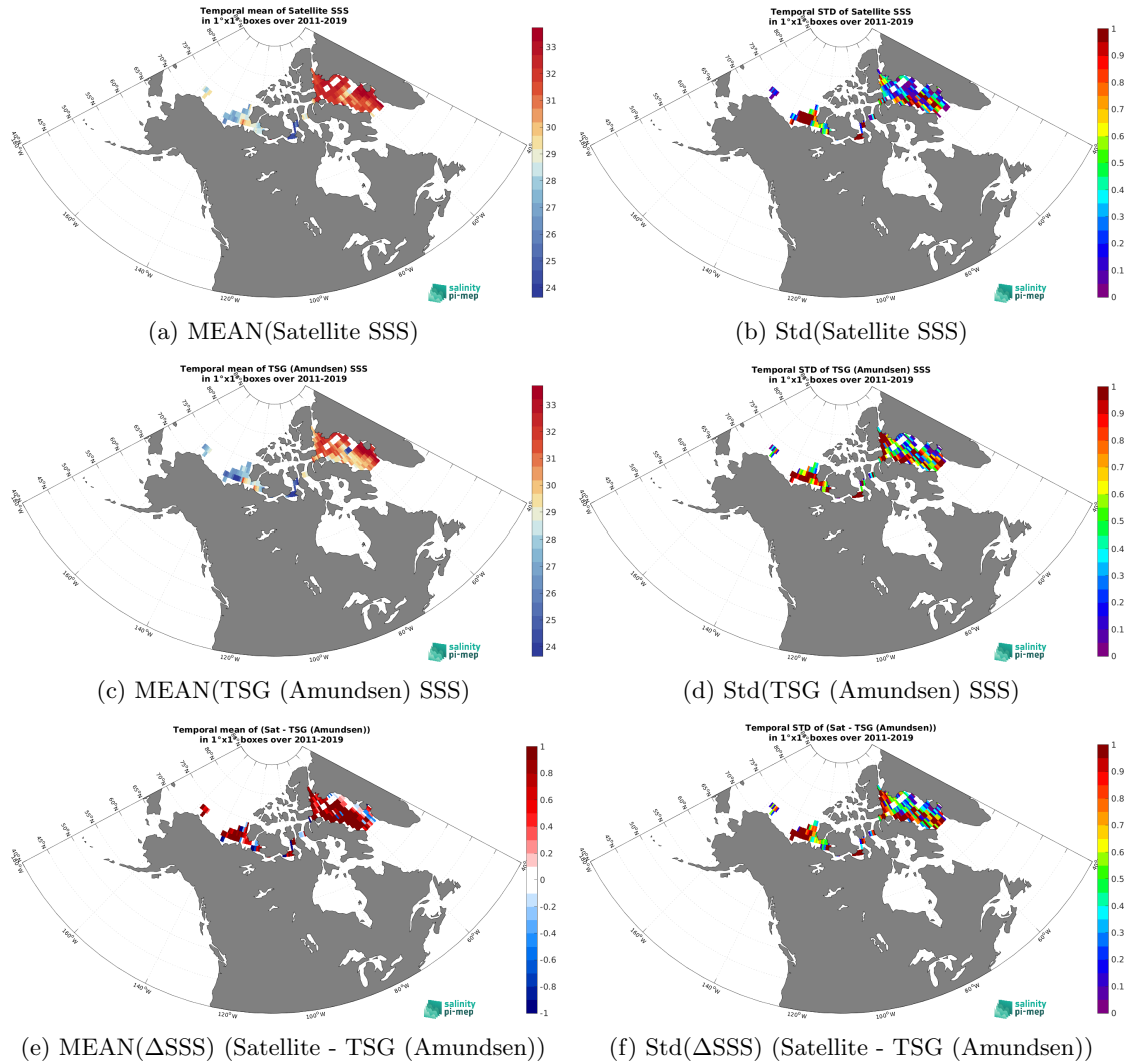
Figure 7: Temporal mean (left) and Std (right) of SSS from SMOS SSS L4 v2 - Daily (BEC) (top), TSG (Amundsen) (middle), and of \Delta SSS (Satellite - TSG (Amundsen)). Only match-up pairs are used to generate these maps.
