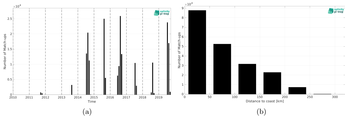
Figure 2: Number of match-ups between TSG (Amundsen) and SMOS SSS L4 v2 - Daily (BEC) SSS as a function of time (a) and as function of the distance to coast (b) over the Arctic Ocean Pi-MEP region and for the full satellite product period.
