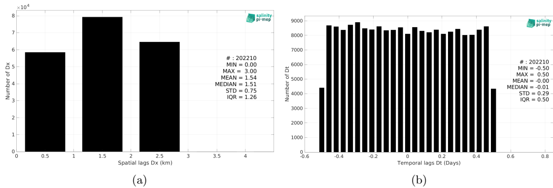
Figure 6: Histograms of the spatial (a) and temporal (b) lags between the location/time of the TSG (Amundsen) measurement and the date of the corresponding SMOS SSS L4 v2 - Daily (BEC) SSS pixel.
