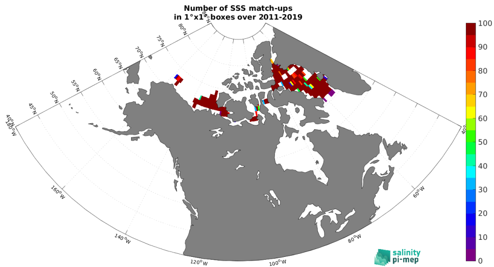
Figure 5: Number of SSS match-ups between TSG (Amundsen) SSS and the SMOS SSS L4 v2 - Daily (BEC) SSS product for the Arctic Ocean Pi-MEP region over 1^\circ \times 1^\circ boxes and for the full satellite product period.
