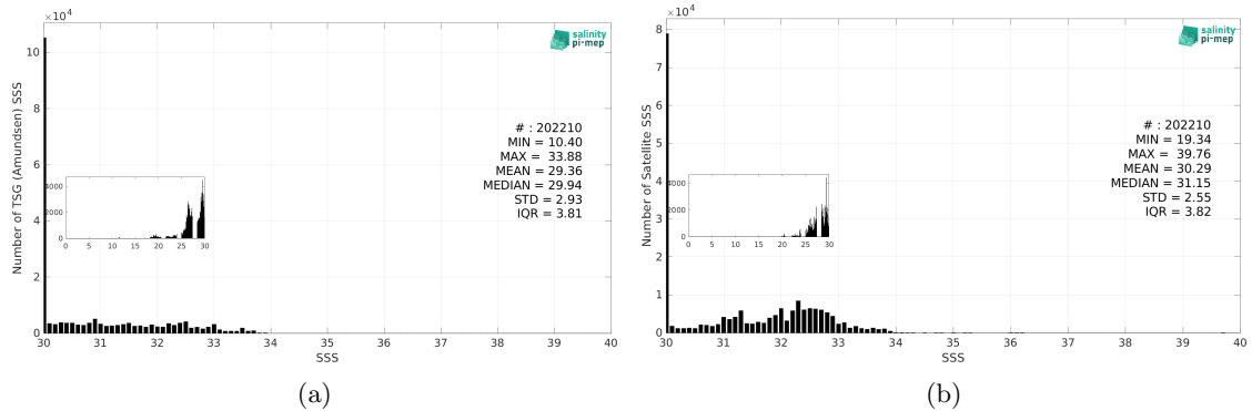
Figure 3: Histograms of SSS from TSG (Amundsen) (a) and SMOS SSS L4 v2 - Daily (BEC) (b) considering all match-up pairs per bins of 0.1 over the Arctic Ocean Pi-MEP region and for the full satellite product period.
