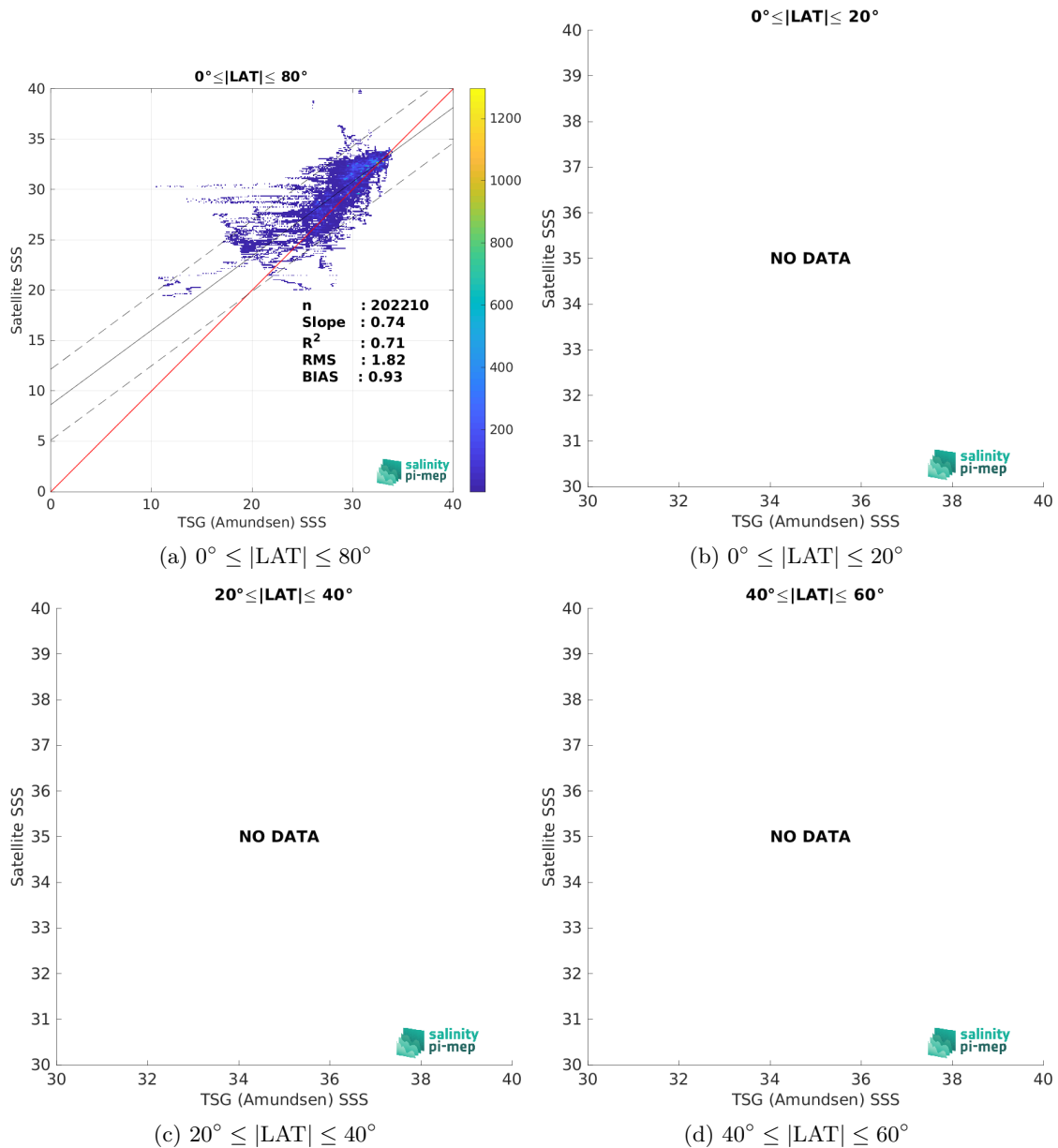
Figure 10: Contour maps of the concentration of SMOS SSS L4 v2 - Daily (BEC) SSS (y-axis) versus TSG (Amundsen) SSS (x-axis) at match-up pairs for different latitude bands. For each plot, the red line shows x=y . The black thin and dashed lines indicate a linear fit through the data cloud and the \pm 95\% confidence levels, respectively. The number match-up pairs n , the slope and R^2 coefficient of the linear fit, the root mean square (RMS) and the mean bias between satellite and in situ data are indicated for each latitude band in each plots.
