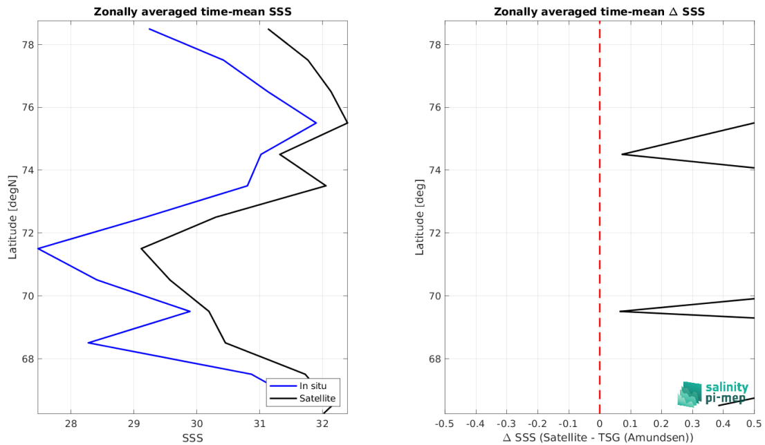
Figure 8: Left panel: Zonal mean SSS from SMOS SSS L4 v2 - Daily (BEC) satellite product (black) and from TSG (Amundsen) (blue). Right panel: Zonal mean of \Delta SSS (Satellite - TSG (Amundsen)) for all the collected Pi-MEP match-up pairs estimated over the full satellite product period.
