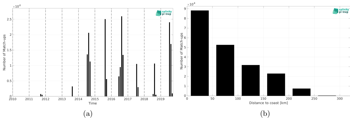
Figure 1: Number of match-ups between TSG (Amundsen) and SMOS SSS L4 v2 - Daily (BEC) SSS as a function of time (a) and as function of the distance to coast (b) over the Arctic Ocean Pi-MEP region and for the full satellite product period.
