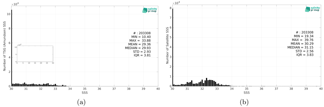
Figure 2: Histograms of SSS from TSG (Amundsen) (a) and SMOS SSS L4 v2 - Daily (BEC) (b) considering all match-up pairs per bins of 0.1 over the Arctic Ocean Pi-MEP region and for the full satellite product period.
