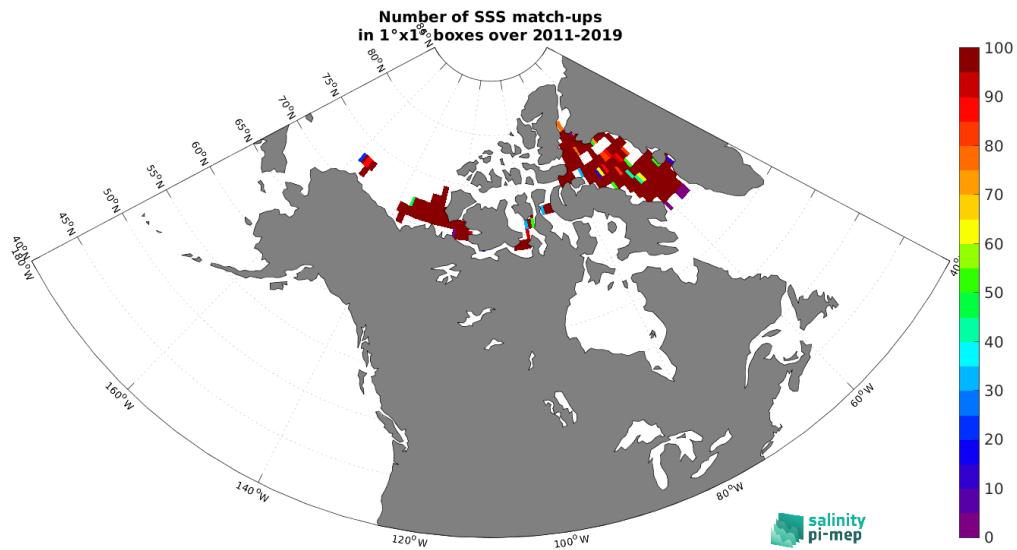
Figure 4: Number of SSS match-ups between TSG (Amundsen) SSS and the SMOS SSS L4 v2 - Daily (BEC) SSS product for the Arctic Ocean Pi-MEP region over 1^\circ \times 1^\circ boxes and for the full satellite product period.
