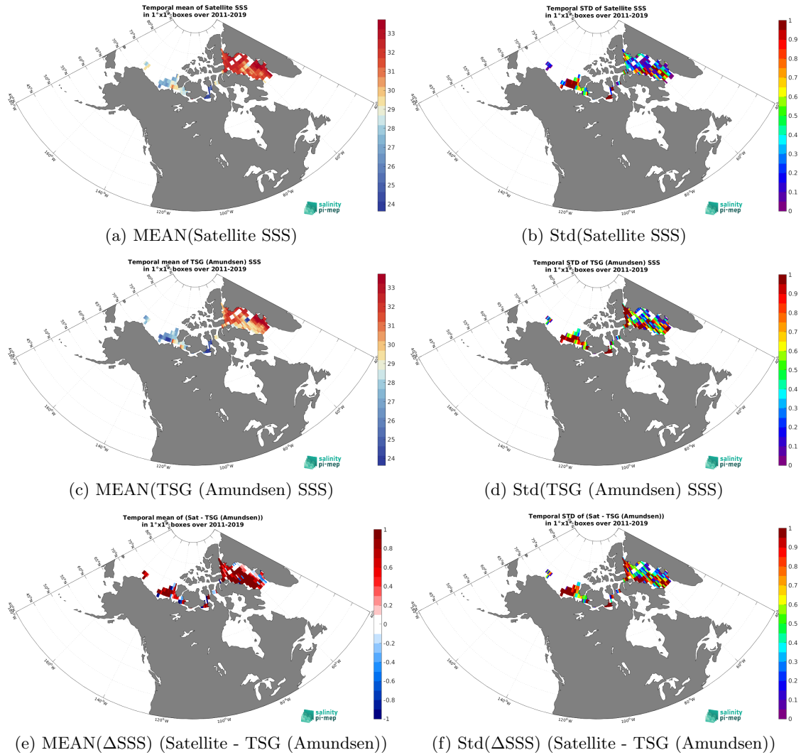
Figure 6: Temporal mean (left) and Std (right) of SSS from SMOS SSS L4 v2 - Daily (BEC) (top), TSG (Amundsen) (middle), and of \Delta SSS (Satellite - TSG (Amundsen)). Only match-up pairs are used to generate these maps.
