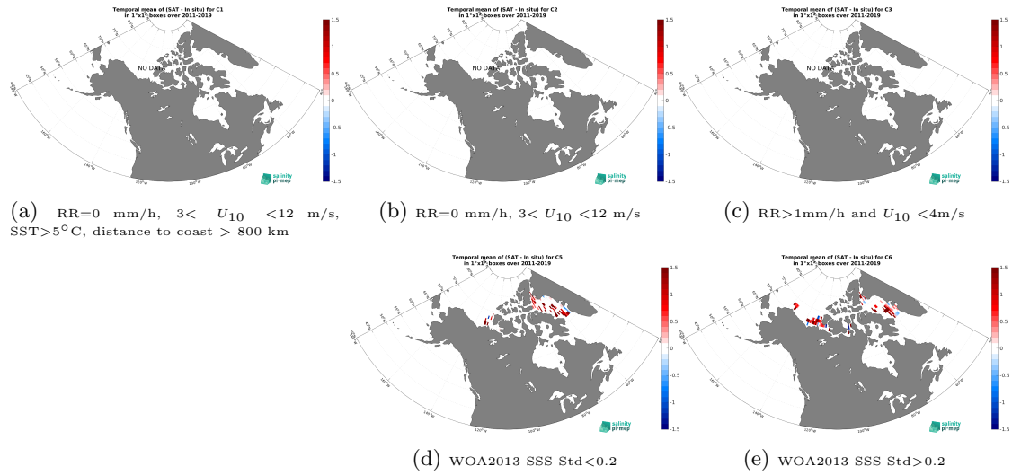
Figure 12: Temporal mean gridded over spatial boxes of size 1^{\circ}\times 1^{\circ} of \Delta\text{SSS} (SMOS SSS L4 v2 - Daily (BEC) - TSG (Amundsen)) for 5 different subdatasets corresponding to:RR=0 mm/h, 3 < U_{10} < 12 m/s, SST > 5^{\circ}\text{C} , distance to coast > 800 km (a), RR=0 mm/h, 3 < U_{10} < 12 m/s (b), RR > 1 mm/h and U_{10} < 4 m/s (c), WOA2013 SSS Std < 0.2 (d), WOA2013 SSS Std > 0.2 (e).
