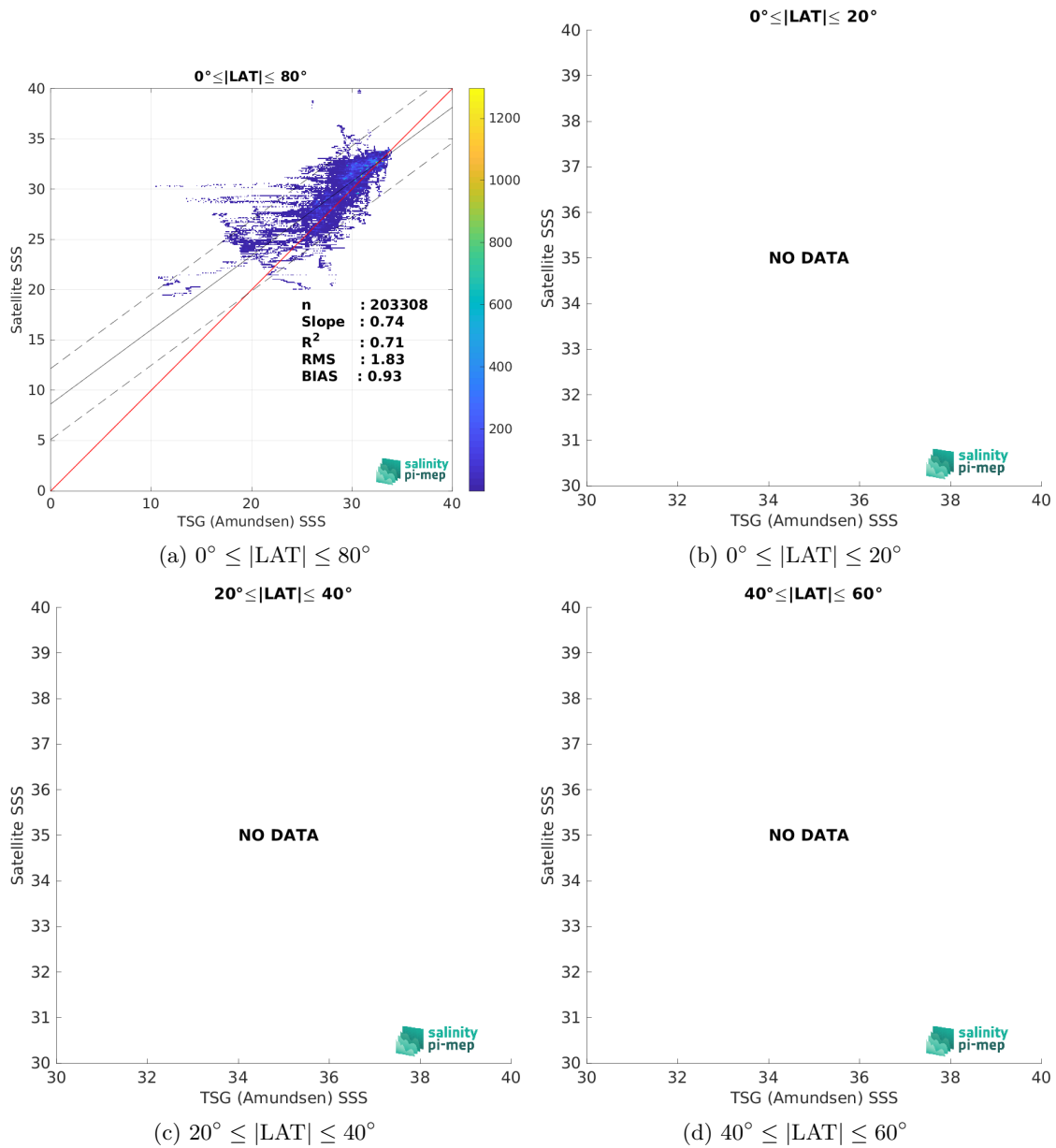
Figure 9: Contour maps of the concentration of SMOS SSS L4 v2 - Daily (BEC) SSS (y-axis) versus TSG (Amundsen) SSS (x-axis) at match-up pairs for different latitude bands. For each plot, the red line shows x=y . The black thin and dashed lines indicate a linear fit through the data cloud and the \pm 95\% confidence levels, respectively. The number match-up pairs n , the slope and R^2 coefficient of the linear fit, the root mean square (RMS) and the mean bias between satellite and in situ data are indicated for each latitude band in each plots.
