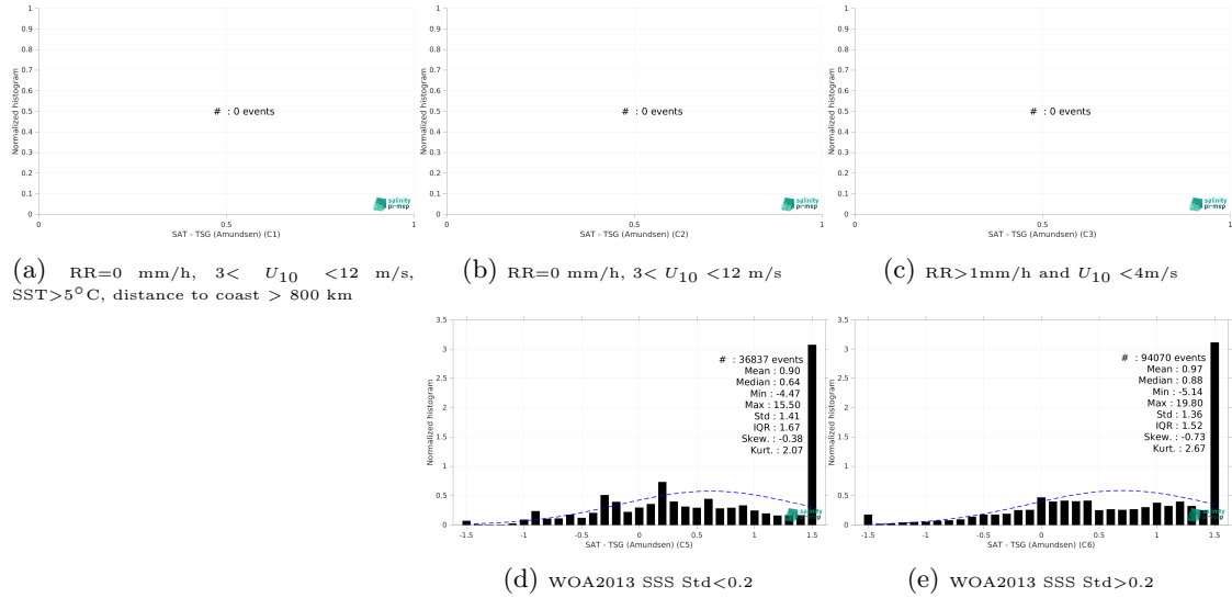
Figure 13: Normalized histogram of \Delta SSS (SMOS SSS L4 v2 - Daily (BEC) - TSG (Amundsen)) for 5 different subdatasets corresponding to: RR=0 mm/h, 3 < U_{10} < 12 m/s, SST > 5°C, distance to coast > 800 km (a), RR=0 mm/h, 3 < U_{10} < 12 m/s (b), RR > 1mm/h and U_{10} < 4 m/s (c), WOA2013 SSS Std < 0.2 (d), WOA2013 SSS Std > 0.2 (e).
