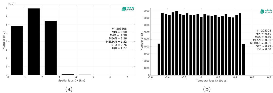
Figure 5: Histograms of the spatial (a) and temporal (b) lags between the location/time of the TSG (Amundsen) measurement and the date of the corresponding SMOS SSS L4 v2 - Daily (BEC) SSS pixel.
