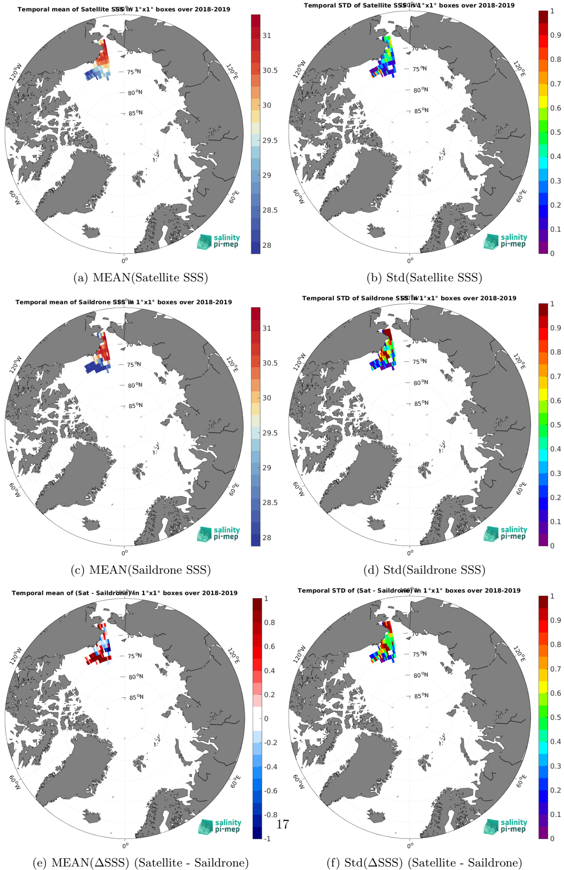
Figure 7: Temporal mean (left) and Std (right) of SSS from SMOS SSS L4 v2 - Daily (BEC) (top), Saildrone (middle), and of \Delta SSS (Satellite - Saildrone). Only match-up pairs are used to generate these maps.
