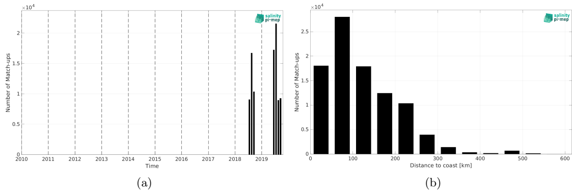
Figure 2: Number of match-ups between Saildrone and SMOS SSS L4 v2 - Daily (BEC) SSS as a function of time (a) and as function of the distance to coast (b) over the Arctic Ocean Pi-MEP region and for the full satellite product period.
