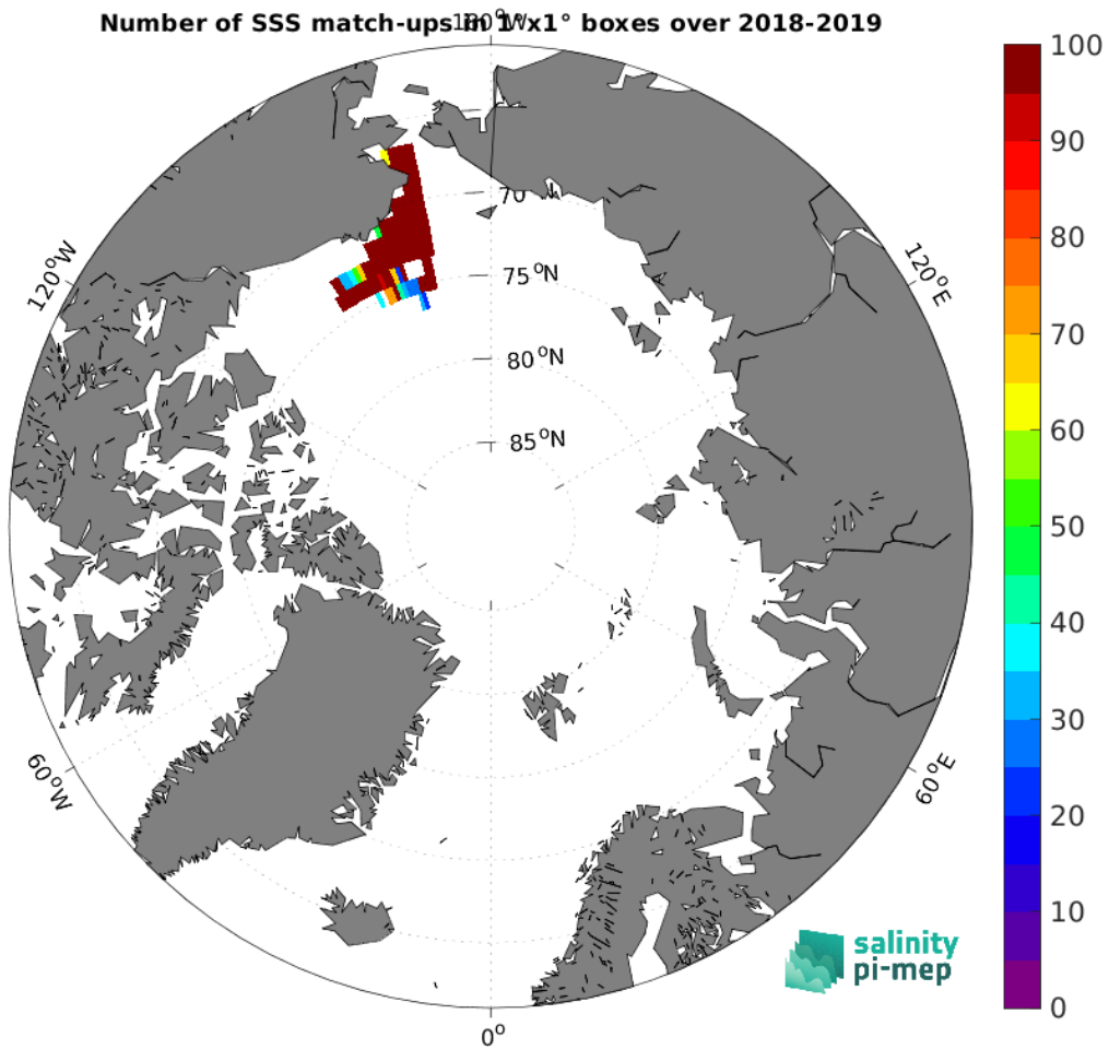
Figure 5: Number of SSS match-ups between Saildrone SSS and the SMOS SSS L4 v2 - Daily (BEC) SSS product for the Arctic Ocean Pi-MEP region over 1^\circ \times 1^\circ boxes and for the full satellite product period.
