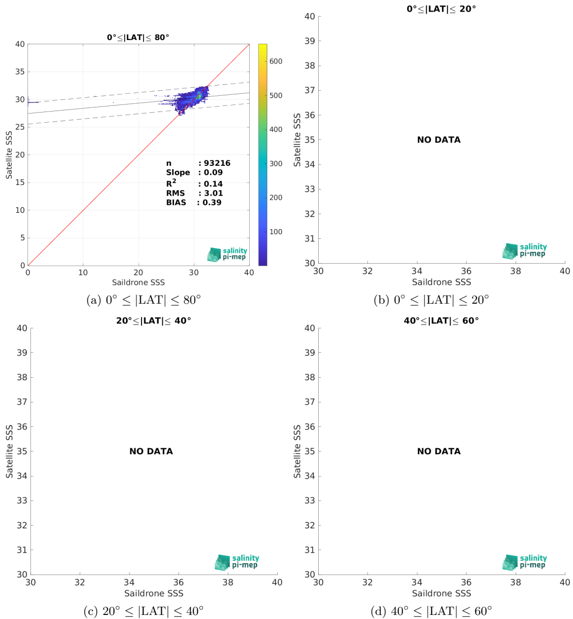
Figure 10: Contour maps of the concentration of SMOS SSS L4 v2 - Daily (BEC) SSS (y-axis) versus Saildrone SSS (x-axis) at match-up pairs for different latitude bands. For each plot, the red line shows x=y . The black thin and dashed lines indicate a linear fit through the data cloud and the \pm 95\% confidence levels, respectively. The number match-up pairs n , the slope and R^2 coefficient of the linear fit, the root mean square (RMS) and the mean bias between satellite and in situ data are indicated for each latitude band in each plots.
