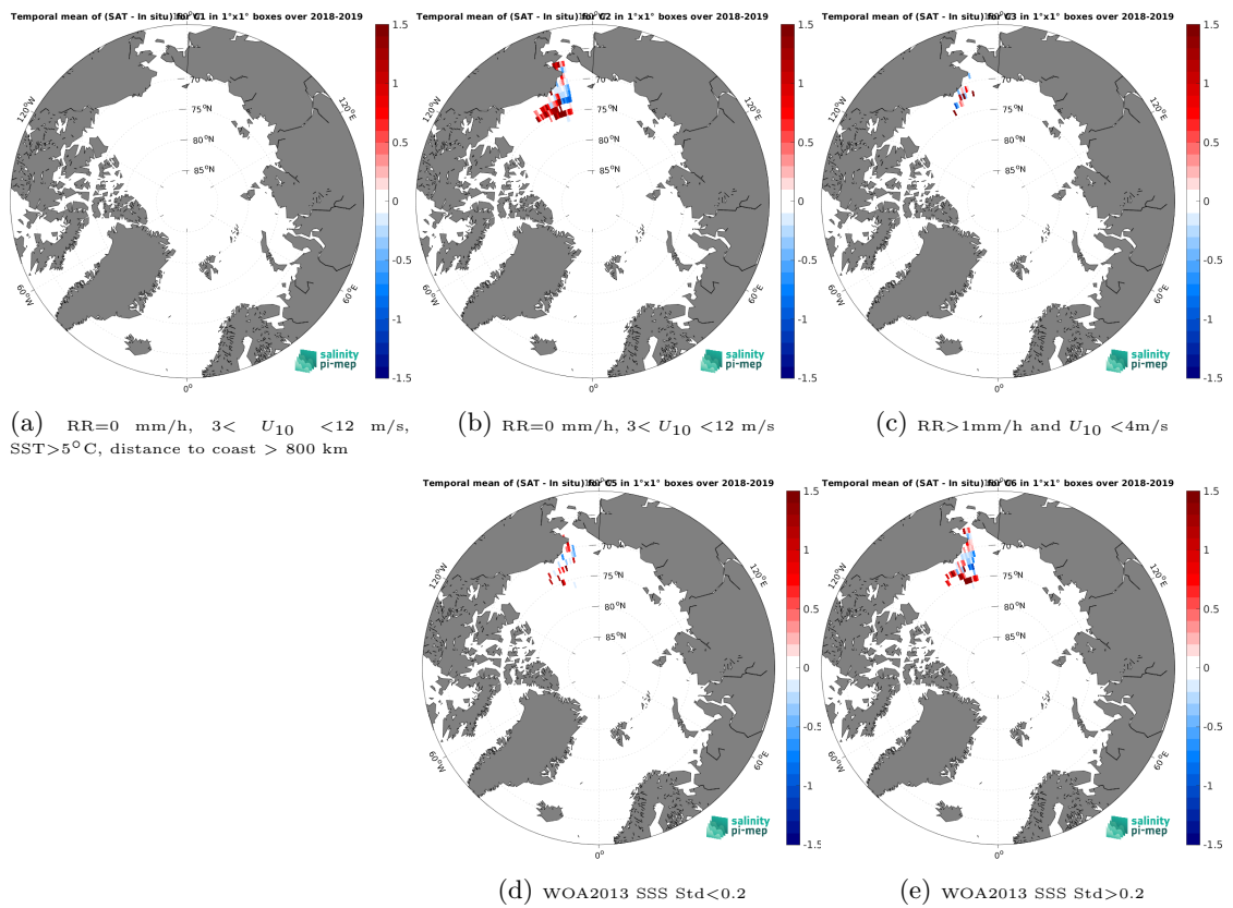
Figure 14: Temporal mean gridded over spatial boxes of size 1^\circ \times 1^\circ of \Delta SSS (SMOS SSS L4 v2 - Daily (BEC) - Saldrone) for 5 different subdatasets corresponding to:RR=0 mm/h, 3 < U_{10} < 12 m/s, SST>5°C, distance to coast > 800 km (a), RR=0 mm/h, 3 < U_{10} < 12 m/s (b), RR>1mm/h and U_{10} < 4 m/s (c), WOA2013 SSS Std<0.2 (d), WOA2013 SSS Std>0.2 (e).
