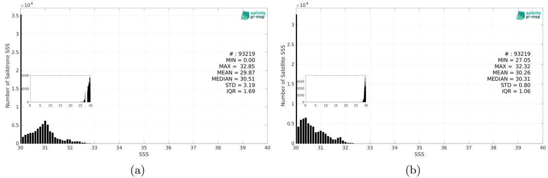
Figure 3: Histograms of SSS from Sairdrone (a) and SMOS SSS L4 v2 - Daily (BEC) (b) considering all match-up pairs per bins of 0.1 over the Arctic Ocean Pi-MEP region and for the full satellite product period.
