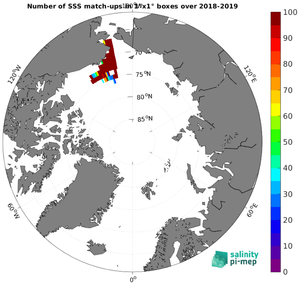
Figure 4: Number of SSS match-ups between Saildrone SSS and the SMOS SSS L4 v2 - Daily (BEC) SSS product for the Arctic Ocean Pi-MEP region over 1^\circ \times 1^\circ boxes and for the full satellite product period.
