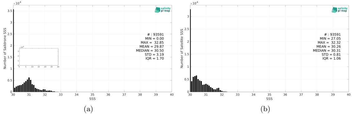
Figure 2: Histograms of SSS from Sairdrone (a) and SMOS SSS L4 v2 - Daily (BEC) (b) considering all match-up pairs per bins of 0.1 over the Arctic Ocean Pi-MEP region and for the full satellite product period.
