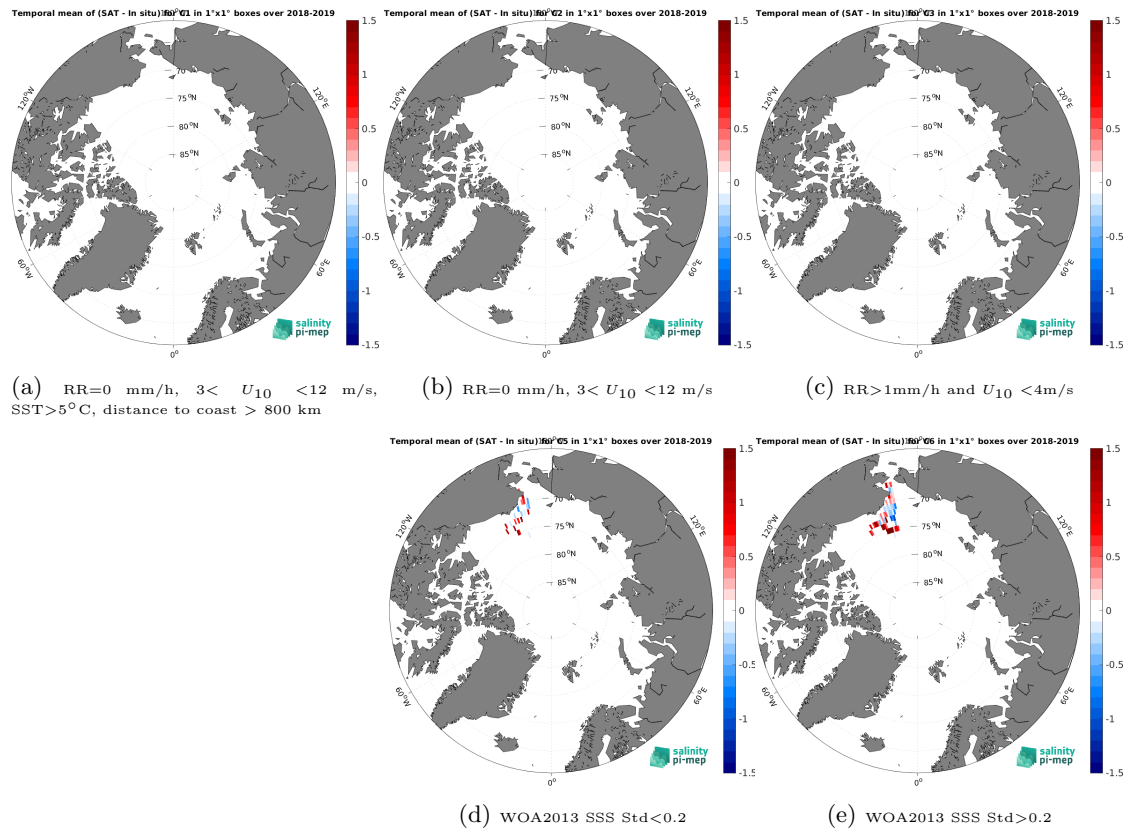
Figure 12: Temporal mean gridded over spatial boxes of size 1^{\circ}\times 1^{\circ} of \Delta\text{SSS} (SMOS SSS L4 v2 - Daily (BEC) - Sairdrone) for 5 different subdatasets corresponding to:RR=0 mm/h, 3 < U_{10} < 12 m/s, SST >5^{\circ}\text{C} , distance to coast > 800 km (a), RR=0 mm/h, 3 < U_{10} < 12 m/s (b), RR >1 mm/h and U_{10} < 4 m/s (c), WOA2013 SSS Std <0.2 (d), WOA2013 SSS Std >0.2 (e).
