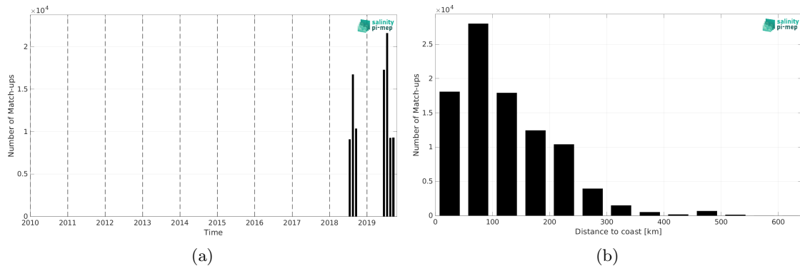
Figure 1: Number of match-ups between Saildrone and SMOS SSS L4 v2 - Daily (BEC) SSS as a function of time (a) and as function of the distance to coast (b) over the Arctic Ocean Pi-MEP region and for the full satellite product period.
