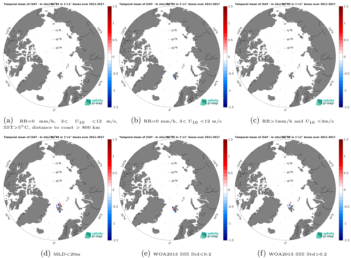
Figure 14: Temporal mean gridded over spatial boxes of size 1^\circ \times 1^\circ of \Delta SSS (SMOS SSS L4 v2 - Daily (BEC) - Marine mammals) for 6 different subdatasets corresponding to: RR=0 mm/h, 3 < U_{10} < 12 m/s, SST > 5°C, distance to coast > 800 km (a), RR=0 mm/h, 3 < U_{10} < 12 m/s (b), RR > 1mm/h and U_{10} < 4 m/s (c), MLD < 20m (d), WOA2013 SSS Std < 0.2 (e), WOA2013 SSS Std > 0.2 (f).
