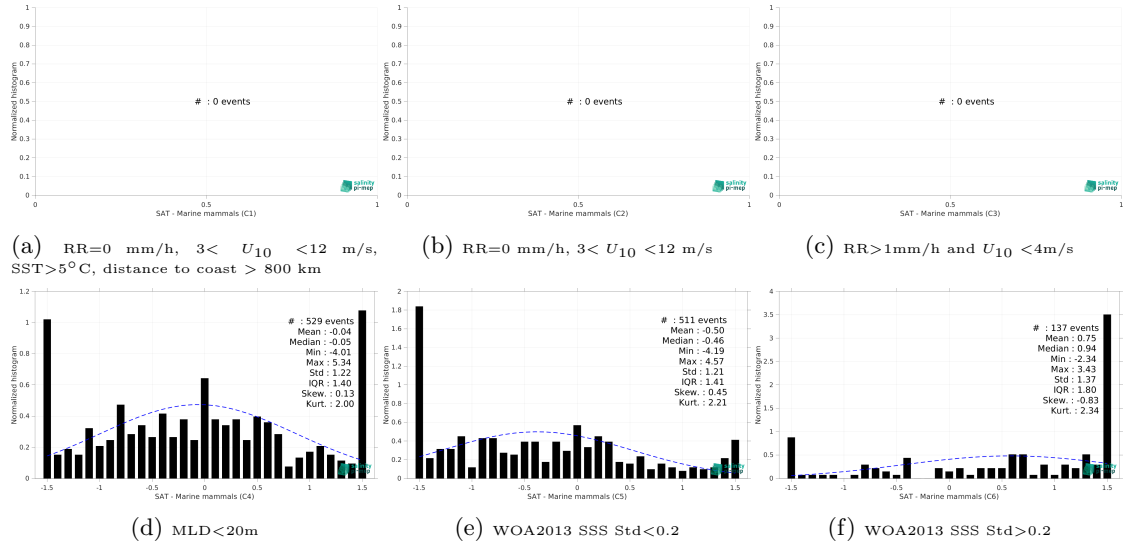
Figure 13: Normalized histogram of \Delta\text{SSS} (SMOS SSS L4 v2 - Daily (BEC) - Marine mammals) for 6 different subdatasets corresponding to: RR=0 mm/h, 3 < U_{10} < 12 m/s, SST > 5^{\circ}\text{C} , distance to coast > 800 km (a), RR=0 mm/h, 3 < U_{10} < 12 m/s (b), RR > 1\text{mm/h} and U_{10} < 4\text{m/s} (c), MLD < 20\text{m} (d), WOA2013 SSS Std < 0.2 (e), WOA2013 SSS Std > 0.2 (f).
