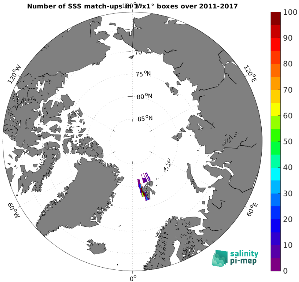
Figure 4: Number of SSS match-ups between Marine mammals SSS and the SMOS SSS L4 v2 - Daily (BEC) SSS product for the Arctic Ocean Pi-MEP region over 1^{\circ} \times 1^{\circ} boxes and for the full satellite product period.
