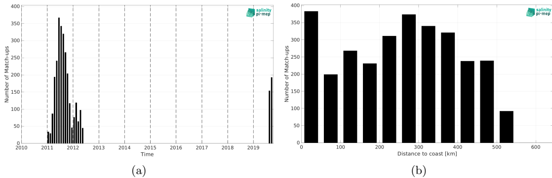
Figure 1: Number of match-ups between Surface drifters and SMOS SSS L4 v2 - Daily (BEC) SSS as a function of time (a) and as function of the distance to coast (b) over the Arctic Ocean Pi-MEP region and for the full satellite product period.
