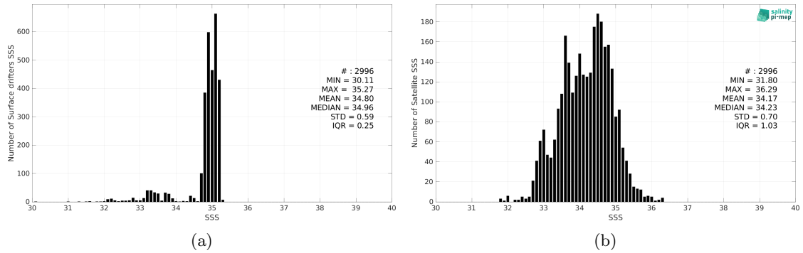
Figure 2: Histograms of SSS from Surface drifters (a) and SMOS SSS L4 v2 - Daily (BEC) (b) considering all match-up pairs per bins of 0.1 over the Arctic Ocean Pi-MEP region and for the full satellite product period.
