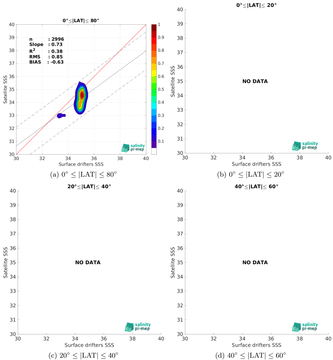
Figure 8: Contour maps of the concentration of SMOS SSS L4 v2 - Daily (BEC) SSS (y-axis) versus Surface drifters SSS (x-axis) at match-up pairs for different latitude bands. For each plot, the red line shows x=y . The black thin and dashed lines indicate a linear fit through the data cloud and the \pm 95\% confidence levels, respectively. The number match-up pairs n , the slope and R^2 coefficient of the linear fit, the root mean square (RMS) and the mean bias between satellite and in situ data are indicated for each latitude band in each plots.
