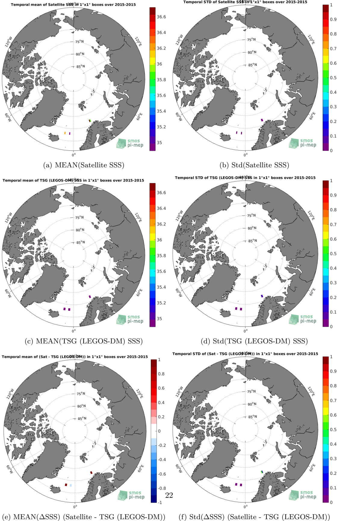
Figure 6: Temporal mean (left) and Std (right) of SSS from SMOS SSS L3 v3 Monthly (ICDC) (top), TSG (LEGOS-DM) (middle), and of \Delta SSS (Satellite - TSG (LEGOS-DM)). Only match-up pairs are used to generate these maps.
