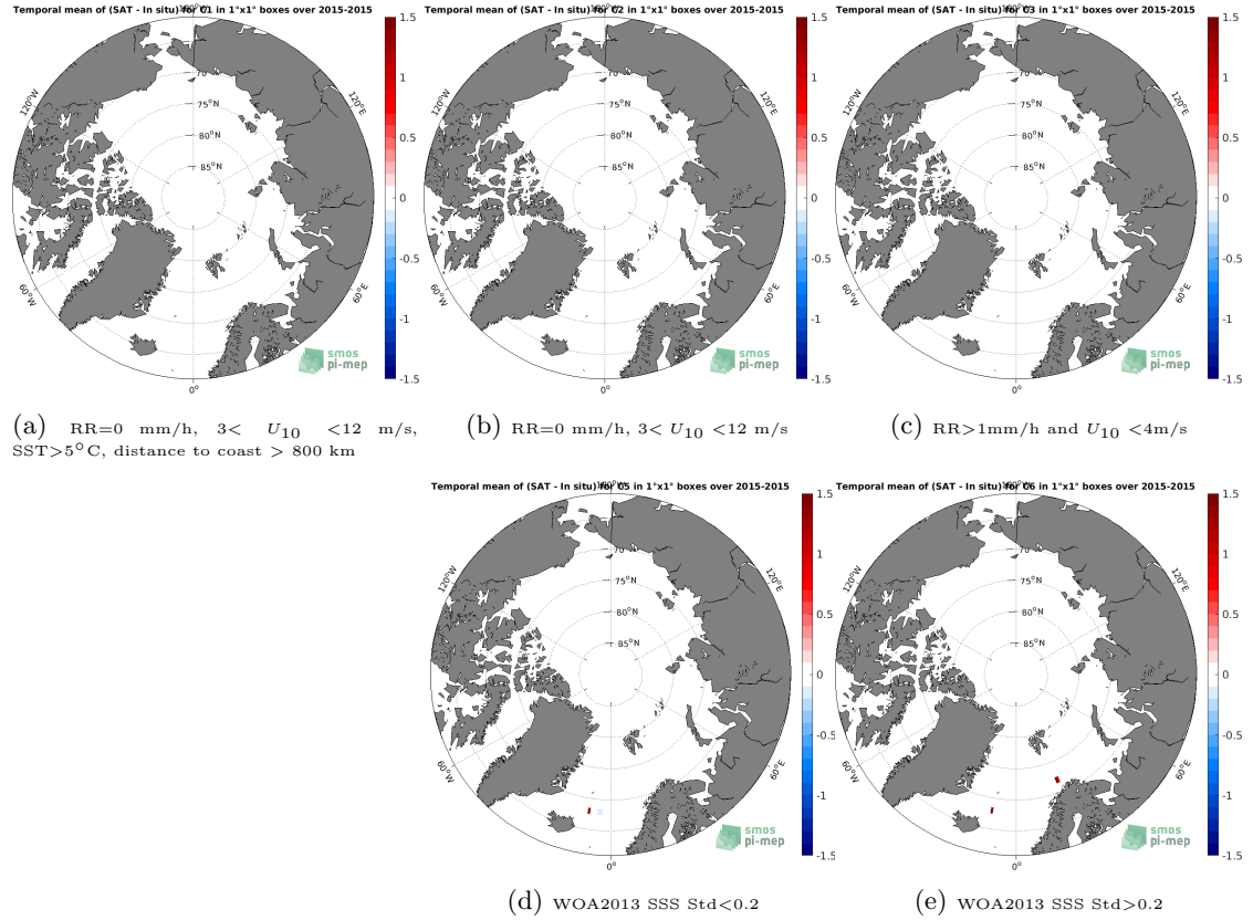
Figure 12: Temporal mean gridded over spatial boxes of size 1^{\circ}\times 1^{\circ} of \Delta\text{SSS} (SMOS SSS L3 v3 Monthly (ICDC) - TSG (LEGOS-DM)) for 5 different subdatasets corresponding to: RR=0 mm/h, 3 < U_{10} < 12 m/s, SST >5^{\circ}\text{C} , distance to coast > 800 km (a), RR=0 mm/h, 3 < U_{10} < 12 m/s (b), RR >1 mm/h and U_{10} < 4 m/s (c), WOA2013 SSS Std <0.2 (d), WOA2013 SSS Std >0.2 (e).
