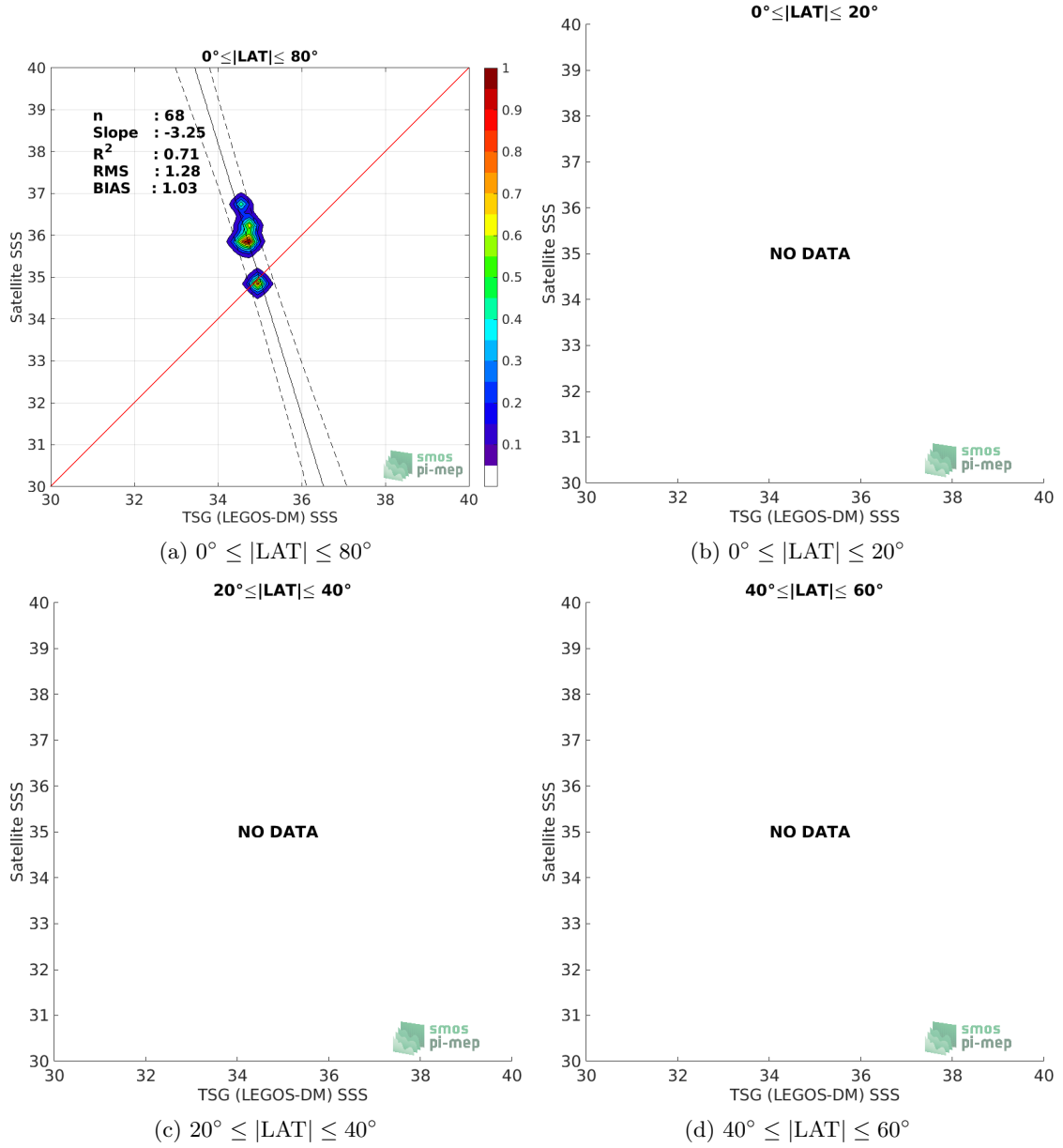
Figure 9: Contour maps of the concentration of SMOS SSS L3 v3 Monthly (ICDC) SSS (y-axis) versus TSG (LEGOS-DM) SSS (x-axis) at match-up pairs for different latitude bands. For each plot, the red line shows x=y . The black thin and dashed lines indicate a linear fit through the data cloud and the \pm 95\% confidence levels, respectively. The number match-up pairs n , the slope and R^2 coefficient of the linear fit, the root mean square (RMS) and the mean bias between satellite and in situ data are indicated for each latitude band in each plots.
