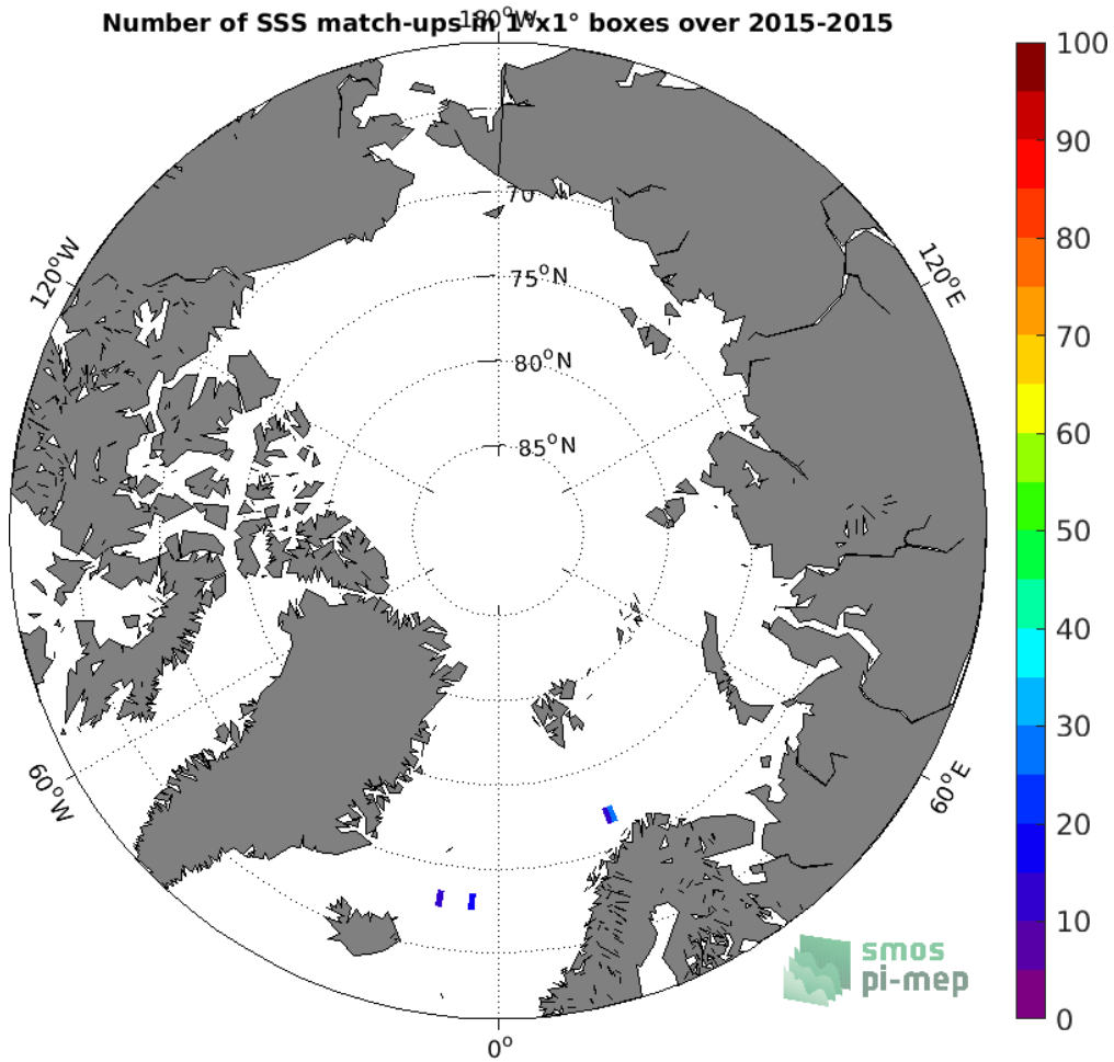
Figure 4: Number of SSS match-ups between TSG (LEGOS-DM) SSS and the SMOS SSS L3 v3 Monthly (ICDC) SSS product for the Arctic Ocean Pi-MEP region over 1^\circ \times 1^\circ boxes and for the full satellite product period.
