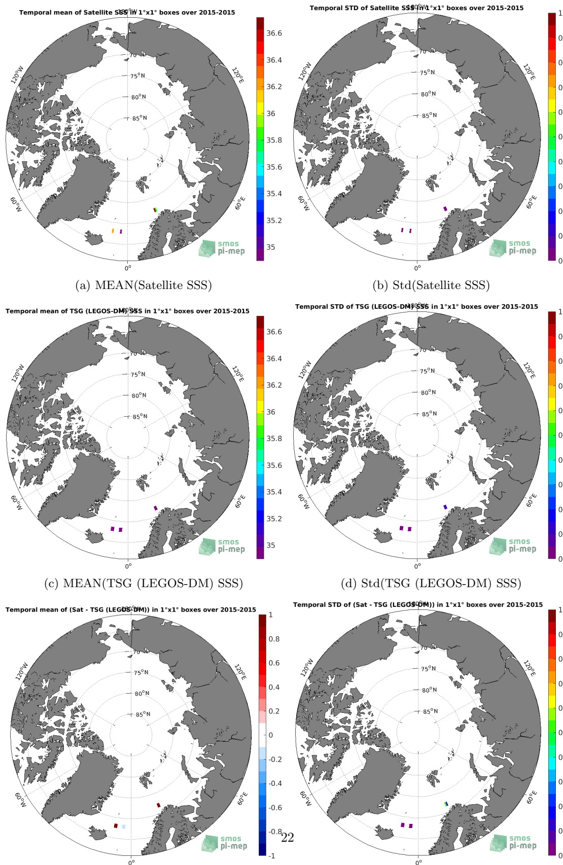
(e) MEAN( \Delta SSS) (Satellite - TSG (LEGOS-DM)) (f) Std( \Delta SSS) (Satellite - TSG (LEGOS-DM)) Figure 6: Temporal mean (left) and Std (right) of SSS from SMOS SSS L3 v3 Monthly (ICDC) (top), TSG (LEGOS-DM) (middle), and of \Delta SSS (Satellite - TSG (LEGOS-DM)). Only match-up pairs are used to generate these maps.
