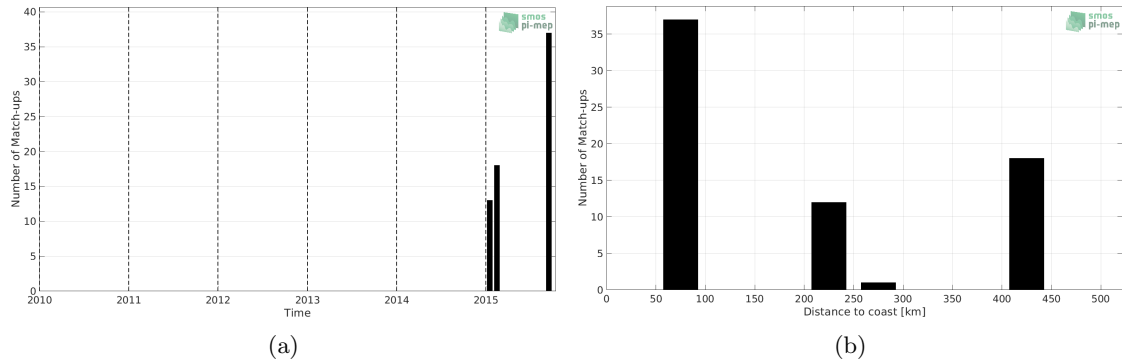
Figure 1: Number of match-ups between TSG (LEGOS-DM) and SMOS SSS L3 v3 Monthly (ICDC) SSS as a function of time (a) and as function of the distance to coast (b) over the Arctic Ocean Pi-MEP region and for the full satellite product period.
