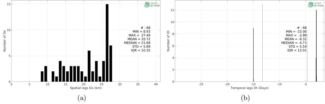
Figure 5: Histograms of the spatial (a) and temporal (b) lags between the location/time of the TSG (LEGOS-DM) measurement and the date of the corresponding SMOS SSS L3 v3 Monthly (ICDC) SSS pixel.
