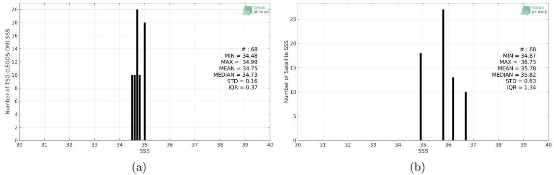
Figure 2: Histograms of SSS from TSG (LEGOS-DM) (a) and SMOS SSS L3 v3 Monthly (ICDC) (b) considering all match-up pairs per bins of 0.1 over the Arctic Ocean Pi-MEP region and for the full satellite product period.
