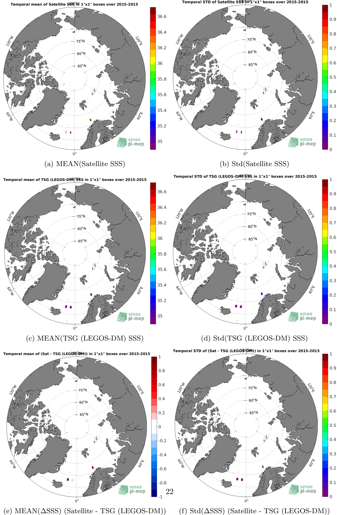
Figure 6: Temporal mean (left) and Std (right) of SSS from SMOS SSS L3 v3 Monthly (ICDC) (top), TSG (LEGOS-DM) (middle), and of \Delta SSS (Satellite - TSG (LEGOS-DM)). Only match-up pairs are used to generate these maps.
