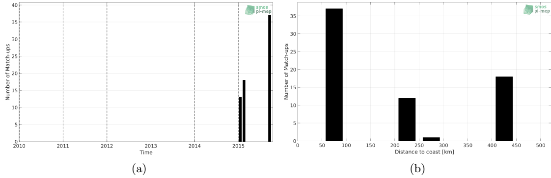
Figure 1: Number of match-ups between TSG-LEGOS-DM and SMOS-L3-ICDC-V3-MONTHLY-0.5DEG SSS as a function of time (a) and as function of the distance to coast (b) over the Arctic Ocean Pi-MEP region and for the full satellite product period.
