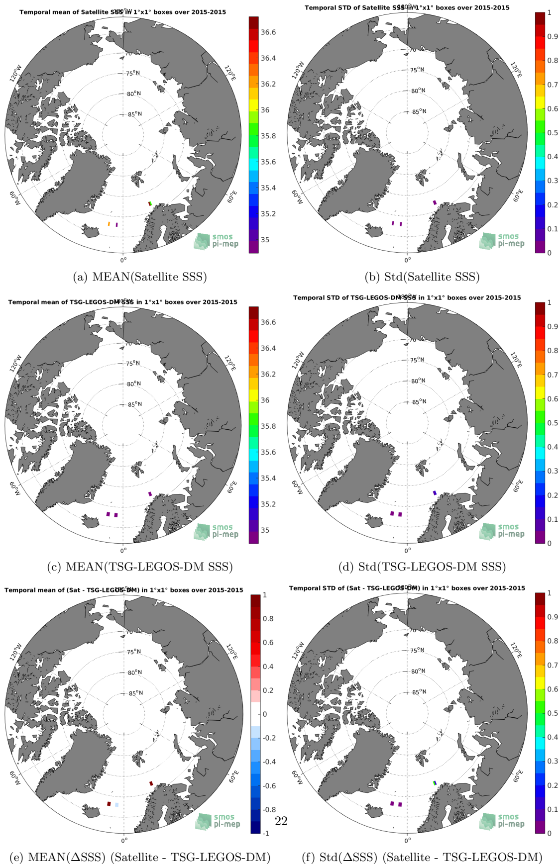
Figure 6: Temporal mean (left) and Std (right) of SSS from SMOS-L3-ICDC-V3-MONTHLY-0.5DEG (top), TSG-LEGOS-DM (middle), and of \Delta SSS (Satellite - TSG-LEGOS-DM). Only match-up pairs are used to generate these maps.
