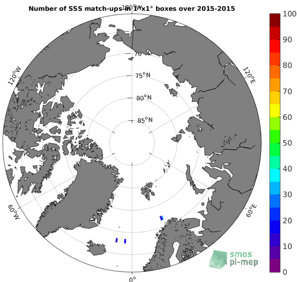
Figure 4: Number of SSS match-ups between TSG-LEGOS-DM SSS and the SMOS-L3-ICDC-V3-MONTHLY-0.5DEG SSS product for the Arctic Ocean Pi-MEP region over 1°x1° boxes and for the full satellite product period.
