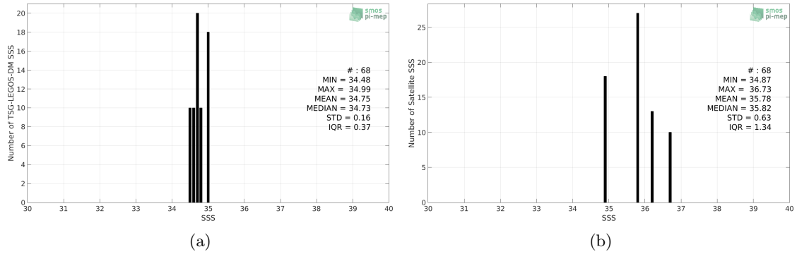
Figure 2: Histograms of SSS from TSG-LEGOS-DM (a) and SMOS-L3-ICDC-V3-MONTHLY-0.5DEG (b) considering all match-up pairs per bins of 0.1 over the Arctic Ocean Pi-MEP region and for the full satellite product period.
