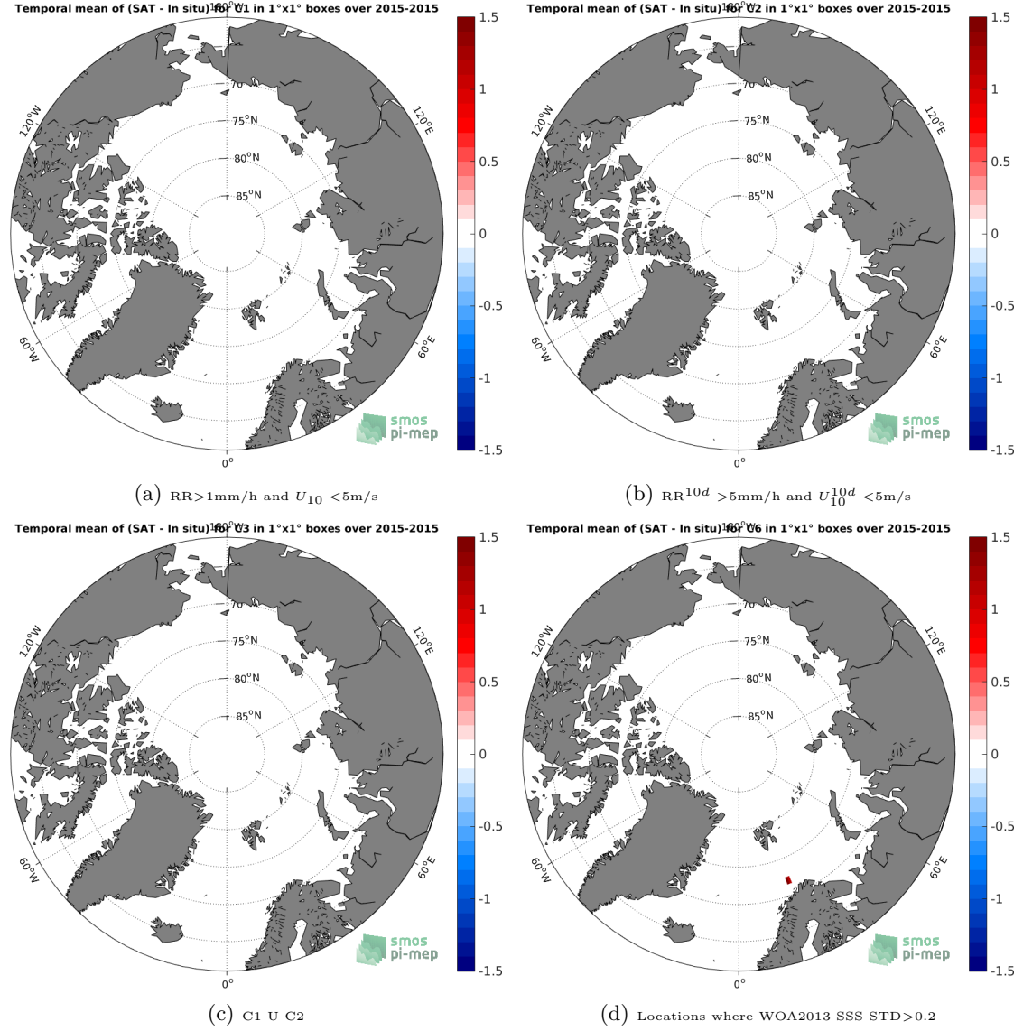
Figure 12: Temporal mean gridded over spatial boxes of size 1^\circ \times 1^\circ of \Delta SSS (SMOS-L3-ICDC-V3-MONTHLY-0.5DEG - TSG-LEGOS-DM) for 4 different subdatasets corresponding to: RR > 1\text{mm/h} and U_{10} < 5\text{m/s} (a), RR^{10d} > 5\text{mm/h} and U_{10}^{10d} < 5\text{m/s} (b), C1 U C2 (c), Locations where WOA2013 SSS STD > 0.2 (d).
