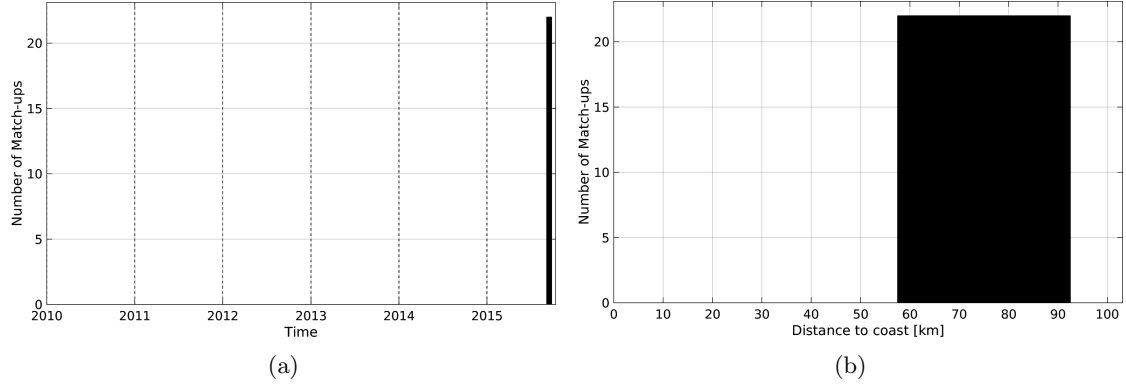
Figure 1: Number of match-ups between TSG-LEGOS-DM and SMOS-L3-ICDC-V3-MONTHLY-0.5DEG SSS as a function of time (a) and as function of the distance to coast (b) over the Arctic Ocean Pi-MEP region and for the full satellite product period.
