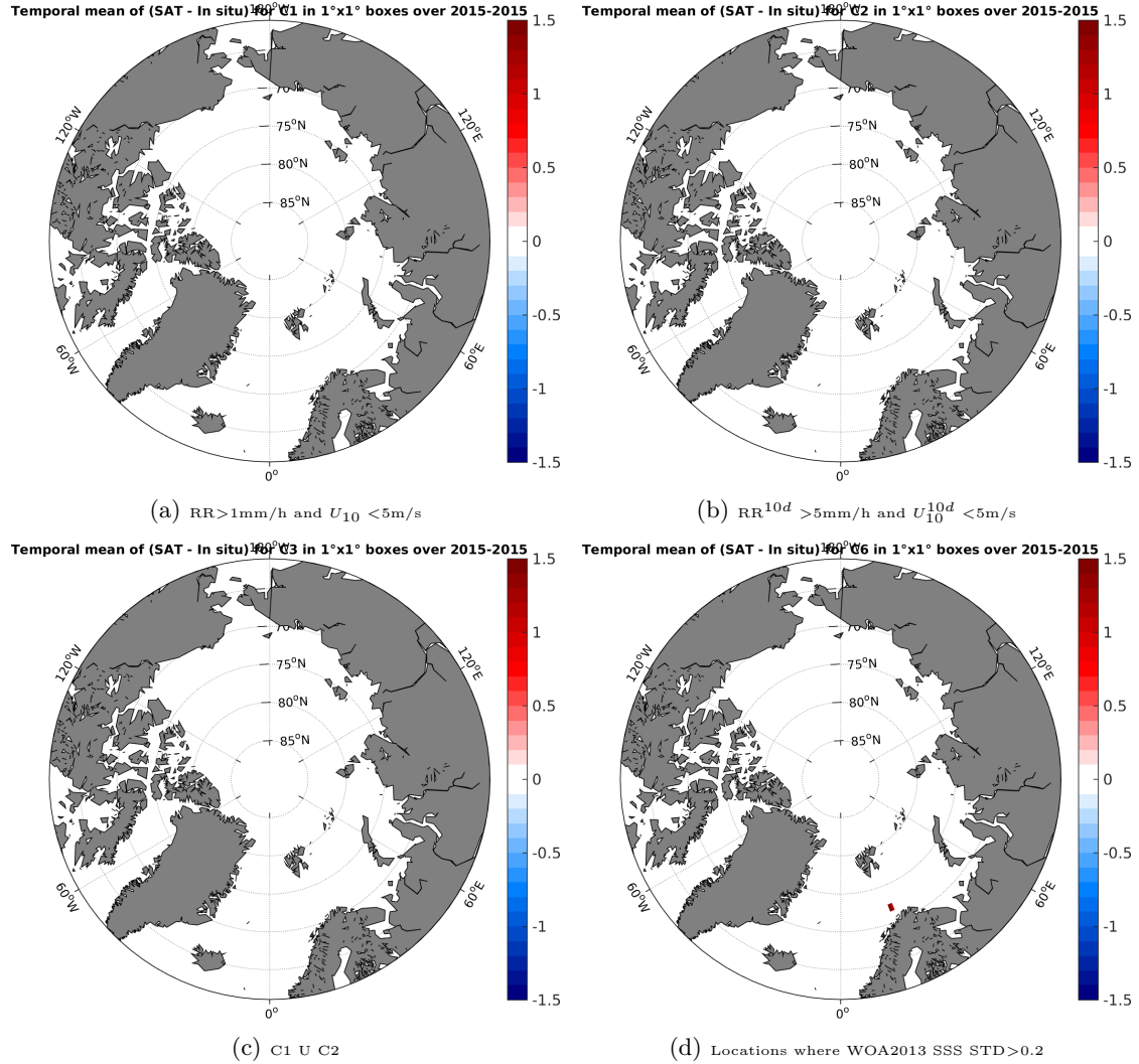
Figure 12: Temporal mean gridded over spatial boxes of size 1^\circ \times 1^\circ of \Delta SSS (SMOS-L3-ICDC-V3-MONTHLY-0.5DEG - TSG-LEGOS-DM) for 4 different subdatasets corresponding to: RR > 1\text{mm/h} and U_{10} < 5\text{m/s} (a), RR^{10d} > 5\text{mm/h} and U_{10}^{10d} < 5\text{m/s} (b), C1 U C2 (c), Locations where WOA2013 SSS STD > 0.2 (d).
