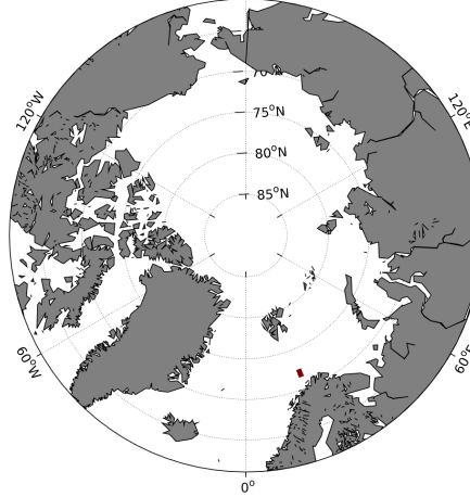
(e) MEAN( \Delta SSS) (Satellite - TSG-LEGOS-DM)
