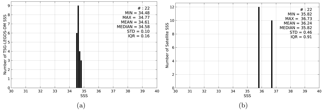
Figure 2: Histograms of SSS from TSG-LEGOS-DM (a) and SMOS-L3-ICDC-V3-MONTHLY-0.5DEG (b) considering all match-up pairs per bins of 0.1 over the Arctic Ocean Pi-MEP region and for the full satellite product period.
