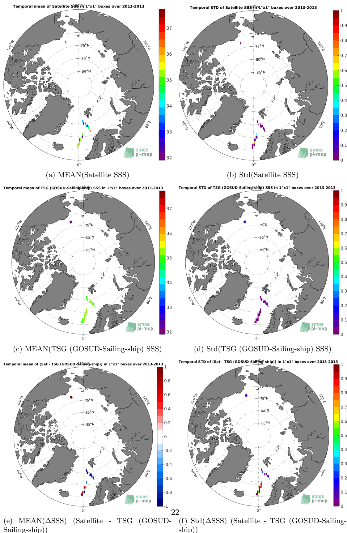
Figure 6: Temporal mean (left) and Std (right) of SSS from SMOS SSS L3 v3 Monthly (ICDC) (top), TSG (GOSUD-Sailing-ship) (middle), and of \Delta SSS (Satellite - TSG (GOSUD-Sailing-ship)). Only match-up pairs are used to generate these maps.
