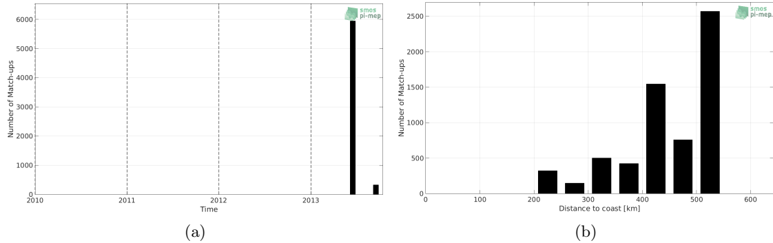
Figure 1: Number of match-ups between TSG (GOSUD-Sailing-ship) and SMOS SSS L3 v3 Monthly (ICDC) SSS as a function of time (a) and as function of the distance to coast (b) over the Arctic Ocean Pi-MEP region and for the full satellite product period.
