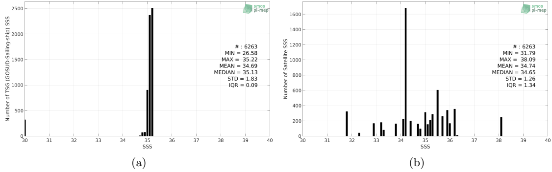
Figure 2: Histograms of SSS from TSG (GOSUD-Sailing-ship) (a) and SMOS SSS L3 v3 Monthly (ICDC) (b) considering all match-up pairs per bins of 0.1 over the Arctic Ocean Pi-MEP region and for the full satellite product period.
