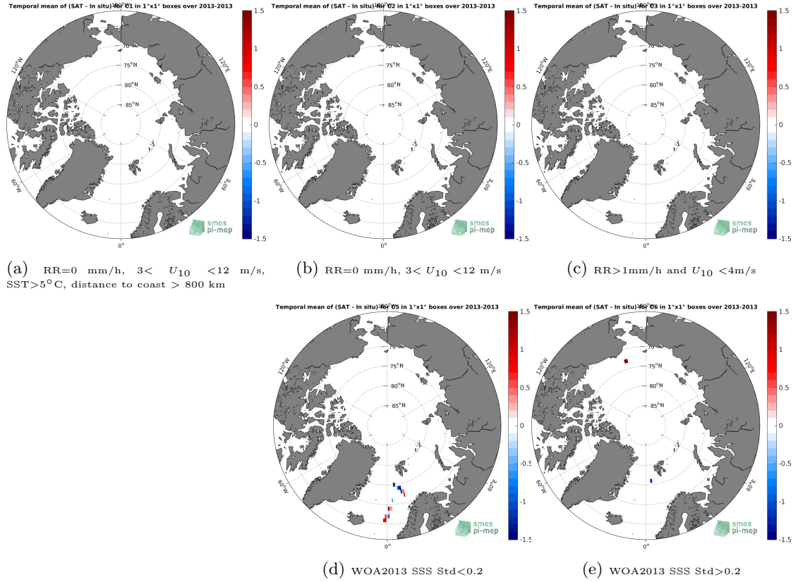
Figure 12: Temporal mean gridded over spatial boxes of size 1^\circ \times 1^\circ of \Delta\text{SSS} (SMOS SSS L3 v3 Monthly (ICDC) - TSG (GOSUD-Sailing-ship)) for 5 different subdatasets corresponding to: RR=0 mm/h, 3 < U_{10} < 12 m/s, SST > 5^\circ\text{C} , distance to coast > 800 km (a), RR=0 mm/h, 3 < U_{10} < 12 m/s (b), RR > 1 mm/h and U_{10} < 4 m/s (c), WOA2013 SSS Std < 0.2 (d), WOA2013 SSS Std > 0.2 (e).
