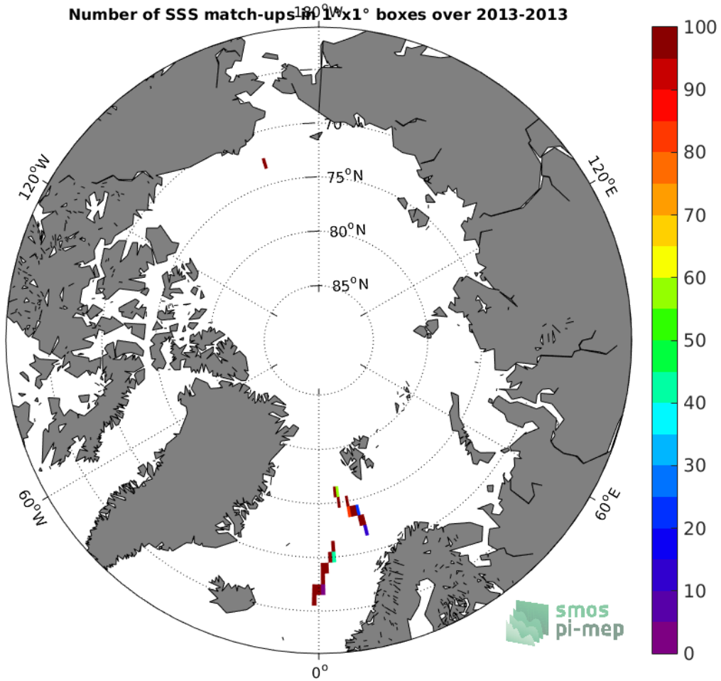
Figure 4: Number of SSS match-ups between TSG (GOSUD-Sailing-ship) SSS and the SMOS SSS L3 v3 Monthly (ICDC) SSS product for the Arctic Ocean Pi-MEP region over 1^\circ \times 1^\circ boxes and for the full satellite product period.
