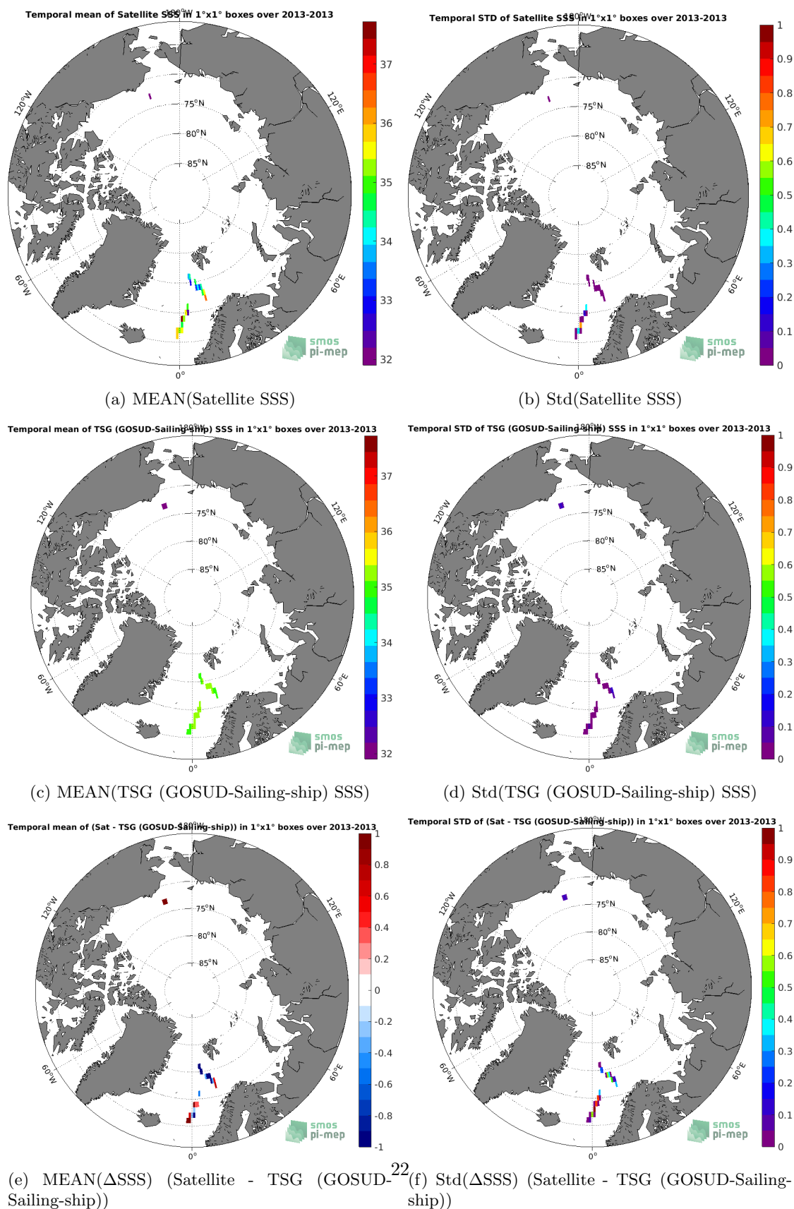
Figure 6: Temporal mean (left) and Std (right) of SSS from SMOS SSS L3 v3 Monthly (ICDC) (top), TSG (GOSUD-Sailing-ship) (middle), and of \Delta SSS (Satellite - TSG (GOSUD-Sailing-ship)). Only match-up pairs are used to generate these maps.
