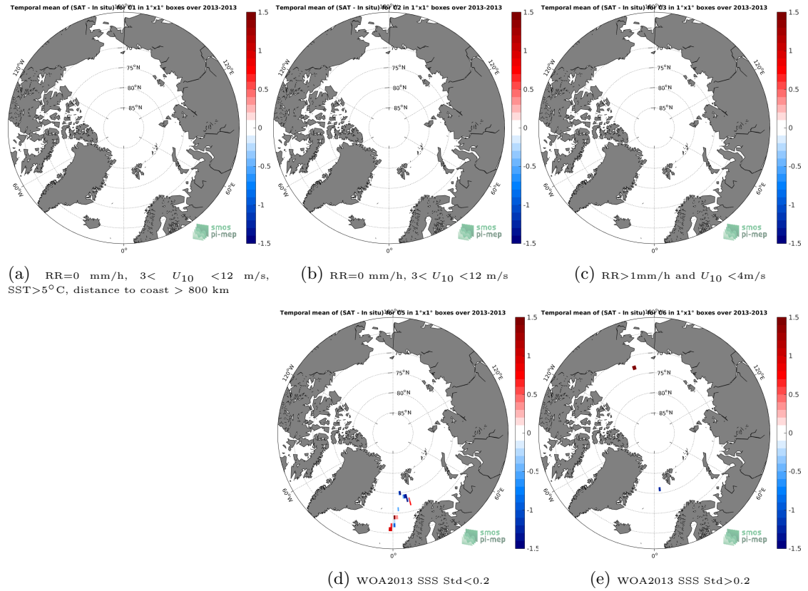
Figure 12: Temporal mean gridded over spatial boxes of size 1^{\circ} \times 1^{\circ} of \Delta\text{SSS} (SMOS-L3-ICDC-V3-MONTHLY-0.5DEG - TSG-GOSUD-Sailing-ship) for 5 different subdatasets corresponding to: RR=0 mm/h, 3 < U_{10} < 12 m/s, SST > 5^{\circ}\text{C} , distance to coast > 800 km (a), RR=0 mm/h, 3 < U_{10} < 12 m/s (b), RR > 1\text{mm/h} and U_{10} < 4\text{m/s} (c), WOA2013 SSS Std < 0.2 (d), WOA2013 SSS Std > 0.2 (e).
