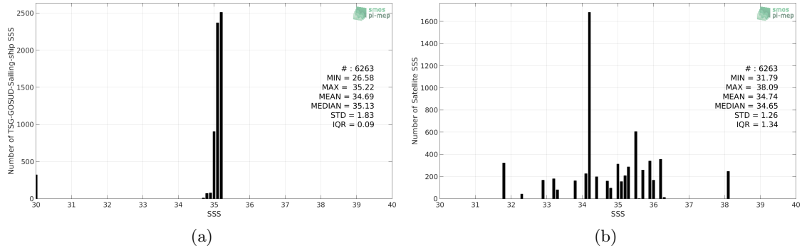
Figure 2: Histograms of SSS from TSG-GOSUD-Sailing-ship (a) and SMOS-L3-ICDC-V3-MONTHLY-0.5DEG (b) considering all match-up pairs per bins of 0.1 over the Arctic Ocean Pi-MEP region and for the full satellite product period.
