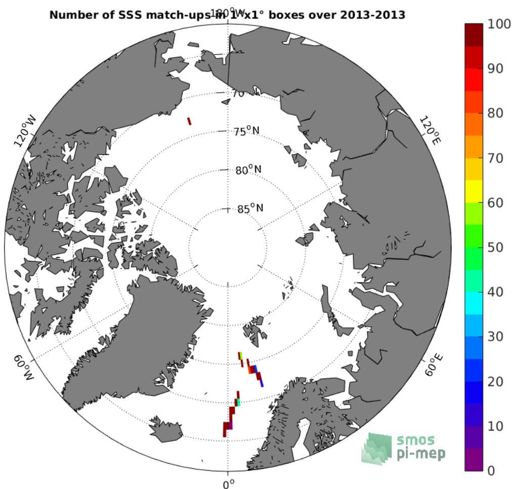
Figure 4: Number of SSS match-ups between TSG-GOSUD-Sailing-ship SSS and the SMOS-L3-ICDC-V3-MONTHLY-0.5DEG SSS product for the Arctic Ocean Pi-MEP region over 1^\circ \times 1^\circ boxes and for the full satellite product period.
