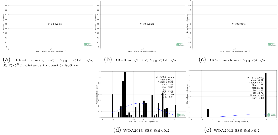
Figure 13: Normalized histogram of \Delta\text{SSS} (SMOS-L3-ICDC-V3-MONTHLY-0.5DEG - TSG-GOSUD-Sailing-ship) for 5 different subdatasets corresponding to: RR=0 mm/h, 3 < U_{10} < 12 m/s, SST > 5^\circ\text{C} , distance to coast > 800 km (a), RR=0 mm/h, 3 < U_{10} < 12 m/s (b), RR > 1\text{mm/h} and U_{10} < 4\text{m/s} (c), WOA2013 SSS Std<0.2 (d), WOA2013 SSS Std>0.2 (e).
