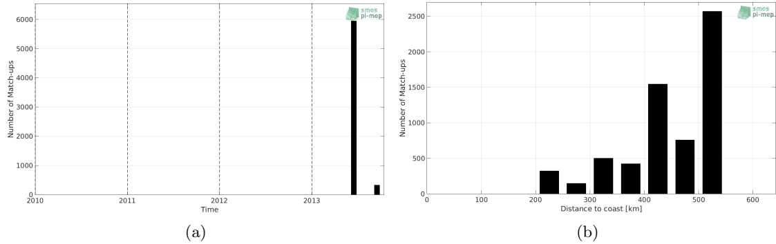
Figure 1: Number of match-ups between TSG-GOSUD-Sailing-ship and SMOS-L3-ICDC-V3-MONTHLY-0.5DEG SSS as a function of time (a) and as function of the distance to coast (b) over the Arctic Ocean Pi-MEP region and for the full satellite product period.
