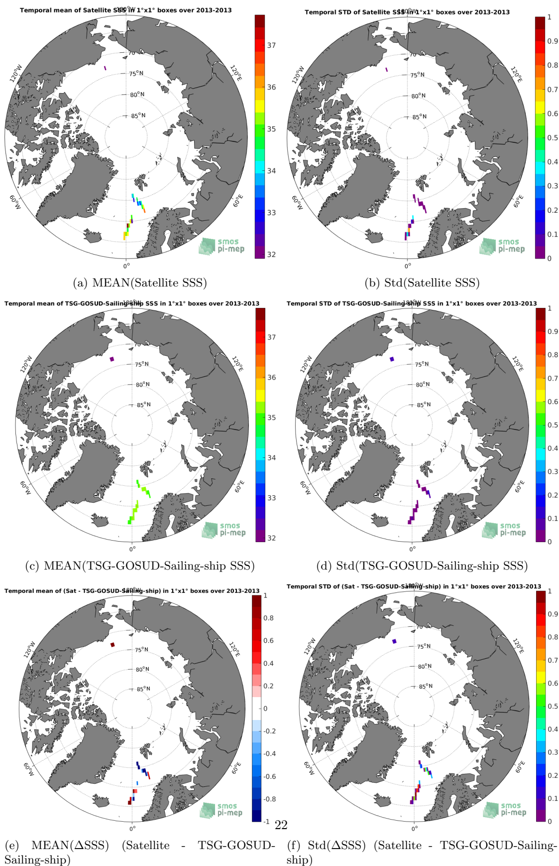
Figure 6: Temporal mean (left) and Std (right) of SSS from SMOS-L3-ICDC-V3-MONTHLY-0.5DEG (top), TSG-GOSUD-Sailing-ship (middle), and of \Delta SSS (Satellite - TSG-GOSUD-Sailing-ship). Only match-up pairs are used to generate these maps.
