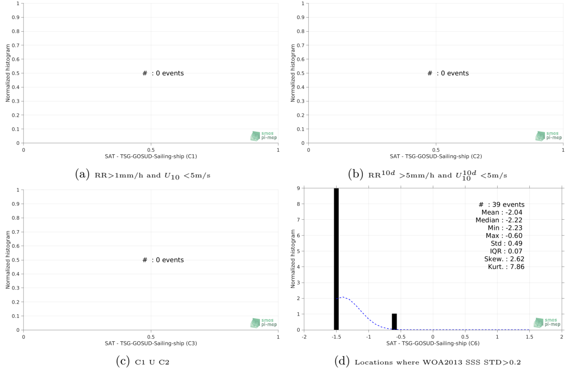
Figure 13: Normalized histogram of \Delta SSS (SMOS-L3-ICDC-V3-MONTHLY-0.5DEG - TSG-GOSUD-Sailing-ship) for 6 different subdatasets corresponding to: RR > 1\text{mm/h} and U_{10} < 5\text{m/s} (a), RR^{10d} > 5\text{mm/h} and U_{10}^{10d} < 5\text{m/s} (b), C1 U C2 (c), Locations where WOA2013 SSS STD > 0.2 (d).
