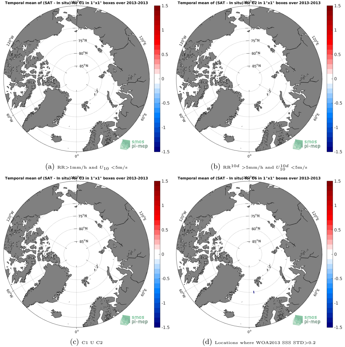
Figure 12: Temporal mean gridded over spatial boxes of size 1^\circ \times 1^\circ of \Delta SSS (SMOS-L3-ICDC-V3-MONTHLY-0.5DEG - TSG-GOSUD-Sailing-ship) for 4 different subdatasets corresponding to: RR > 1\text{mm/h} and U_{10} < 5\text{m/s} (a), RR^{10d} > 5\text{mm/h} and U_{10}^{10d} < 5\text{m/s} (b), C1 U C2 (c), Locations where WOA2013 SSS STD > 0.2 (d).
