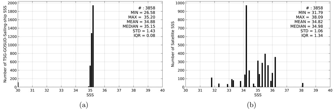
Figure 2: Histograms of SSS from TSG-GOSUD-Sailing-ship (a) and SMOS-L3-ICDC-V3-MONTHLY-0.5DEG (b) considering all match-up pairs per bins of 0.1 over the Arctic Ocean Pi-MEP region and for the full satellite product period.
