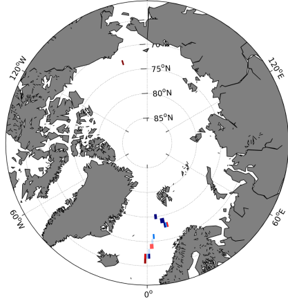
(e) MEAN( \Delta SSS) (Satellite - TSG-GOSUD-Sailing-ship)
