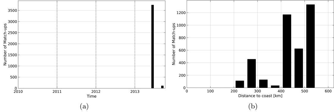
Figure 1: Number of match-ups between TSG-GOSUD-Sailing-ship and SMOS-L3-ICDC-V3-MONTHLY-0.5DEG SSS as a function of time (a) and as function of the distance to coast (b) over the Arctic Ocean Pi-MEP region and for the full satellite product period.
