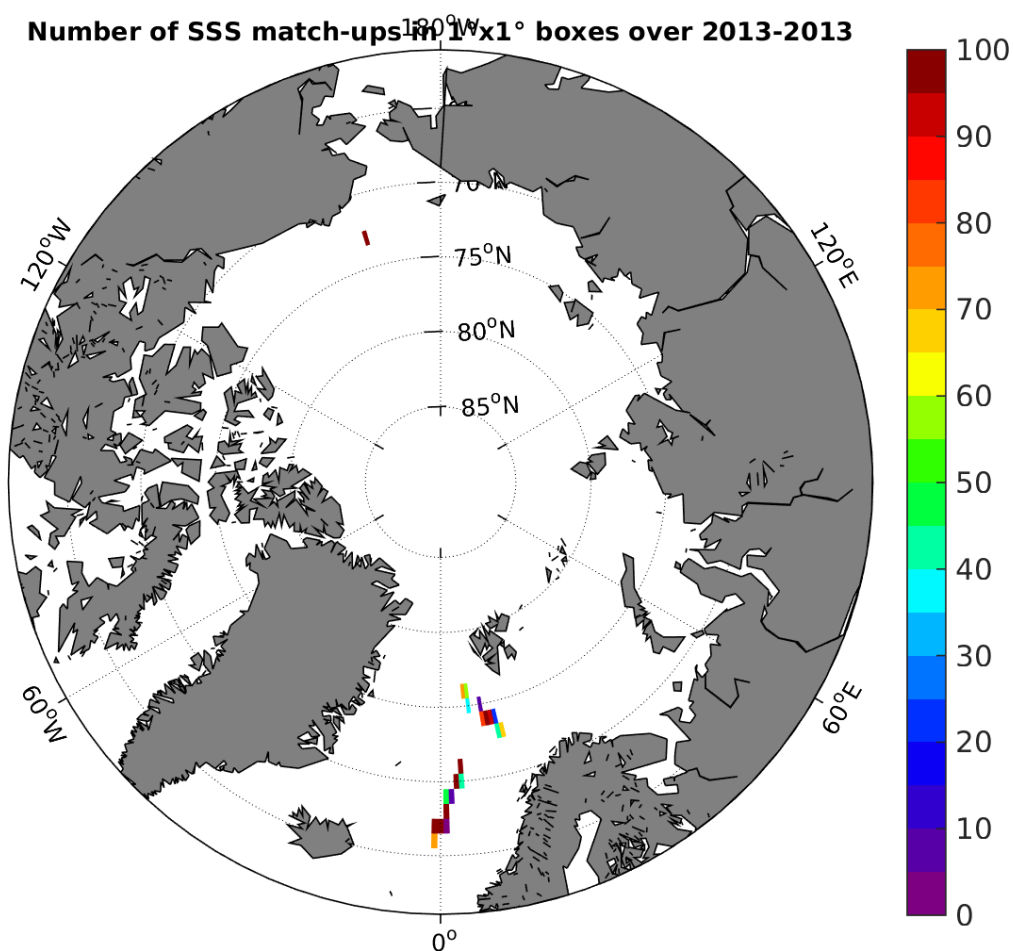
Figure 4: Number of SSS match-ups between TSG-GOSUD-Sailing-ship SSS and the SMOS-L3-ICDC-V3-MONTHLY-0.5DEG SSS product for the Arctic Ocean Pi-MEP region over 1°x1° boxes and for the full satellite product period.
