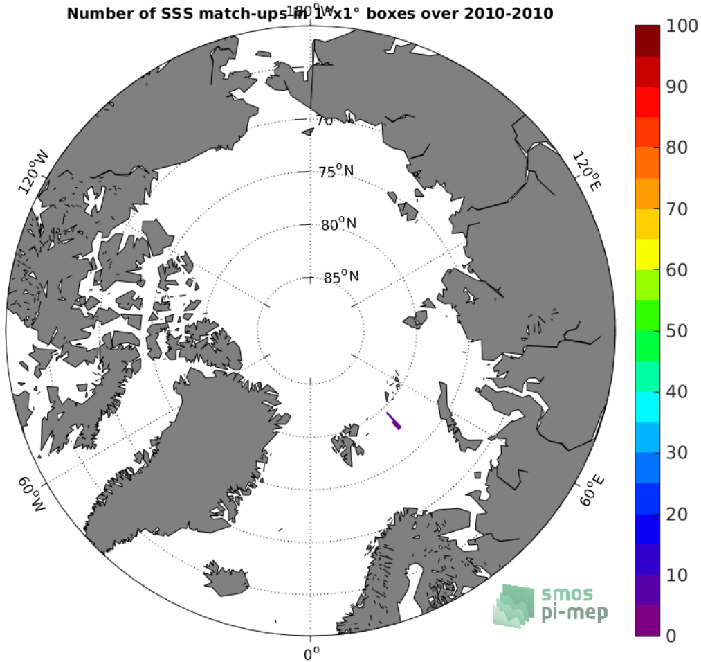
Figure 4: Number of SSS match-ups between Marine mammals SSS and the SMOS SSS L3 v3 Monthly (ICDC) SSS product for the Arctic Ocean Pi-MEP region over 1^\circ \times 1^\circ boxes and for the full satellite product period.
