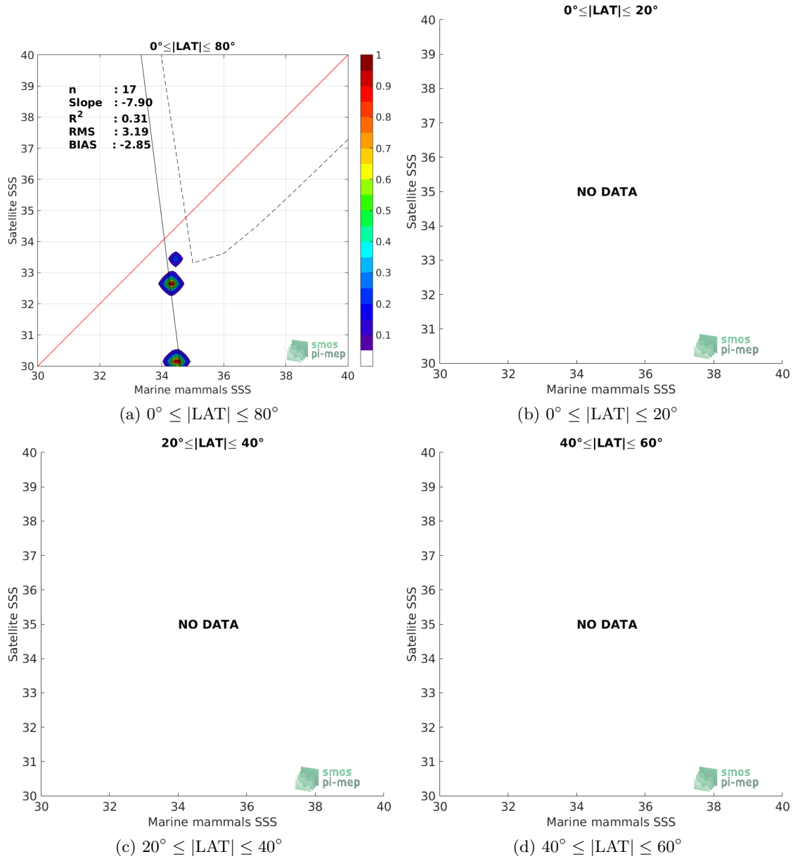
Figure 9: Contour maps of the concentration of SMOS SSS L3 v3 Monthly (ICDC) SSS (y-axis) versus Marine mammals SSS (x-axis) at match-up pairs for different latitude bands. For each plot, the red line shows x=y . The black thin and dashed lines indicate a linear fit through the data cloud and the \pm 95\% confidence levels, respectively. The number match-up pairs n , the slope and R^2 coefficient of the linear fit, the root mean square (RMS) and the mean bias between satellite and in situ data are indicated for each latitude band in each plots.
