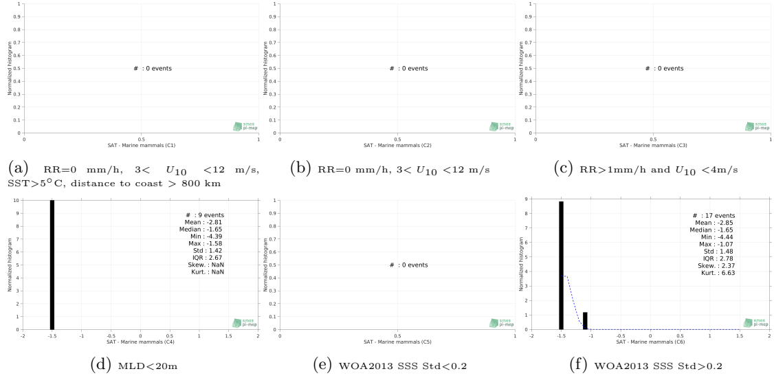
Figure 13: Normalized histogram of \Delta\text{SSS} (SMOS SSS L3 v3 Monthly (ICDC) - Marine mammals) for 6 different subdatasets corresponding to: RR=0 mm/h, 3 < U_{10} < 12 m/s, SST > 5^\circ\text{C} , distance to coast > 800 km (a), RR=0 mm/h, 3 < U_{10} < 12 m/s (b), RR > 1\text{mm/h} and U_{10} < 4\text{m/s} (c), MLD < 20\text{m} (d), WOA2013 SSS Std < 0.2 (e), WOA2013 SSS Std > 0.2 (f).
