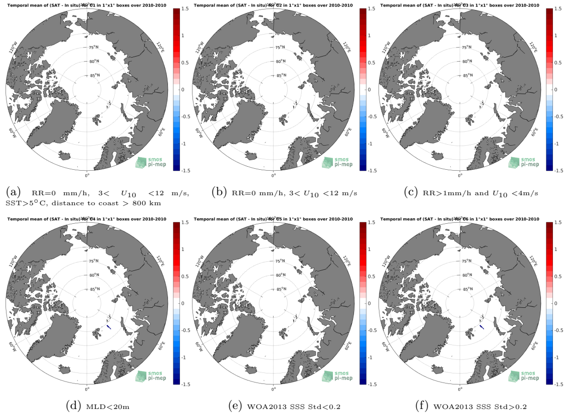
Figure 12: Temporal mean gridded over spatial boxes of size 1^{\circ} \times 1^{\circ} of \Delta\text{SSS} (SMOS SSS L3 v3 Monthly (ICDC) - Marine mammals) for 6 different subdatasets corresponding to: RR=0 mm/h, 3 < U_{10} < 12 m/s, SST > 5^{\circ}\text{C} , distance to coast > 800 km (a), RR=0 mm/h, 3 < U_{10} < 12 m/s (b), RR > 1 mm/h and U_{10} < 4 m/s (c), MLD < 20\text{m} (d), WOA2013 SSS Std < 0.2 (e), WOA2013 SSS Std > 0.2 (f).
