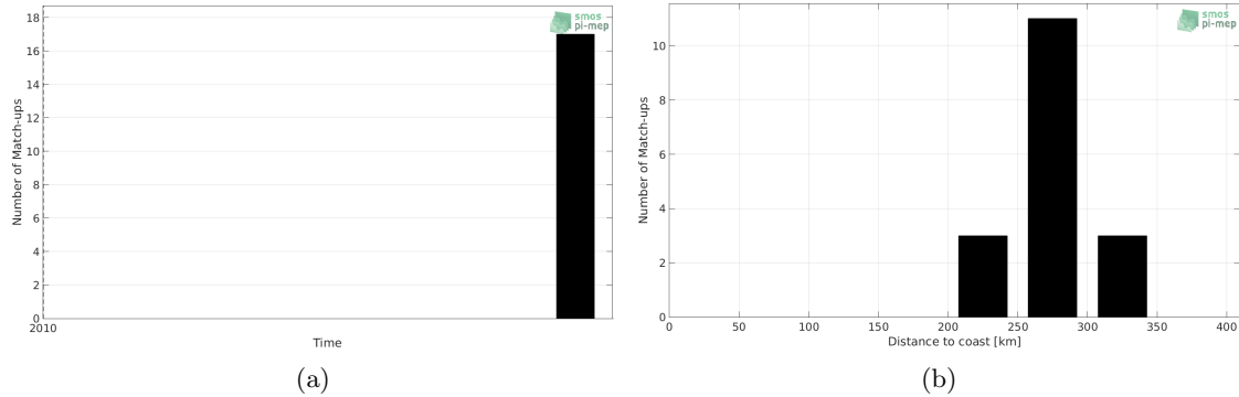
Figure 1: Number of match-ups between Marine mammals and SMOS SSS L3 v3 Monthly (ICDC) SSS as a function of time (a) and as function of the distance to coast (b) over the Arctic Ocean Pi-MEP region and for the full satellite product period.
