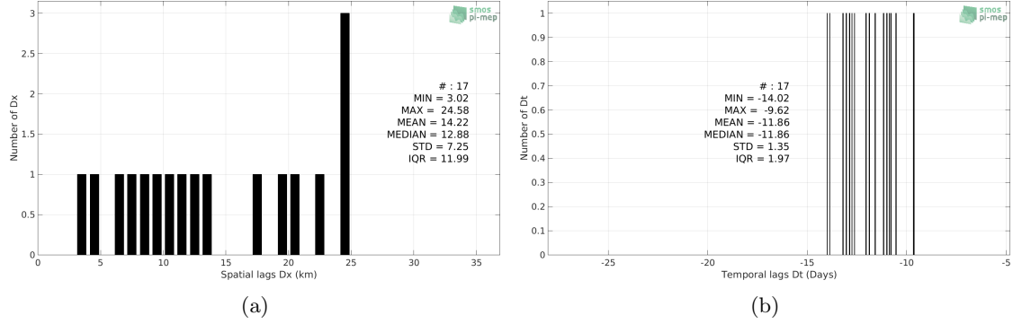
Figure 5: Histograms of the spatial (a) and temporal (b) lags between the location/time of the Marine mammals measurement and the date of the corresponding SMOS SSS L3 v3 Monthly (ICDC) SSS pixel.
