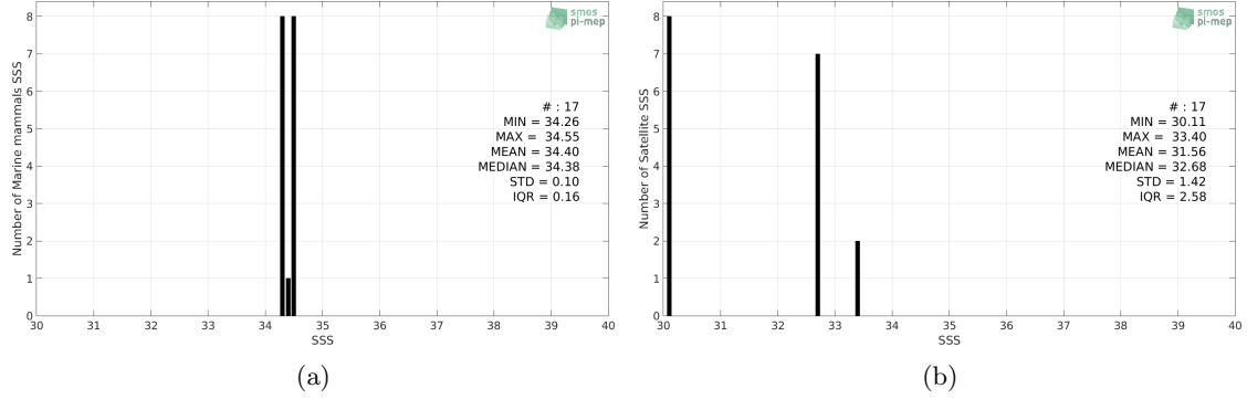
Figure 2: Histograms of SSS from Marine mammals (a) and SMOS SSS L3 v3 Monthly (ICDC) (b) considering all match-up pairs per bins of 0.1 over the Arctic Ocean Pi-MEP region and for the full satellite product period.
