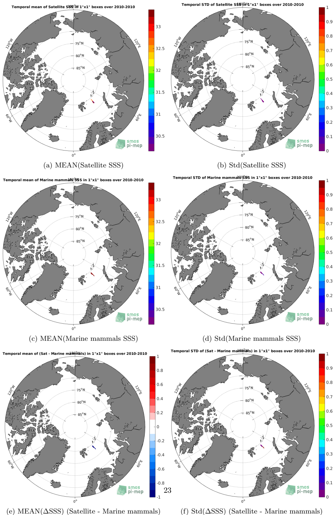
Figure 6: Temporal mean (left) and Std (right) of SSS from SMOS SSS L3 v3 Monthly (ICDC) (top), Marine mammals (middle), and of \Delta SSS (Satellite - Marine mammals). Only match-up pairs are used to generate these maps.
