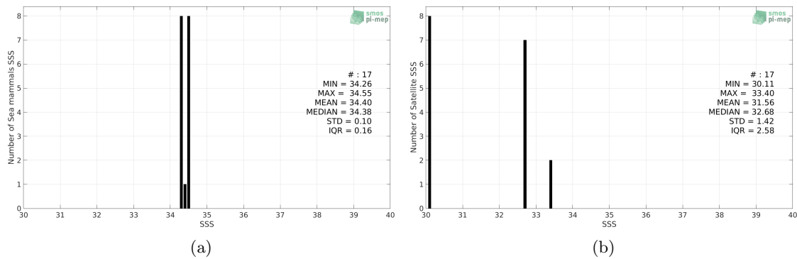
Figure 2: Histograms of SSS from Sea mammals (a) and SMOS SSS L3 v3 Monthly (ICDC) (b) considering all match-up pairs per bins of 0.1 over the Arctic Ocean Pi-MEP region and for the full satellite product period.
