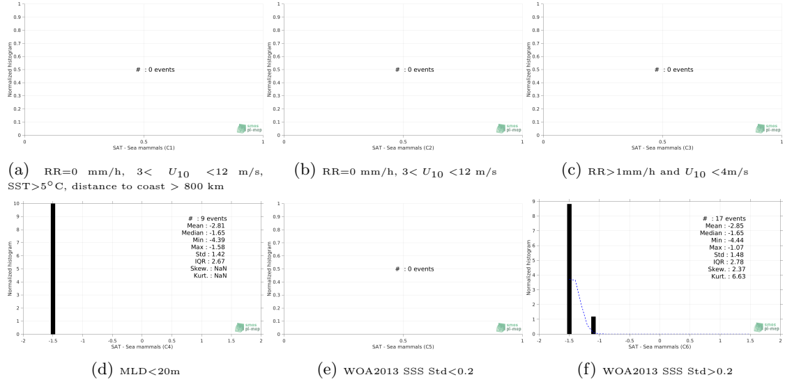
Figure 13: Normalized histogram of \Delta\text{SSS} (SMOS SSS L3 v3 Monthly (ICDC) - Sea mammals) for 6 different subdatasets corresponding to: RR=0 mm/h, 3 < U_{10} < 12 m/s, SST > 5^{\circ}\text{C} , distance to coast > 800 km (a), RR=0 mm/h, 3 < U_{10} < 12 m/s (b), RR > 1\text{mm/h} and U_{10} < 4\text{m/s} (c), MLD < 20\text{m} (d), WOA2013 SSS Std < 0.2 (e), WOA2013 SSS Std > 0.2 (f).
