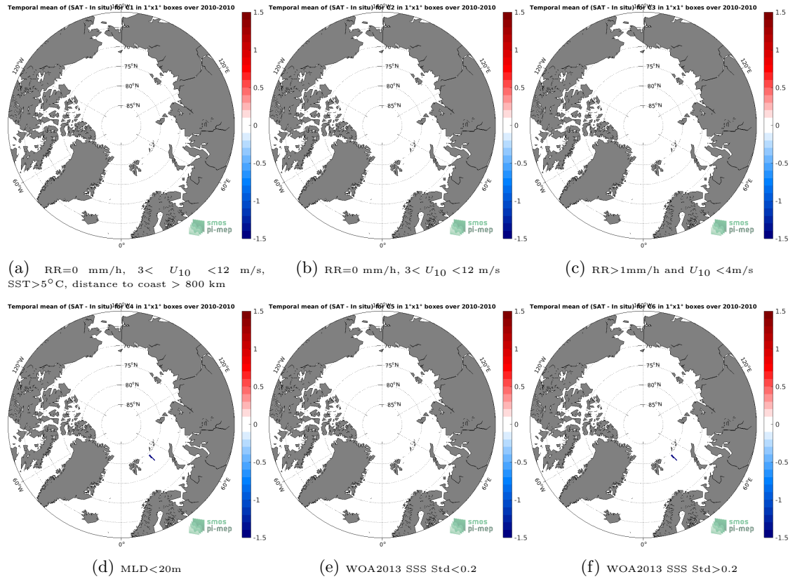
Figure 12: Temporal mean gridded over spatial boxes of size 1^{\circ}\times 1^{\circ} of \Delta\text{SSS} (SMOS SSS L3 v3 Monthly (ICDC) - Sea mammals) for 6 different subdatasets corresponding to:RR=0 mm/h, 3 < U_{10} < 12 m/s, SST >5^{\circ}\text{C} , distance to coast > 800 km (a), RR=0 mm/h, 3 < U_{10} < 12 m/s (b), RR >1 mm/h and U_{10} < 4 m/s (c),MLD <20 m (d),WOA2013 SSS Std <0.2 (e),WOA2013 SSS Std >0.2 (f).
