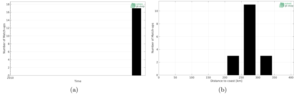
Figure 1: Number of match-ups between Sea mammals and SMOS SSS L3 v3 Monthly (ICDC) SSS as a function of time (a) and as function of the distance to coast (b) over the Arctic Ocean Pi-MEP region and for the full satellite product period.
