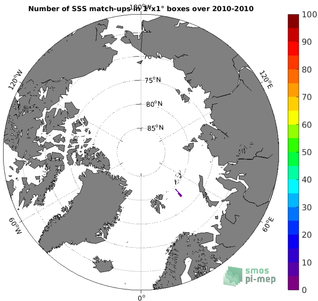
Figure 4: Number of SSS match-ups between Sea mammals SSS and the SMOS SSS L3 v3 Monthly (ICDC) SSS product for the Arctic Ocean Pi-MEP region over 1°x1° boxes and for the full satellite product period.
