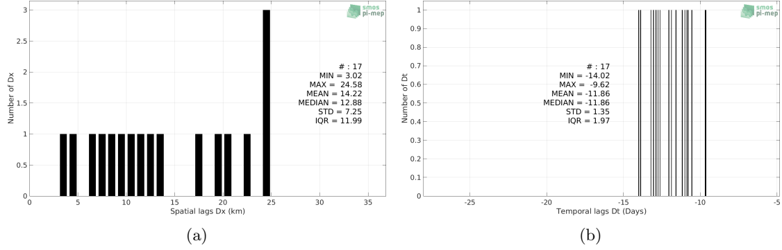
Figure 5: Histograms of the spatial (a) and temporal (b) lags between the time of the Sea mammals measurements and the date of the corresponding SMOS SSS L3 v3 Monthly (ICDC) SSS product.
