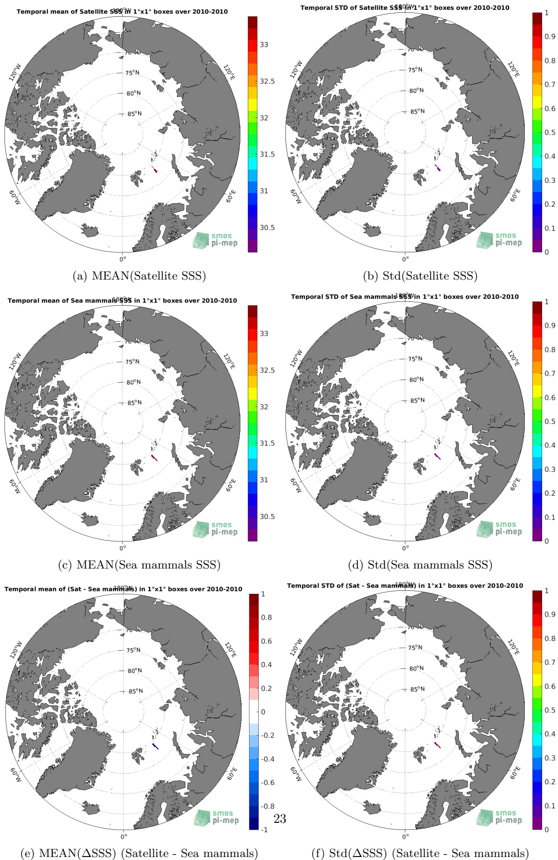
Figure 6: Temporal mean (left) and Std (right) of SSS from SMOS SSS L3 v3 Monthly (ICDC) (top), Sea mammals (middle), and of \Delta SSS (Satellite - Sea mammals). Only match-up pairs are used to generate these maps.
