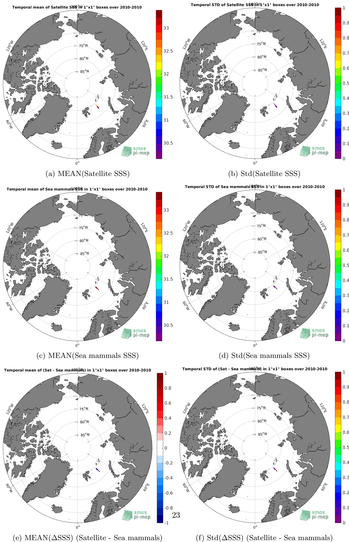
Figure 6: Temporal mean (left) and Std (right) of SSS from SMOS-L3-ICDC-V3-MONTHLY-0.5DEG (top), Sea mammals (middle), and of \Delta SSS (Satellite - Sea mammals). Only match-up pairs are used to generate these maps.
