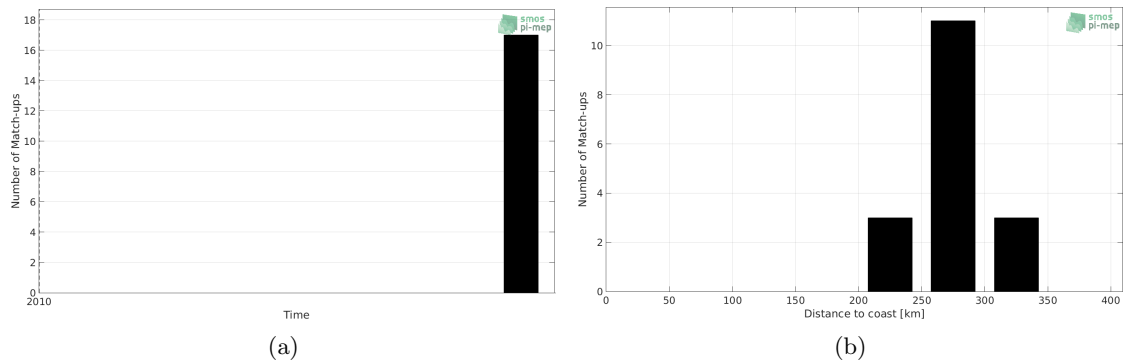
Figure 1: Number of match-ups between Sea mammals and SMOS-L3-ICDC-V3-MONTHLY-0.5DEG SSS as a function of time (a) and as function of the distance to coast (b) over the Arctic Ocean Pi-MEP region and for the full satellite product period.
