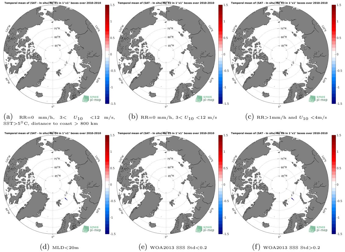
Figure 12: Temporal mean gridded over spatial boxes of size 1^\circ \times 1^\circ of \Delta SSS (SMOS-L3-ICDC-V3-MONTHLY-0.5DEG - Sea mammals) for 6 different subdatasets corresponding to: RR=0 mm/h, 3 < U_{10} < 12 m/s, SST > 5^\circ C , distance to coast > 800 km (a), RR=0 mm/h, 3 < U_{10} < 12 m/s (b), RR > 1 mm/h and U_{10} < 4 m/s (c), MLD < 20 m (d), WOA2013 SSS Std < 0.2 (e), WOA2013 SSS Std > 0.2 (f).
