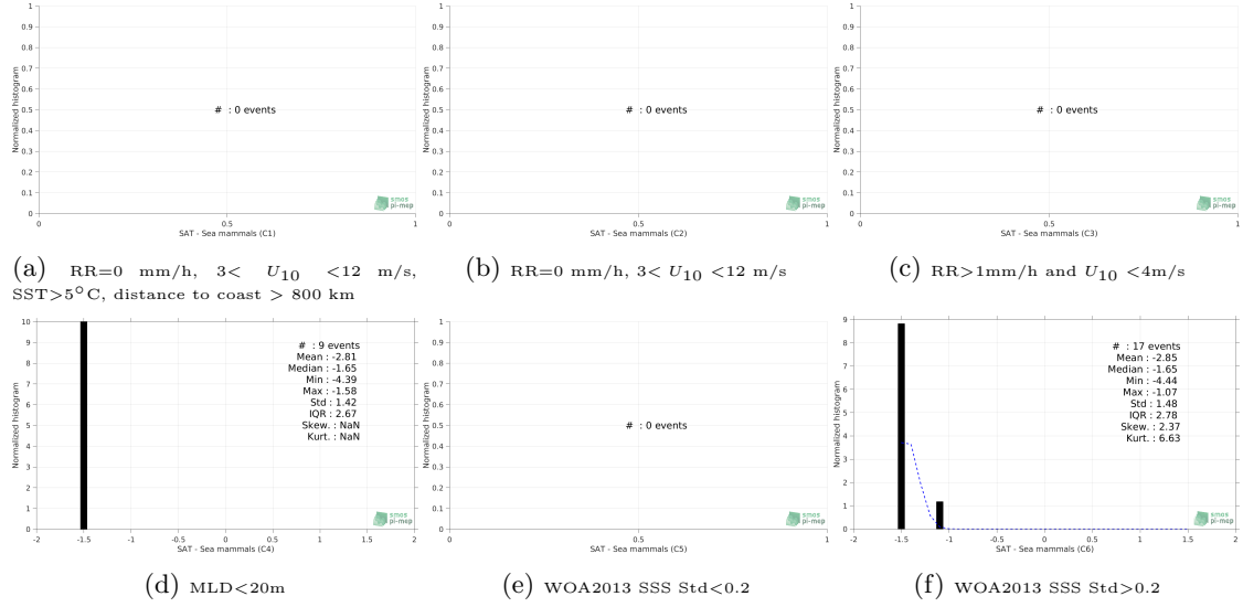
Figure 13: Normalized histogram of \Delta SSS (SMOS-L3-ICDC-V3-MONTHLY-0.5DEG - Sea mammals) for 6 different subdatasets corresponding to: RR=0 mm/h, 3 < U_{10} < 12 m/s, SST > 5^\circ\text{C} , distance to coast > 800 km (a), RR=0 mm/h, 3 < U_{10} < 12 m/s (b), RR > 1\text{mm/h} and U_{10} < 4\text{m/s} (c), MLD < 20\text{m} (d), WOA2013 SSS Std < 0.2 (e), WOA2013 SSS Std > 0.2 (f).
