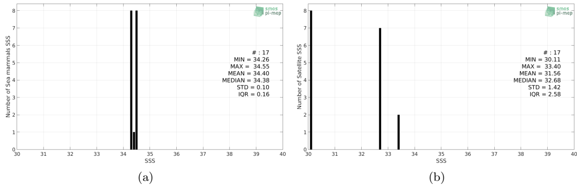
Figure 2: Histograms of SSS from Sea mammals (a) and SMOS-L3-ICDC-V3-MONTHLY-0.5DEG (b) considering all match-up pairs per bins of 0.1 over the Arctic Ocean Pi-MEP region and for the full satellite product period.
