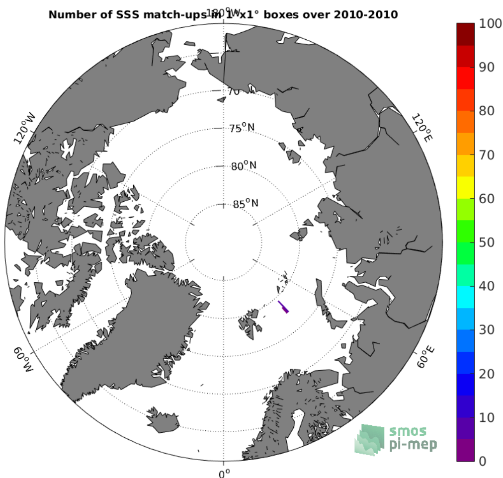
Figure 4: Number of SSS match-ups between Sea mammals SSS and the SMOS-L3-ICDC-V3-MONTHLY-0.5DEG SSS product for the Arctic Ocean Pi-MEP region over 1^\circ \times 1^\circ boxes and for the full satellite product period.
