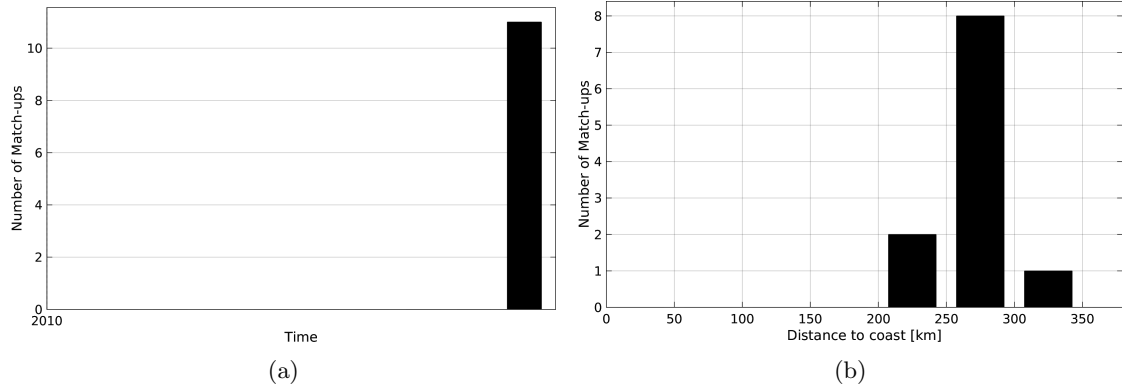
Figure 1: Number of match-ups between Sea mammals and SMOS-L3-ICDC-V3-MONTHLY-0.5DEG SSS as a function of time (a) and as function of the distance to coast (b) over the Arctic Ocean Pi-MEP region and for the full satellite product period.
