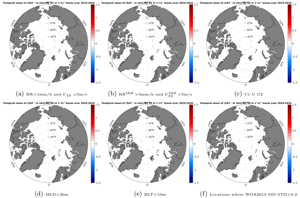
Figure 12: Temporal mean gridded over spatial boxes of size 1^\circ \times 1^\circ of \Delta SSS (SMOS-L3-ICDC-V3-MONTHLY-0.5DEG - Sea mammals) for 6 different subdatasets corresponding to: RR > 1mm/h and U_{10} < 5 m/s (a), RR^{10d} > 5 mm/h and U_{10}^{10d} < 5 m/s (b), C1 U C2 (c), MLD < 20m (d), BLT > 10m (e), Locations where WOA2013 SSS STD > 0.2 (f).
