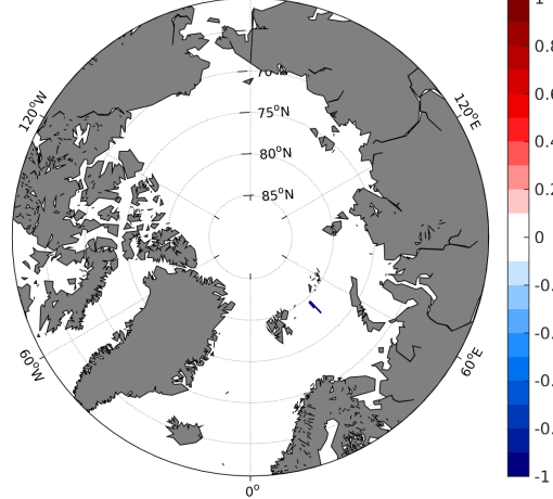
(e) MEAN( \Delta SSS) (Satellite - Sea mammals) 18
