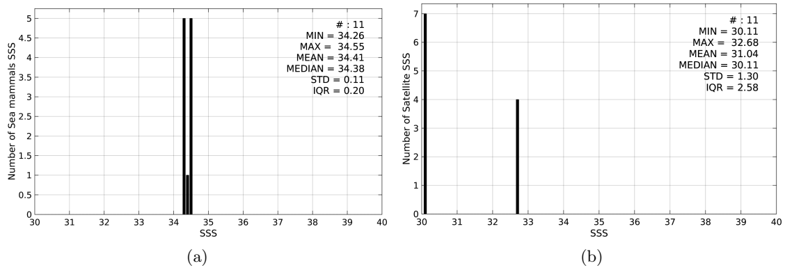
Figure 2: Histograms of SSS from Sea mammals (a) and SMOS-L3-ICDC-V3-MONTHLY-0.5DEG (b) considering all match-up pairs per bins of 0.1 over the Arctic Ocean Pi-MEP region and for the full satellite product period.
