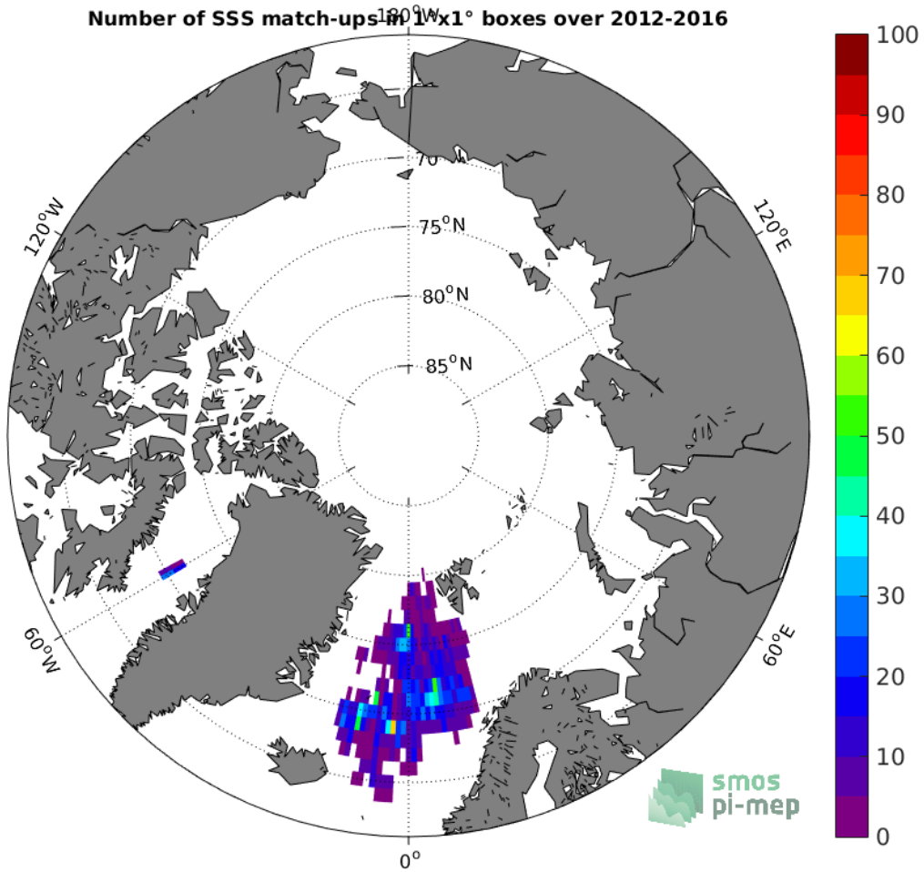
Figure 4: Number of SSS match-ups between Argo SSS and the SMOS SSS L3 v3 Monthly (ICDC) SSS product for the Arctic Ocean Pi-MEP region over 1^\circ \times 1^\circ boxes and for the full satellite product period.
