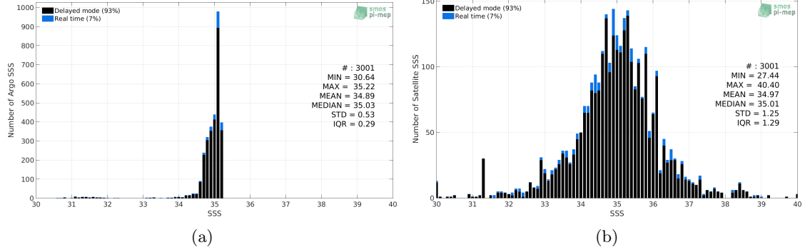
Figure 2: Histograms of SSS from Argo (a) and SMOS SSS L3 v3 Monthly (ICDC) (b) considering all match-up pairs per bins of 0.1 over the Arctic Ocean Pi-MEP region and for the full satellite product period.
