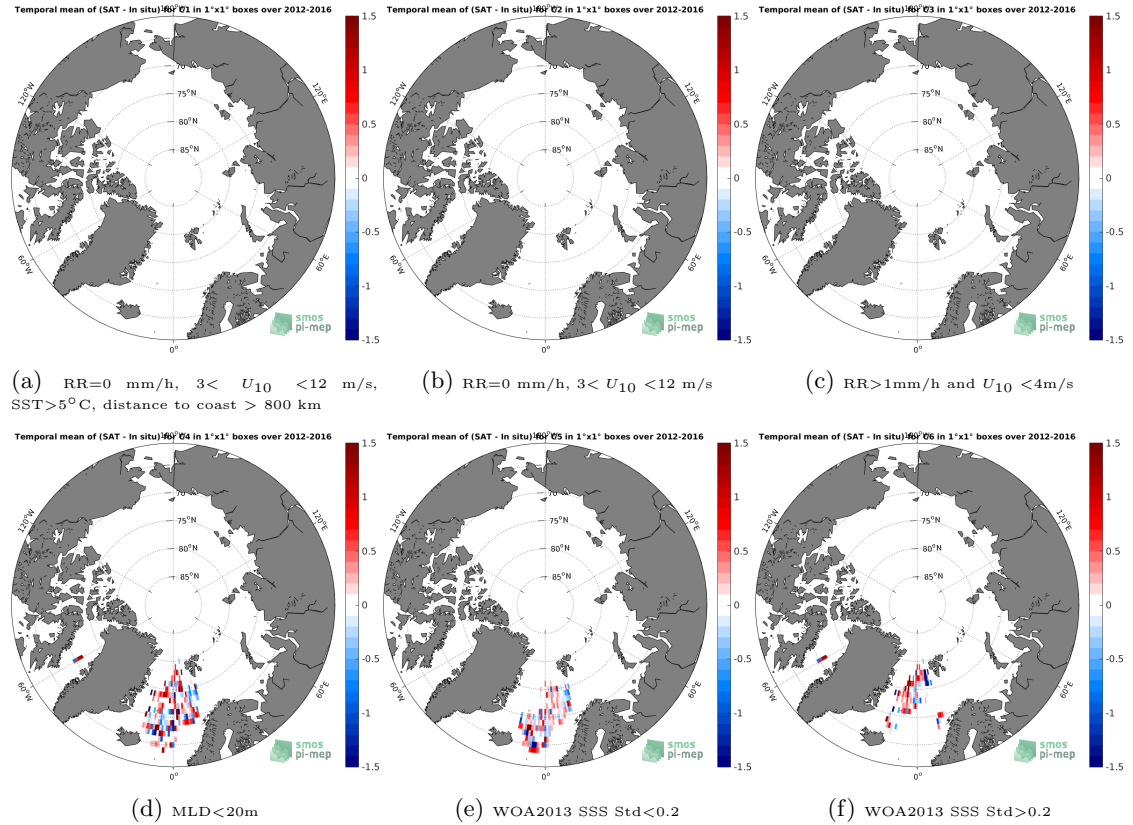
Figure 12: Temporal mean gridded over spatial boxes of size 1^{\circ} \times 1^{\circ} of \Delta\text{SSS} (SMOS SSS L3 v3 Monthly (ICDC) - Argo) for 6 different subdatasets corresponding to: RR=0 mm/h, 3 < U_{10} < 12 m/s, SST >5^{\circ}\text{C} , distance to coast > 800 km (a), RR=0 mm/h, 3 < U_{10} < 12 m/s (b), RR >1\text{mm/h} and U_{10} < 4\text{m/s} (c), MLD <20\text{m} (d), WOA2013 SSS Std <0.2 (e), WOA2013 SSS Std >0.2 (f).
