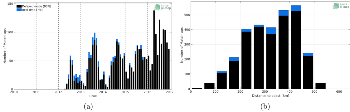
Figure 1: Number of match-ups between Argo and SMOS SSS L3 v3 Monthly (ICDC) SSS as a function of time (a) and as function of the distance to coast (b) over the Arctic Ocean Pi-MEP region and for the full satellite product period.
