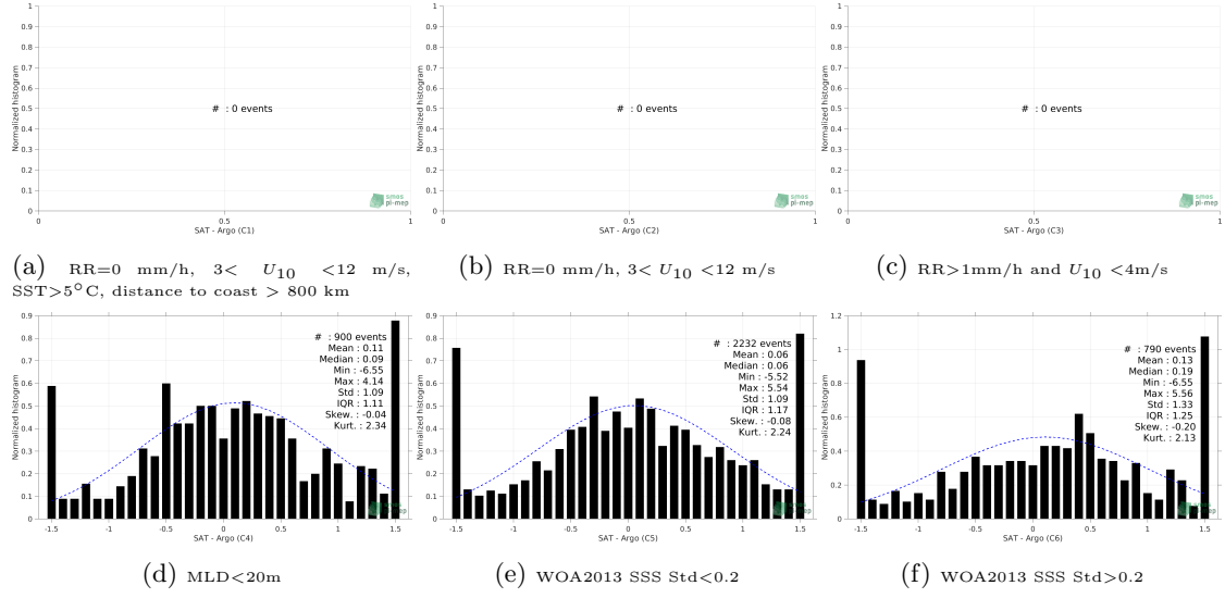
Figure 13: Normalized histogram of \Delta\text{SSS} (SMOS SSS L3 v3 Monthly (ICDC) - Argo) for 6 different subdatasets corresponding to: RR=0 mm/h, 3 < U_{10} < 12 m/s, SST > 5^\circ\text{C} , distance to coast > 800 km (a), RR=0 mm/h, 3 < U_{10} < 12 m/s (b), RR > 1 mm/h and U_{10} < 4 m/s (c), MLD < 20 m (d), WOA2013 SSS Std < 0.2 (e), WOA2013 SSS Std > 0.2 (f).
