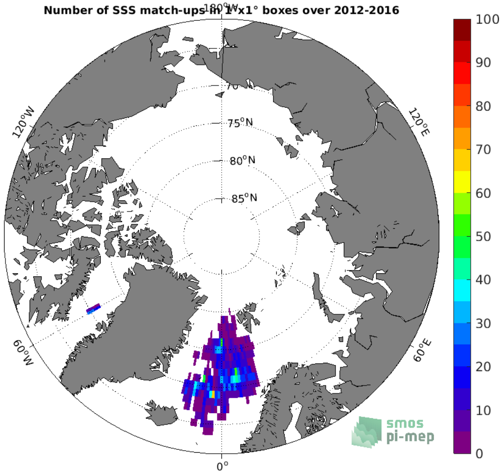
Figure 4: Number of SSS match-ups between Argo SSS and the SMOS SSS L3 v3 Monthly (ICDC) SSS product for the Arctic Ocean Pi-MEP region over 1°x1° boxes and for the full satellite product period.
