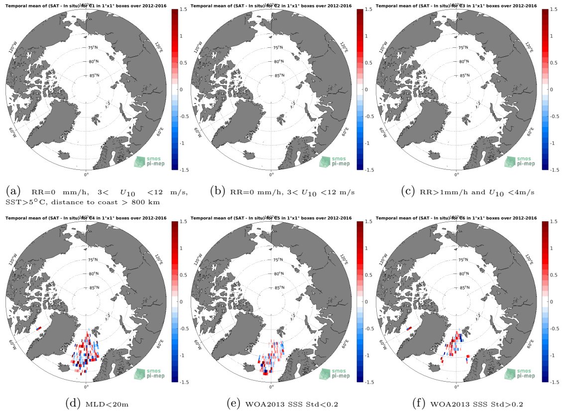
Figure 12: Temporal mean gridded over spatial boxes of size 1^{\circ}\times 1^{\circ} of \Delta\text{SSS} (SMOS SSS L3 v3 Monthly (ICDC) - Argo) for 6 different subdatasets corresponding to:RR=0 mm/h, 3 < U_{10} < 12 m/s, SST >5^{\circ}\text{C} , distance to coast > 800 km (a), RR=0 mm/h, 3 < U_{10} < 12 m/s (b), RR >1\text{mm/h} and U_{10} < 4\text{m/s} (c),MLD <20\text{m} (d),WOA2013 SSS Std <0.2 (e),WOA2013 SSS Std >0.2 (f).
