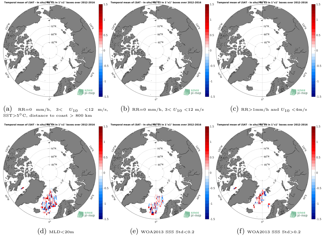
Figure 12: Temporal mean gridded over spatial boxes of size 1^{\circ}\times 1^{\circ} of \Delta\text{SSS} (SMOS-L3-ICDC-V3-MONTHLY-0.5DEG - Argo) for 6 different subdatasets corresponding to: RR=0 mm/h, 3 < U_{10} < 12 m/s, SST >5^{\circ}\text{C} , distance to coast > 800 km (a), RR=0 mm/h, 3 < U_{10} < 12 m/s (b), RR >1\text{mm/h} and U_{10} < 4\text{m/s} (c), MLD <20\text{m} (d), WOA2013 SSS Std <0.2 (e), WOA2013 SSS Std >0.2 (f).
