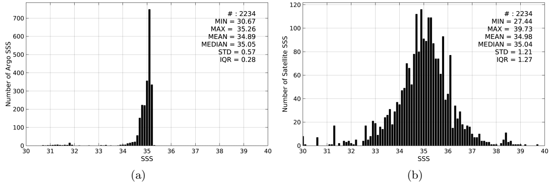
Figure 2: Histograms of SSS from Argo (a) and SMOS-L3-ICDC-V3-MONTHLY-0.5DEG (b) considering all match-up pairs per bins of 0.1 over the Arctic Ocean Pi-MEP region and for the full satellite product period.
