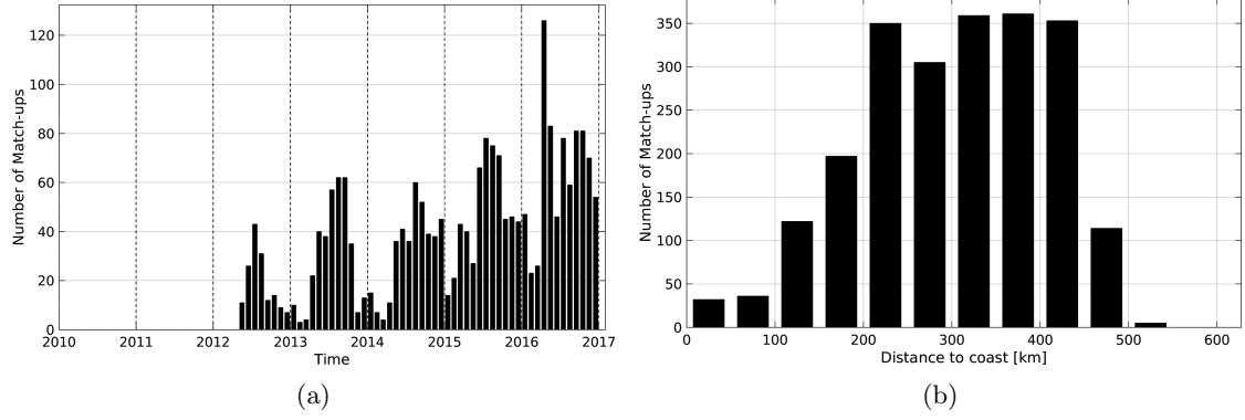
Figure 1: Number of match-ups between Argo and SMOS-L3-ICDC-V3-MONTHLY-0.5DEG SSS as a function of time (a) and as function of the distance to coast (b) over the Arctic Ocean Pi-MEP region and for the full satellite product period.
