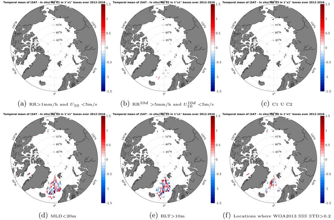
Figure 12: Temporal mean gridded over spatial boxes of size 1^\circ \times 1^\circ of \Delta SSS (SMOS-L3-ICDC-V3-MONTHLY-0.5DEG - Argo) for 6 different subdatasets corresponding to: RR > 1mm/h and U_{10} < 5\text{m/s} (a), RR^{10d} > 5\text{mm/h} and U_{10}^{10d} < 5\text{m/s} (b), C1 U C2 (c), MLD < 20m (d), BLT > 10m (e), Locations where WOA2013 SSS STD > 0.2 (f).
