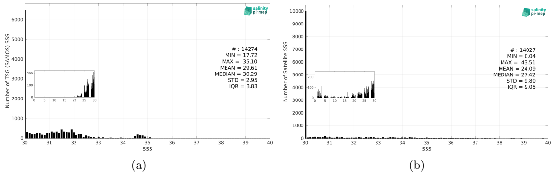
Figure 3: Histograms of SSS from TSG (SAMOS) (a) and SMOS SSS L2Q v331 - With FLAG (CMEMS-CATDS-CPDC) (b) considering all match-up pairs per bins of 0.1 over the Arctic Ocean Pi-MEP region and for the full satellite product period.
