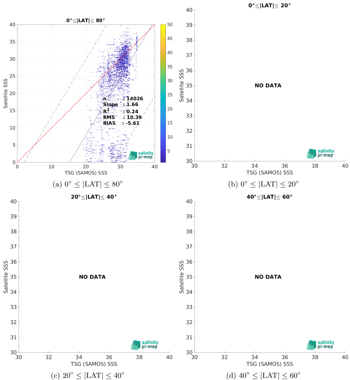
Figure 10: Contour maps of the concentration of SMOS SSS L2Q v331 - With FLAG (CMEMS-CATDS-CPDC) SSS (y-axis) versus TSG (SAMOS) SSS (x-axis) at match-up pairs for different latitude bands. For each plot, the red line shows x=y . The black thin and dashed lines indicate a linear fit through the data cloud and the \pm 95\% confidence levels, respectively. The number match-up pairs n , the slope and R^2 coefficient of the linear fit, the root mean square (RMS) and the mean bias between satellite and in situ data are indicated for each latitude band in each plots.
