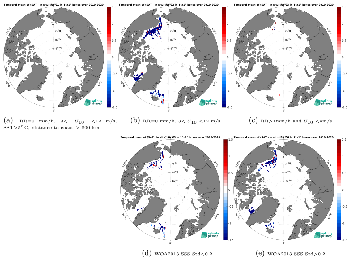
Figure 14: Temporal mean gridded over spatial boxes of size 1^\circ \times 1^\circ of \Delta\text{SSS} (SMOS SSS L2Q v331 - With FLAG (CMEMS-CATDS-CPDC) - TSG (SAMOS)) for 5 different subdatasets corresponding to: RR=0 mm/h, 3 < U_{10} < 12 m/s, SST > 5°C, distance to coast > 800 km (a), RR=0 mm/h, 3 < U_{10} < 12 m/s (b), RR > 1mm/h and U_{10} < 4 m/s (c), WOA2013 SSS Std < 0.2 (d), WOA2013 SSS Std > 0.2 (e).
