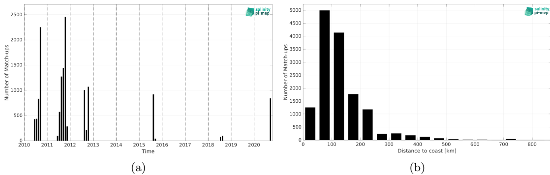
Figure 2: Number of match-ups between TSG (SAMOS) and SMOS SSS L2Q v331 - With FLAG (CMEMS-CATDS-CPDC) SSS as a function of time (a) and as function of the distance to coast (b) over the Arctic Ocean Pi-MEP region and for the full satellite product period.
