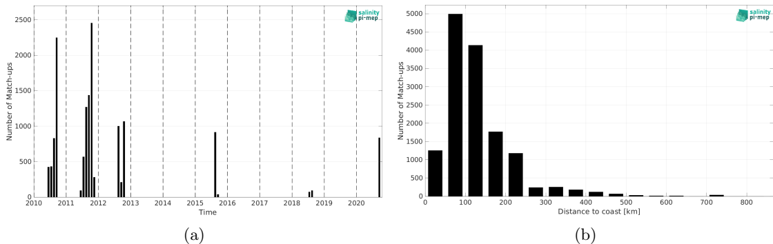
Figure 1: Number of match-ups between TSG (SAMOS) and SMOS SSS L2Q v331 - With FLAG (CMEMS-CATDS-CPDC) SSS as a function of time (a) and as function of the distance to coast (b) over the Arctic Ocean Pi-MEP region and for the full satellite product period.
