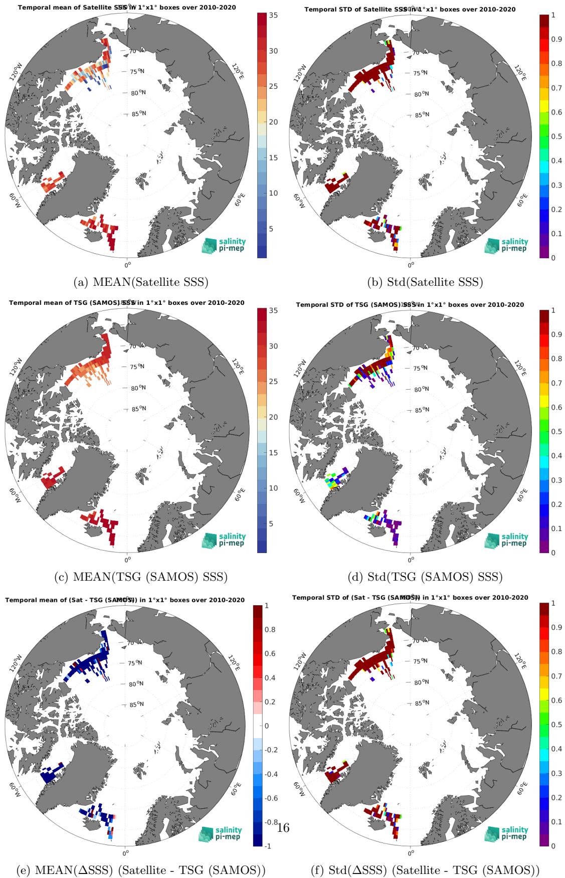
Figure 6: Temporal mean (left) and Std (right) of SSS from SMOS SSS L2Q v331 - With FLAG (CMEMS-CATDS-CPDC) (top), TSG (SAMOS) (middle), and of \Delta SSS (Satellite - TSG (SAMOS)). Only match-up pairs are used to generate these maps.
