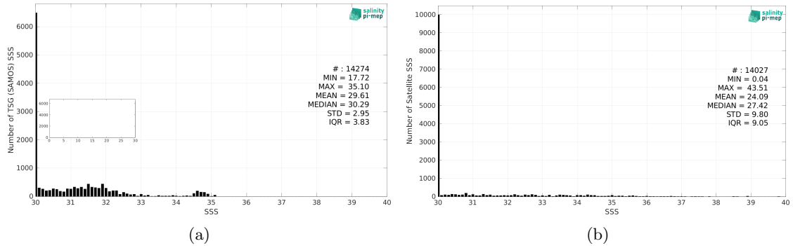
Figure 2: Histograms of SSS from TSG (SAMOS) (a) and SMOS SSS L2Q v331 - With FLAG (CMEMS-CATDS-CPDC) (b) considering all match-up pairs per bins of 0.1 over the Arctic Ocean Pi-MEP region and for the full satellite product period.
