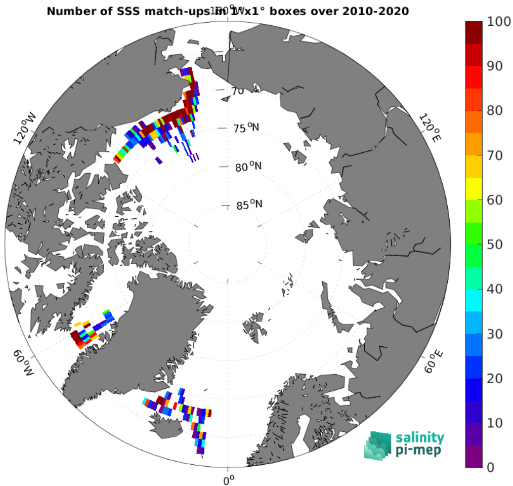
Figure 4: Number of SSS match-ups between TSG (SAMOS) SSS and the SMOS SSS L2Q v331 - With FLAG (CMEMS-CATDS-CPDC) SSS product for the Arctic Ocean Pi-MEP region over 1^\circ \times 1^\circ boxes and for the full satellite product period.
