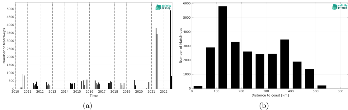
Figure 2: Number of match-ups between TSG (Polarstern) and SMOS SSS L2Q v331 - With FLAG (CMEMS-CATDS-CPDC) SSS as a function of time (a) and as function of the distance to coast (b) over the Arctic Ocean Pi-MEP region and for the full satellite product period.
