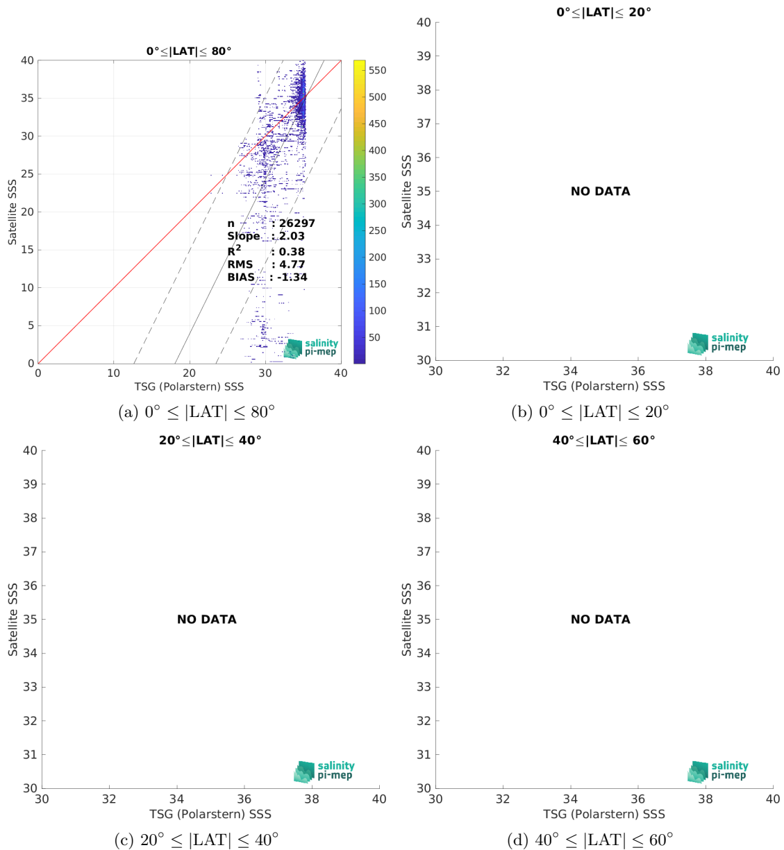
Figure 10: Contour maps of the concentration of SMOS SSS L2Q v331 - With FLAG (CMEMS-CATDS-CPDC) SSS (y-axis) versus TSG (Polarstern) SSS (x-axis) at match-up pairs for different latitude bands. For each plot, the red line shows x=y . The black thin and dashed lines indicate a linear fit through the data cloud and the \pm 95\% confidence levels, respectively. The number match-up pairs n , the slope and R^2 coefficient of the linear fit, the root mean square (RMS) and the mean bias between satellite and in situ data are indicated for each latitude band in each plots.
