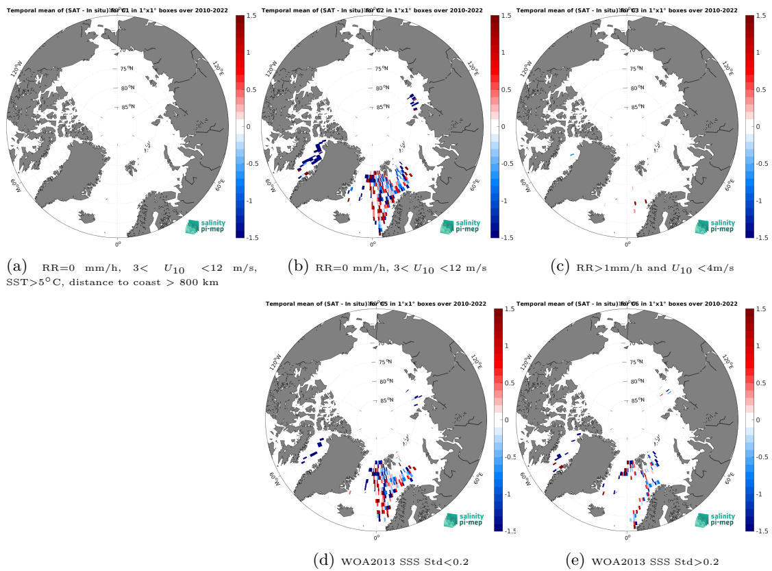
Figure 14: Temporal mean gridded over spatial boxes of size 1^\circ \times 1^\circ of \Delta SSS (SMOS SSS L2Q v331 - With FLAG (CMEMS-CATDS-CPDC) - TSG (Polarstern)) for 5 different subdatasets corresponding to: RR=0 mm/h, 3 < U_{10} < 12 m/s, SST > 5°C, distance to coast > 800 km (a), RR=0 mm/h, 3 < U_{10} < 12 m/s (b), RR > 1mm/h and U_{10} < 4 m/s (c), WOA2013 SSS Std < 0.2 (d), WOA2013 SSS Std > 0.2 (e).
