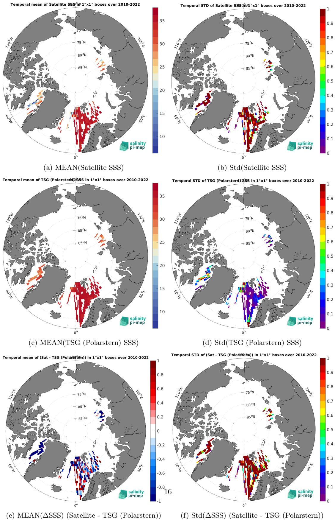
Figure 7: Temporal mean (left) and Std (right) of SSS from SMOS SSS L2Q v331 - With FLAG (CMEMS-CATDS-CPDC) (top), TSG (Polarstern) (middle), and of \Delta SSS (Satellite - TSG (Polarstern)). Only match-up pairs are used to generate these maps.
