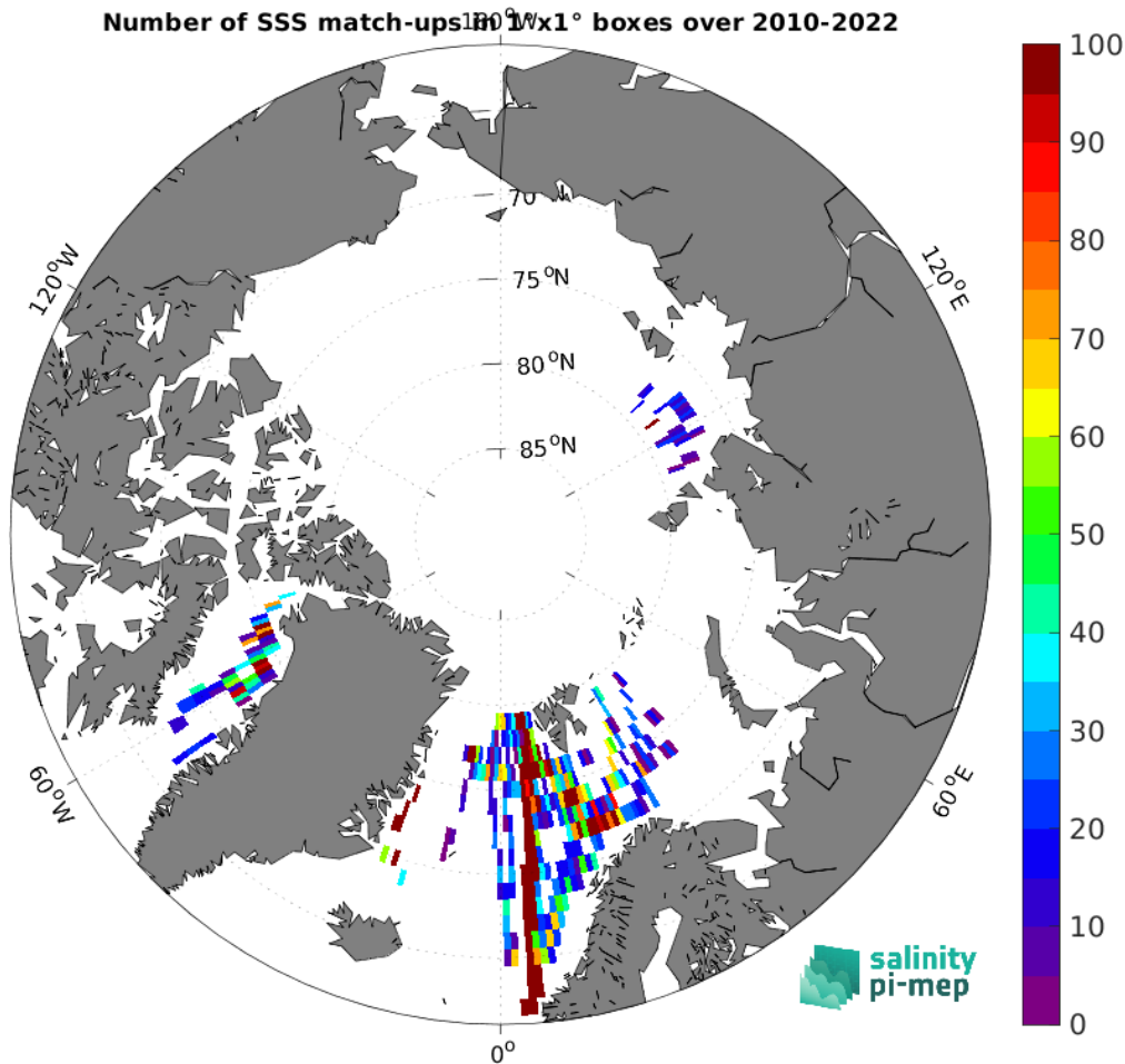
Figure 5: Number of SSS match-ups between TSG (Polarstern) SSS and the SMOS SSS L2Q v331 - With FLAG (CMEMS-CATDS-CPDC) SSS product for the Arctic Ocean Pi-MEP region over 1^\circ \times 1^\circ boxes and for the full satellite product period.
