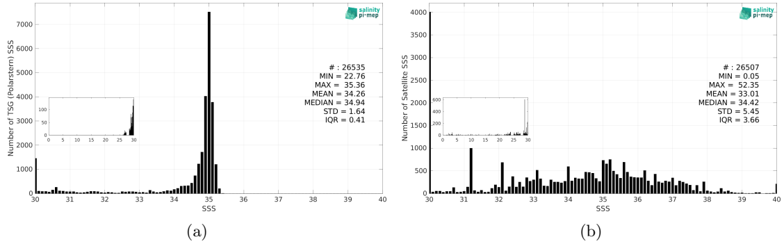
Figure 3: Histograms of SSS from TSG (Polarstern) (a) and SMOS SSS L2Q v331 - With FLAG (CMEMS-CATDS-CPDC) (b) considering all match-up pairs per bins of 0.1 over the Arctic Ocean Pi-MEP region and for the full satellite product period.
