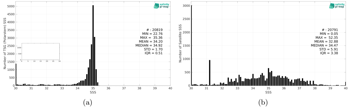
Figure 2: Histograms of SSS from TSG (Polarstern) (a) and SMOS SSS L2Q v331 - With FLAG (CMEMS-CATDS-CPDC) (b) considering all match-up pairs per bins of 0.1 over the Arctic Ocean Pi-MEP region and for the full satellite product period.
