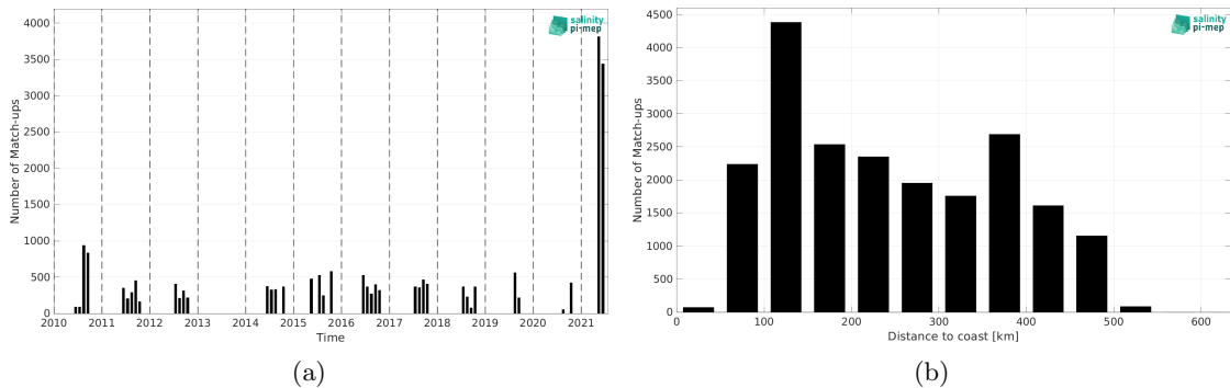
Figure 1: Number of match-ups between TSG (Polarstern) and SMOS SSS L2Q v331 - With FLAG (CMEMS-CATDS-CPDC) SSS as a function of time (a) and as function of the distance to coast (b) over the Arctic Ocean Pi-MEP region and for the full satellite product period.
