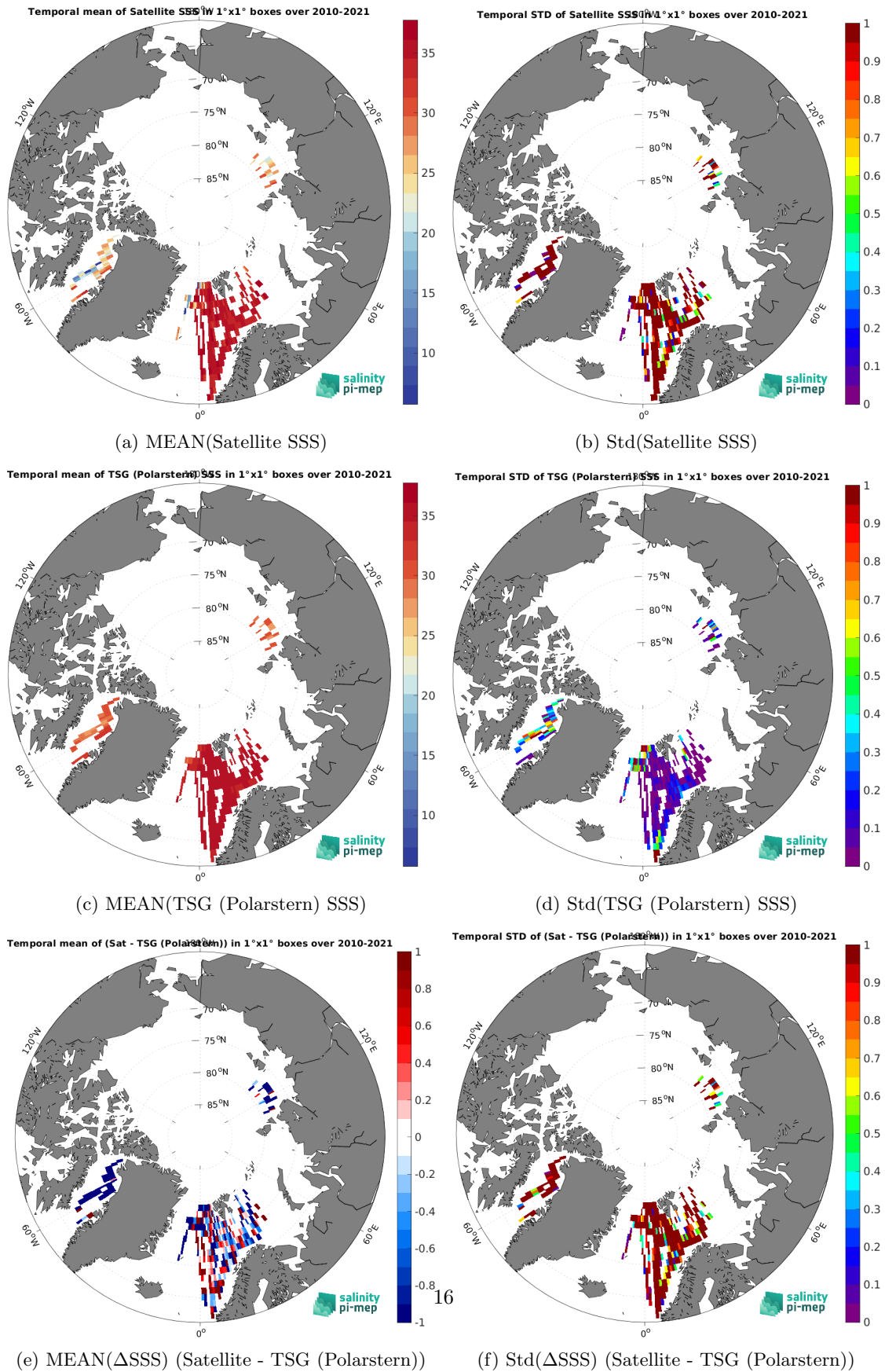
Figure 6: Temporal mean (left) and Std (right) of SSS from SMOS SSS L2Q v331 - With FLAG (CMEMS-CATDS-CPDC) (top), TSG (Polarstern) (middle), and of \Delta SSS (Satellite - TSG (Polarstern)). Only match-up pairs are used to generate these maps.
