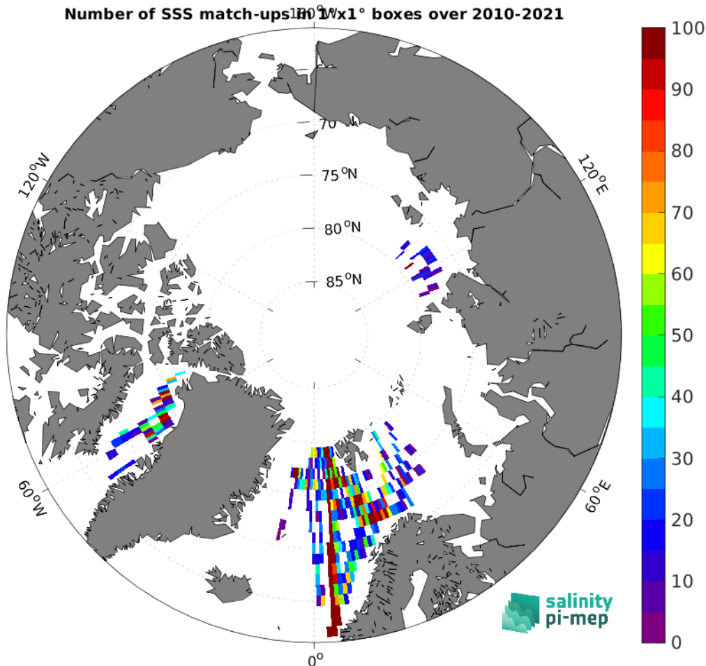
Figure 4: Number of SSS match-ups between TSG (Polarstern) SSS and the SMOS SSS L2Q v331 - With FLAG (CMEMS-CATDS-CPDC) SSS product for the Arctic Ocean Pi-MEP region over 1^\circ \times 1^\circ boxes and for the full satellite product period.
