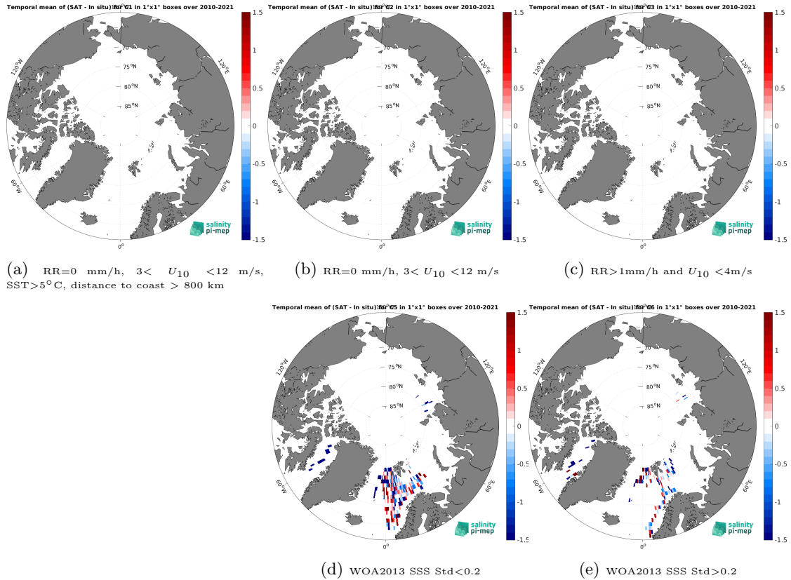
Figure 12: Temporal mean gridded over spatial boxes of size 1^{\circ}\times 1^{\circ} of \Delta\text{SSS} (SMOS SSS L2Q v331 - With FLAG (CMEMS-CATDS-CPDC) - TSG (Polarstern)) for 5 different subdatasets corresponding to:RR=0 mm/h, 3 < U_{10} < 12 m/s, SST > 5^{\circ}\text{C} , distance to coast > 800 km (a), RR=0 mm/h, 3 < U_{10} < 12 m/s (b), RR > 1 mm/h and U_{10} < 4 m/s (c), WOA2013 SSS Std < 0.2 (d), WOA2013 SSS Std > 0.2 (e).
