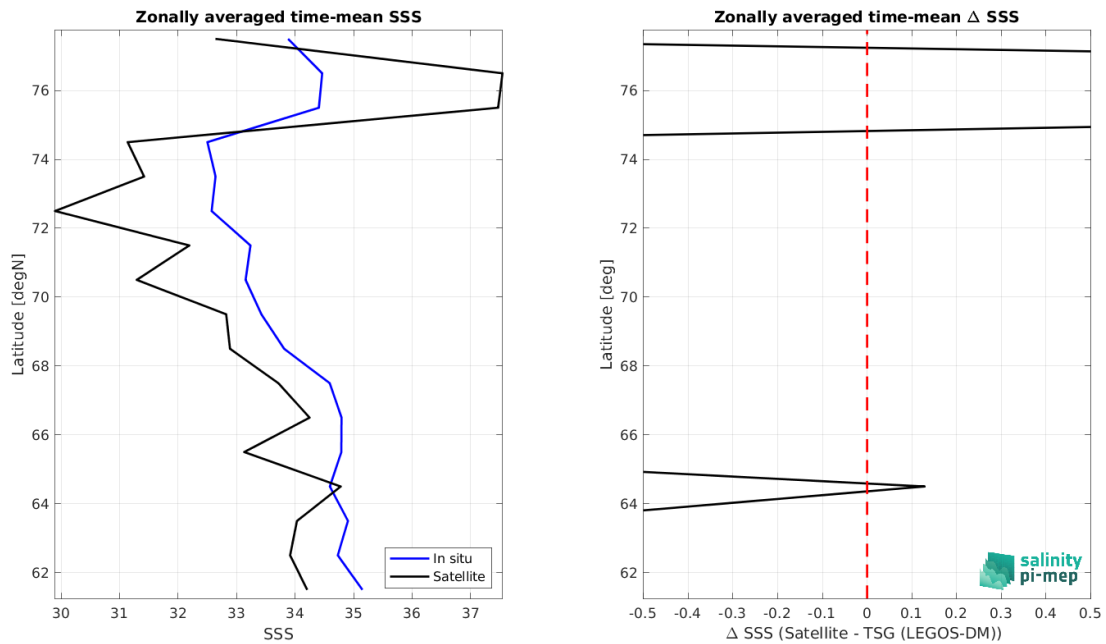
Figure 9: Left panel: Zonal mean SSS from SMOS SSS L2Q v331 - With FLAG (CMEMS-CATDS-CPDC) satellite product (black) and from TSG (LEGOS-DM) (blue). Right panel: Zonal mean of \Delta SSS (Satellite - TSG (LEGOS-DM)) for all the collected Pi-MEP match-up pairs estimated over the full satellite product period.
