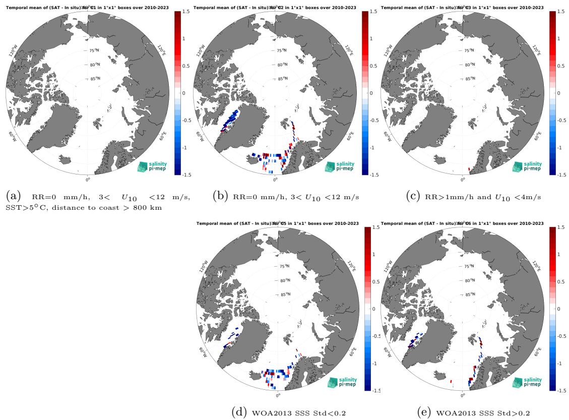
Figure 14: Temporal mean gridded over spatial boxes of size 1^\circ \times 1^\circ of \Delta\text{SSS} (SMOS SSS L2Q v331 - With FLAG (CMEMS-CATDS-CPDC) - TSG (LEGOS-DM)) for 5 different subdatasets corresponding to:RR=0 mm/h, 3 < U_{10} < 12 m/s, SST>5°C, distance to coast > 800 km (a), RR=0 mm/h, 3 < U_{10} < 12 m/s (b), RR>1mm/h and U_{10} < 4 m/s (c), WOA2013 SSS Std<0.2 (d), WOA2013 SSS Std>0.2 (e).
