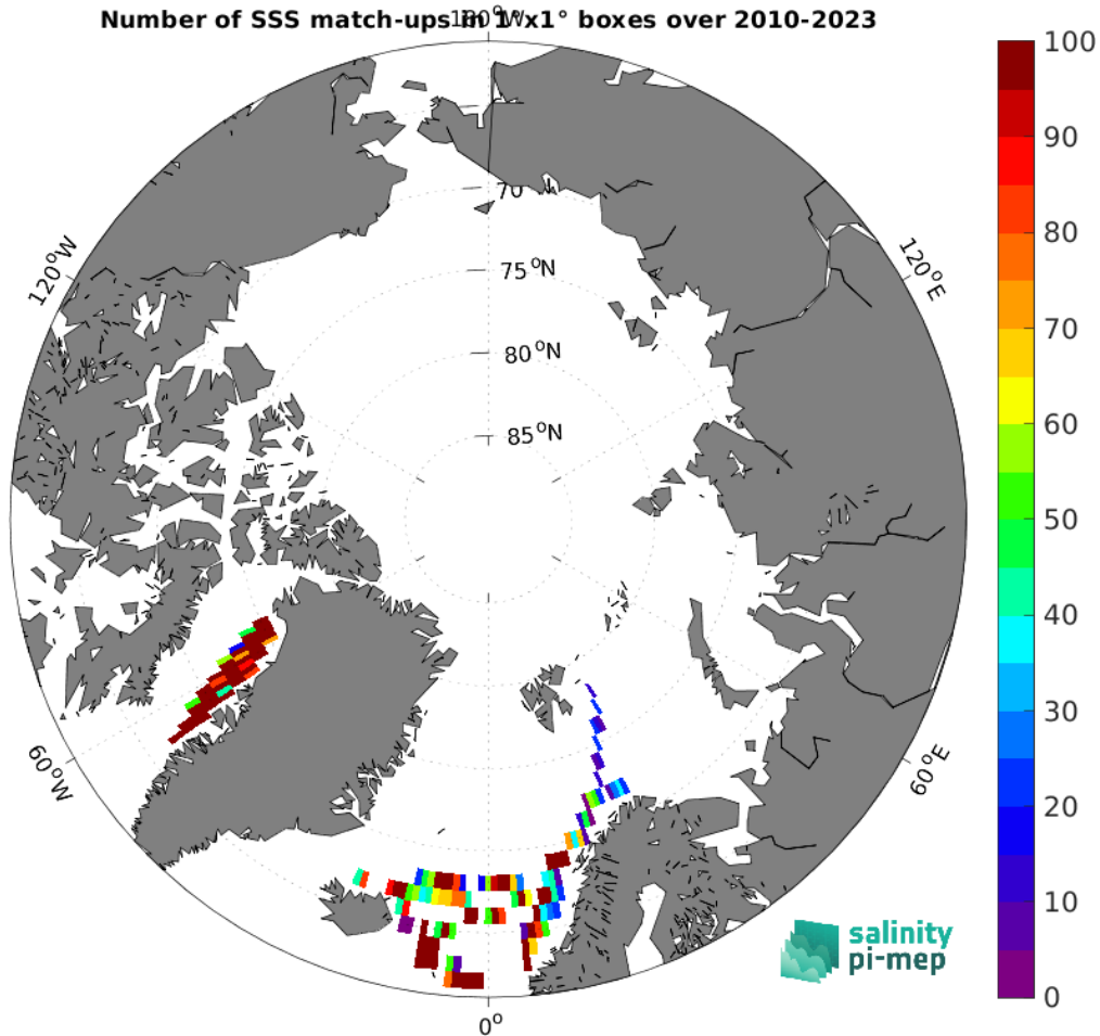
Figure 5: Number of SSS match-ups between TSG (LEGOS-DM) SSS and the SMOS SSS L2Q v331 - With FLAG (CMEMS-CATDS-CPDC) SSS product for the Arctic Ocean Pi-MEP region over 1^\circ \times 1^\circ boxes and for the full satellite product period.
