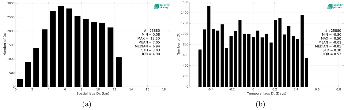
Figure 6: Histograms of the spatial (a) and temporal (b) lags between the location/time of the TSG (LEGOS-DM) measurement and the date of the corresponding SMOS SSS L2Q v331 - With FLAG (CMEMS-CATDS-CPDC) SSS pixel.
