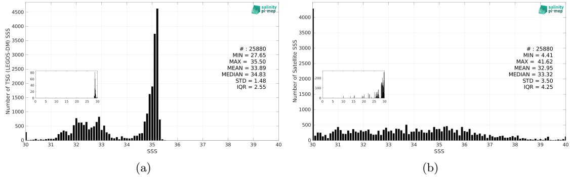
Figure 3: Histograms of SSS from TSG (LEGOS-DM) (a) and SMOS SSS L2Q v331 - With FLAG (CMEMS-CATDS-CPDC) (b) considering all match-up pairs per bins of 0.1 over the Arctic Ocean Pi-MEP region and for the full satellite product period.
