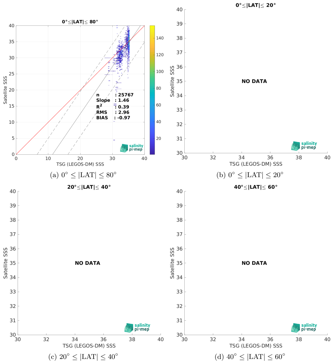
Figure 10: Contour maps of the concentration of SMOS SSS L2Q v331 - With FLAG (CMEMS-CATDS-CPDC) SSS (y-axis) versus TSG (LEGOS-DM) SSS (x-axis) at match-up pairs for different latitude bands. For each plot, the red line shows x=y . The black thin and dashed lines indicate a linear fit through the data cloud and the \pm 95\% confidence levels, respectively. The number match-up pairs n , the slope and R^2 coefficient of the linear fit, the root mean square (RMS) and the mean bias between satellite and in situ data are indicated for each latitude band in each plots.
