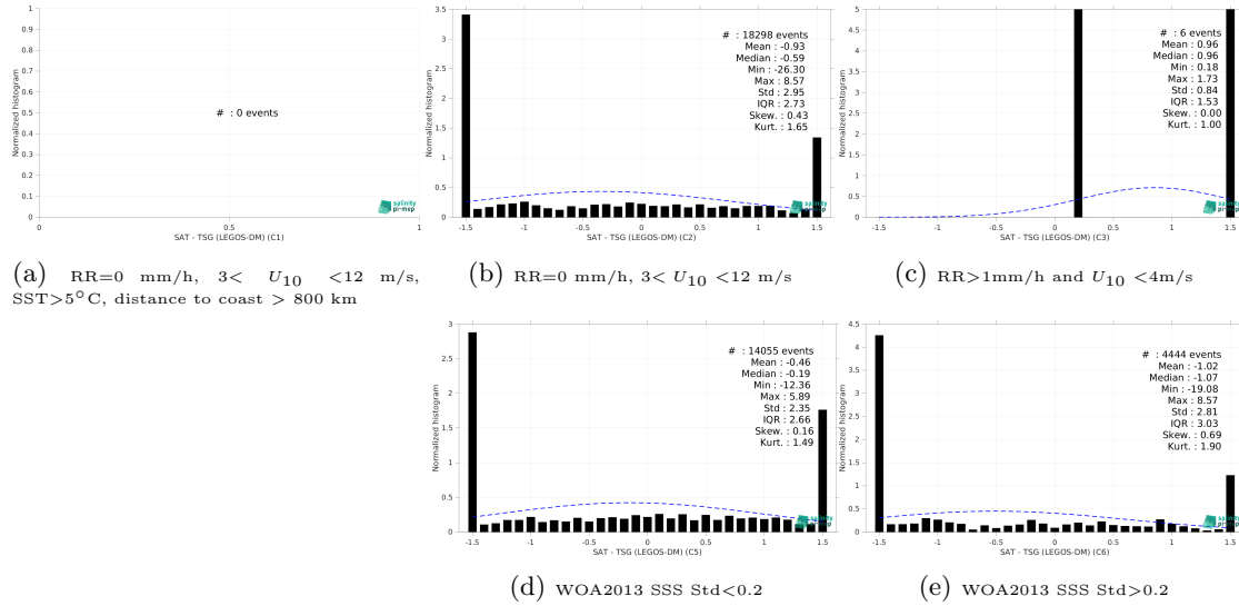
Figure 15: Normalized histogram of \Delta SSS (SMOS SSS L2Q v331 - With FLAG (CMEMS-CATDS-CPDC) - TSG (LEGOS-DM)) for 5 different subdatasets corresponding to: RR=0 mm/h, 3 < U_{10} < 12 m/s, SST > 5°C, distance to coast > 800 km (a), RR=0 mm/h, 3 < U_{10} < 12 m/s (b), RR > 1mm/h and U_{10} < 4 m/s (c), WOA2013 SSS Std < 0.2 (d), WOA2013 SSS Std > 0.2 (e).
