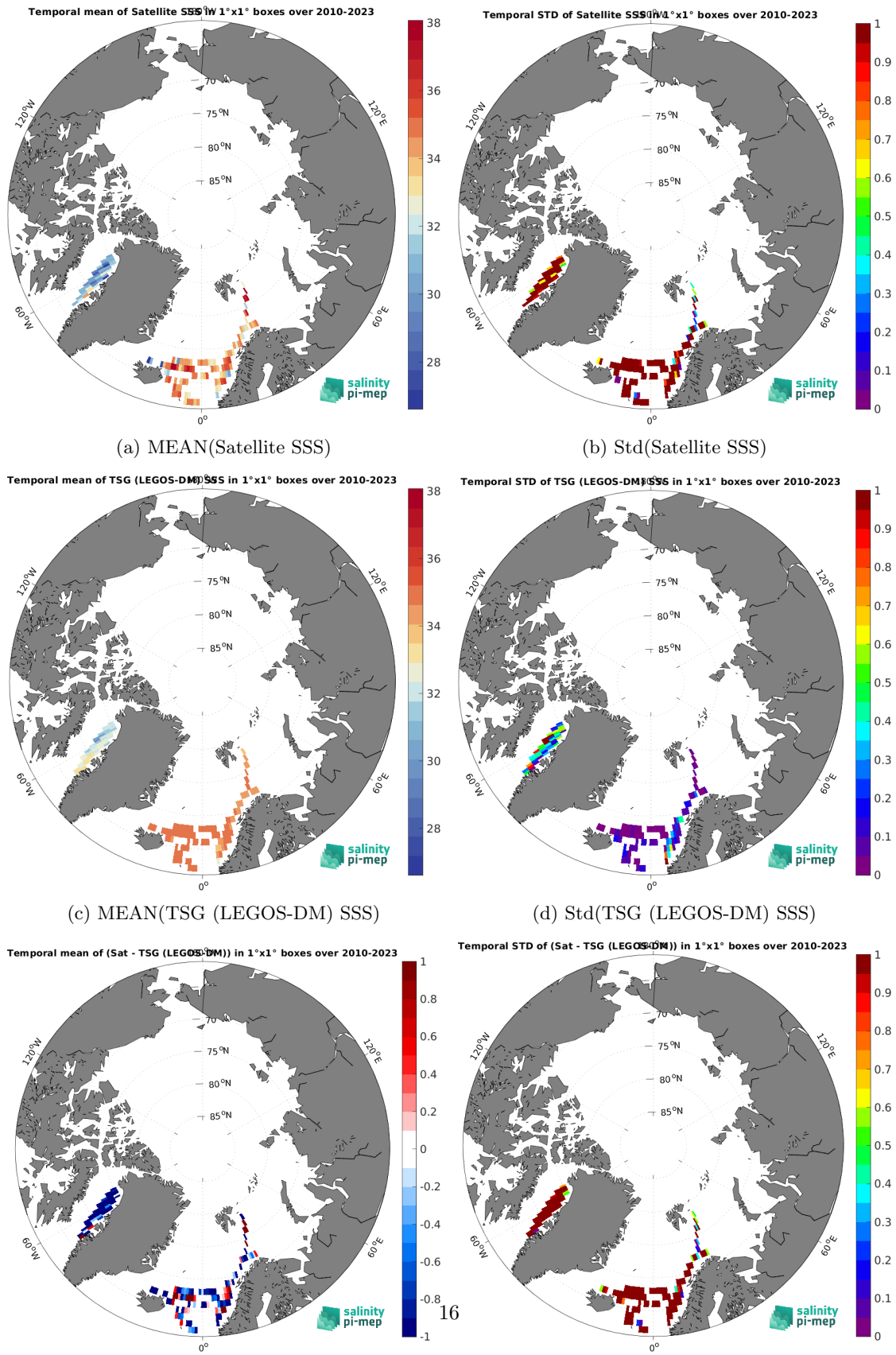
Figure 7: Temporal mean (left) and Std (right) of SSS from SMOS SSS L2Q v331 - With FLAG (CMEMS-CATDS-CPDC) (top), TSG (LEGOS-DM) (middle), and of \Delta SSS (Satellite - TSG (LEGOS-DM)). Only match-up pairs are used to generate these maps.
