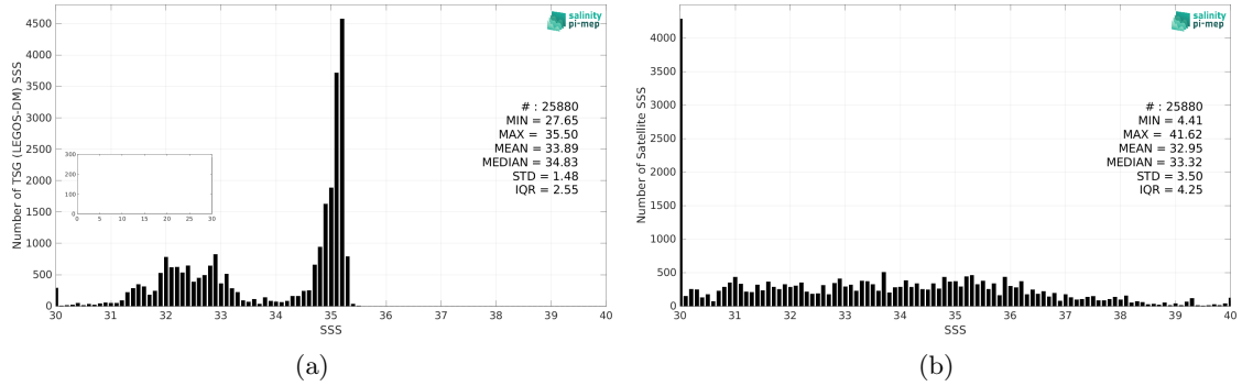
Figure 2: Histograms of SSS from TSG (LEGOS-DM) (a) and SMOS SSS L2Q v331 - With FLAG (CMEMS-CATDS-CPDC) (b) considering all match-up pairs per bins of 0.1 over the Arctic Ocean Pi-MEP region and for the full satellite product period.
