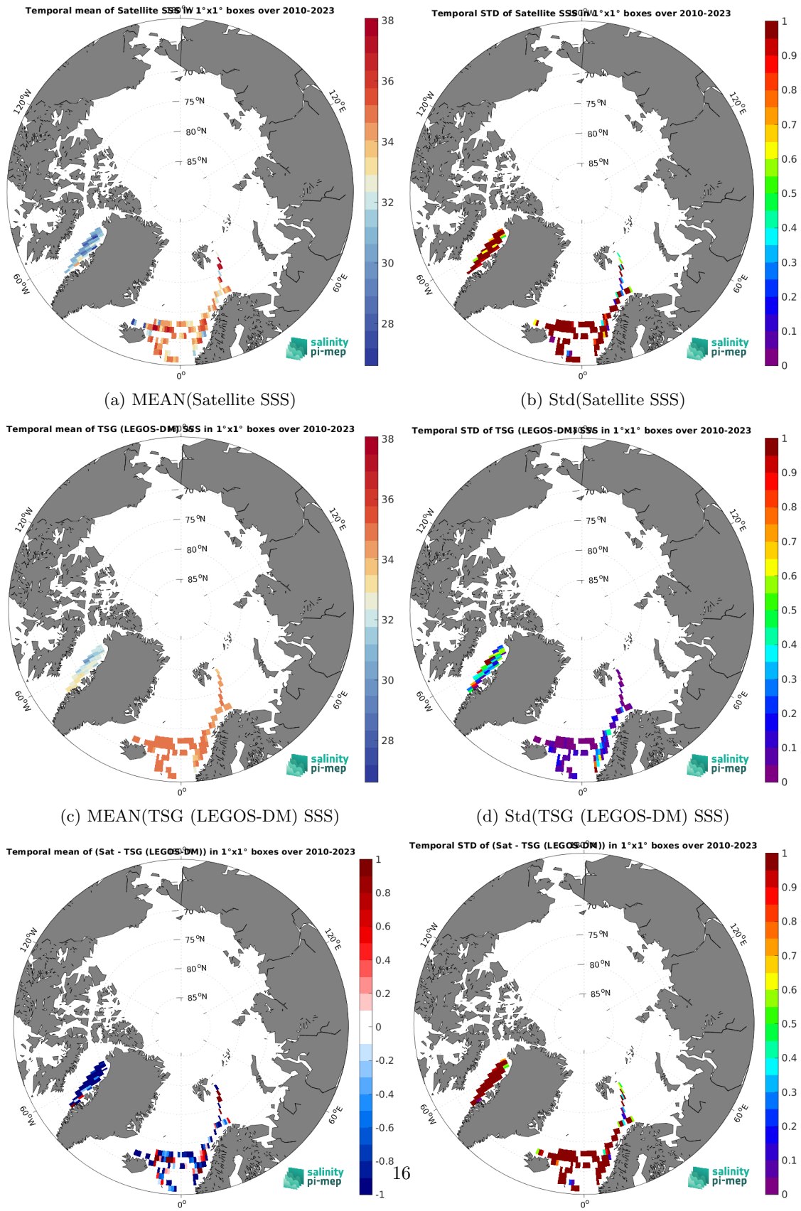
Figure 6: Temporal mean (left) and Std (right) of SSS from SMOS SSS L2Q v331 - With FLAG (CMEMS-CATDS-CPDC) (top), TSG (LEGOS-DM) (middle), and of \Delta SSS (Satellite - TSG (LEGOS-DM)). Only match-up pairs are used to generate these maps.
