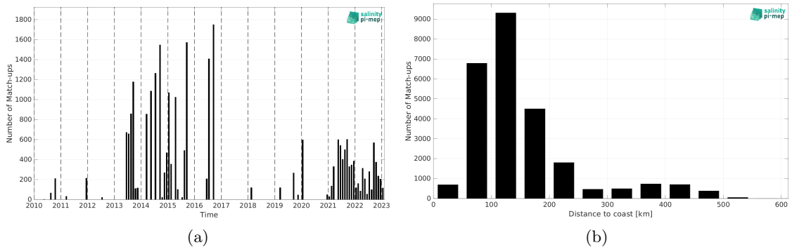
Figure 1: Number of match-ups between TSG (LEGOS-DM) and SMOS SSS L2Q v331 - With FLAG (CMEMS-CATDS-CPDC) SSS as a function of time (a) and as function of the distance to coast (b) over the Arctic Ocean Pi-MEP region and for the full satellite product period.
