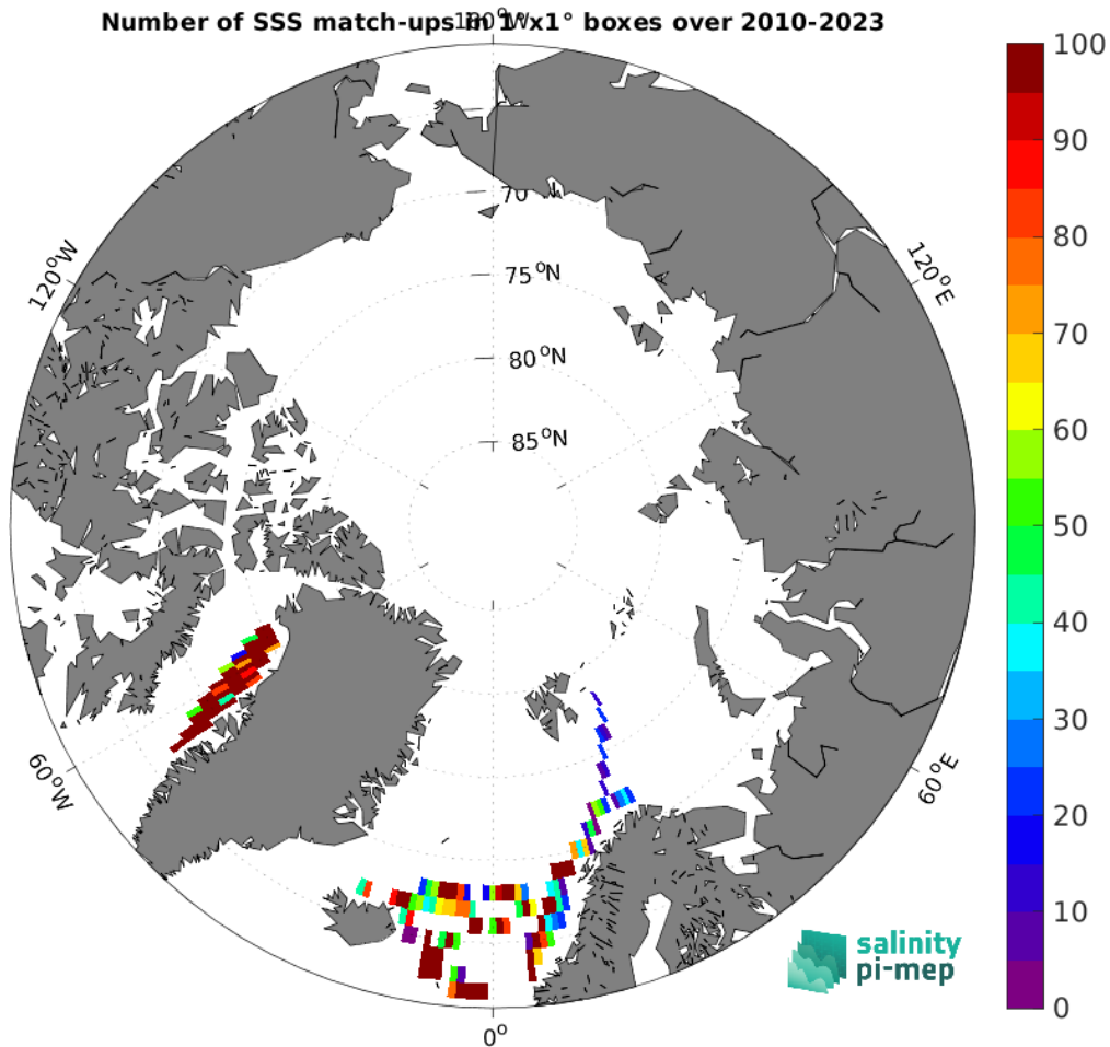
Figure 4: Number of SSS match-ups between TSG (LEGOS-DM) SSS and the SMOS SSS L2Q v331 - With FLAG (CMEMS-CATDS-CPDC) SSS product for the Arctic Ocean Pi-MEP region over 1^\circ \times 1^\circ boxes and for the full satellite product period.
