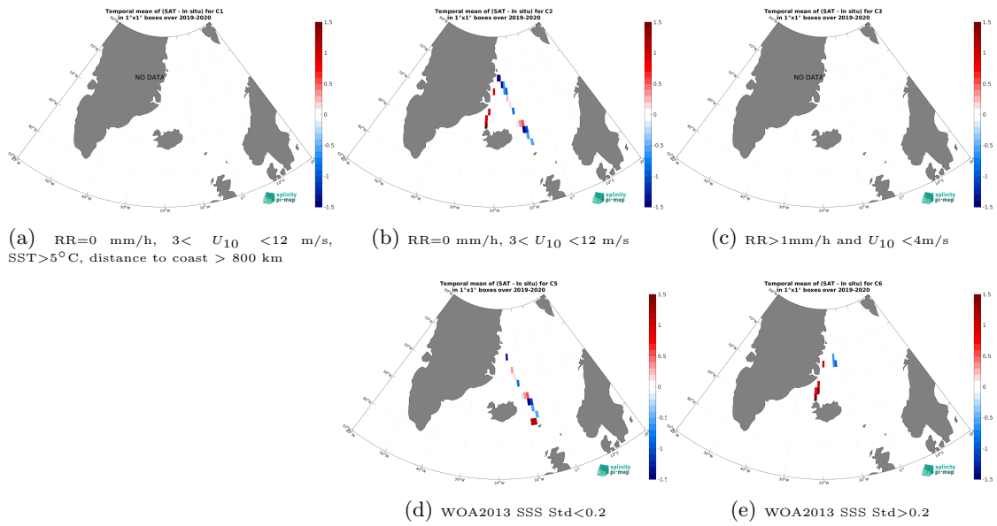
Figure 14: Temporal mean gridded over spatial boxes of size 1^\circ \times 1^\circ of \Delta SSS (SMOS SSS L2Q v331 - With FLAG (CMEMS-CATDS-CPDC) - TSG (Lauge-Koch)) for 5 different subdatasets corresponding to: RR=0 mm/h, 3 < U_{10} < 12 m/s, SST > 5°C, distance to coast > 800 km (a), RR=0 mm/h, 3 < U_{10} < 12 m/s (b), RR > 1mm/h and U_{10} < 4 m/s (c), WOA2013 SSS Std < 0.2 (d), WOA2013 SSS Std > 0.2 (e).
