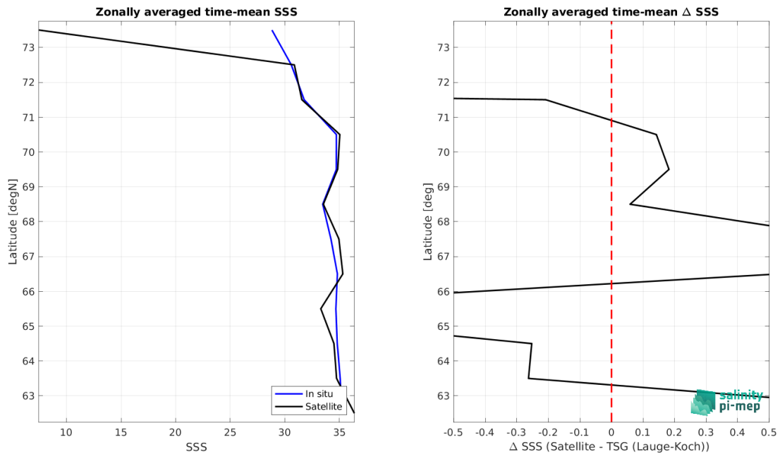
Figure 9: Left panel: Zonal mean SSS from SMOS SSS L2Q v331 - With FLAG (CMEMS-CATDS-CPDC) satellite product (black) and from TSG (Lauge-Koch) (blue). Right panel: Zonal mean of \Delta SSS (Satellite - TSG (Lauge-Koch)) for all the collected Pi-MEP match-up pairs estimated over the full satellite product period.
