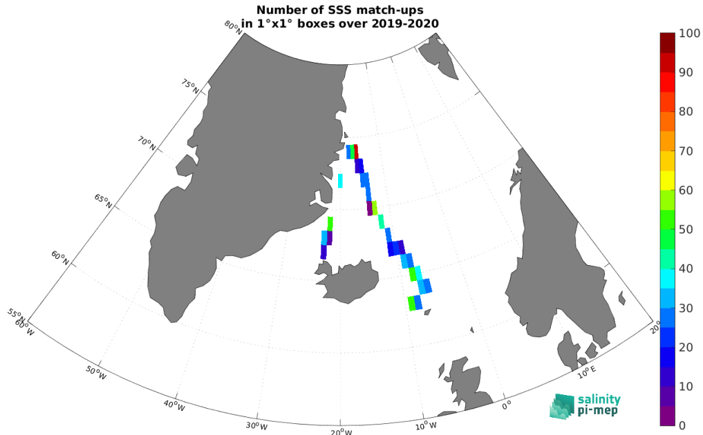
Figure 5: Number of SSS match-ups between TSG (Lauge-Koch) SSS and the SMOS SSS L2Q v331 - With FLAG (CMEMS-CATDS-CPDC) SSS product for the Arctic Ocean Pi-MEP region over 1^\circ \times 1^\circ boxes and for the full satellite product period.
