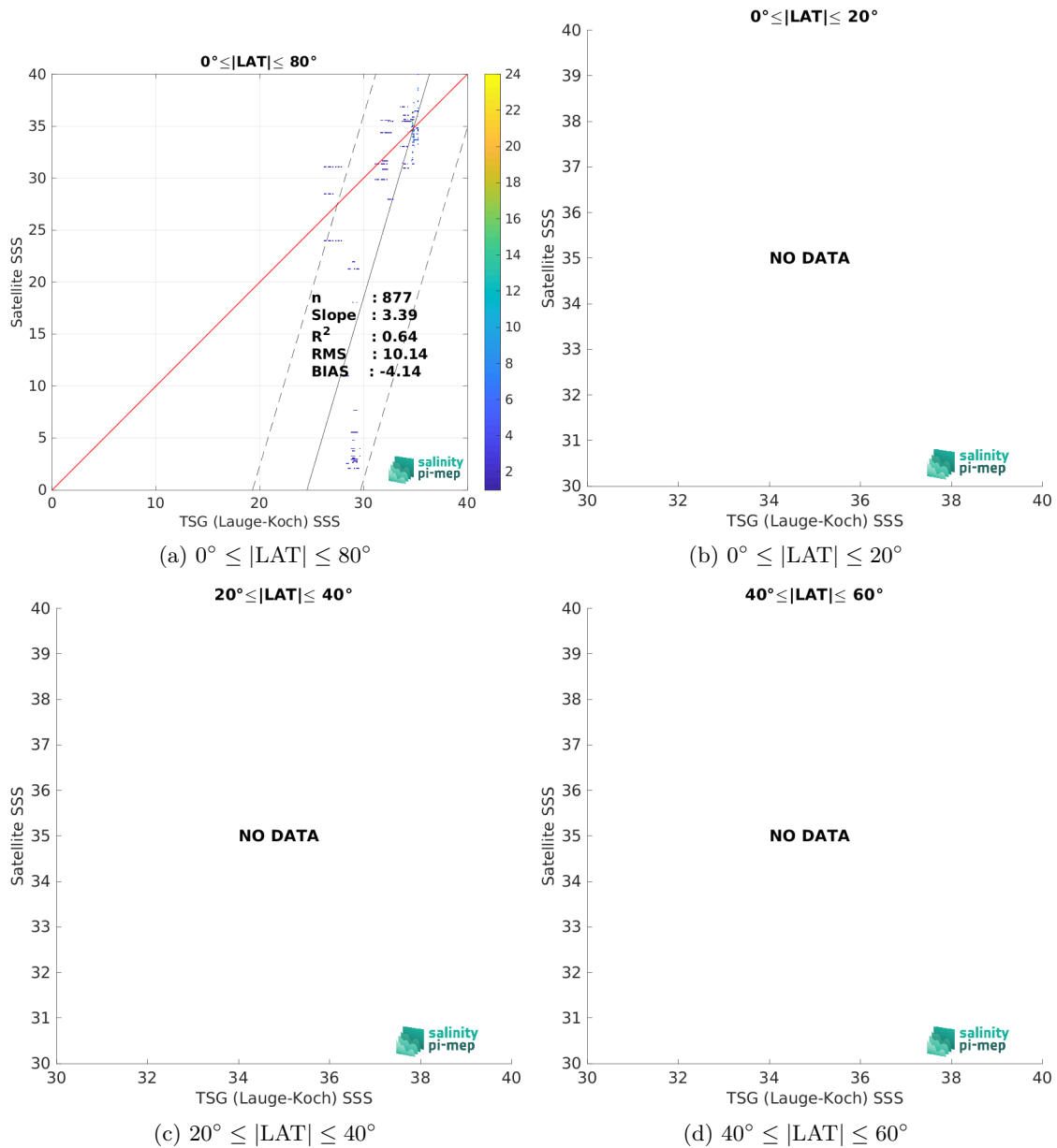
Figure 10: Contour maps of the concentration of SMOS SSS L2Q v331 - With FLAG (CMEMS-CATDS-CPDC) SSS (y-axis) versus TSG (Lauge-Koch) SSS (x-axis) at match-up pairs for different latitude bands. For each plot, the red line shows x=y . The black thin and dashed lines indicate a linear fit through the data cloud and the \pm 95\% confidence levels, respectively. The number match-up pairs n , the slope and R^2 coefficient of the linear fit, the root mean square (RMS) and the mean bias between satellite and in situ data are indicated for each latitude band in each plots.
