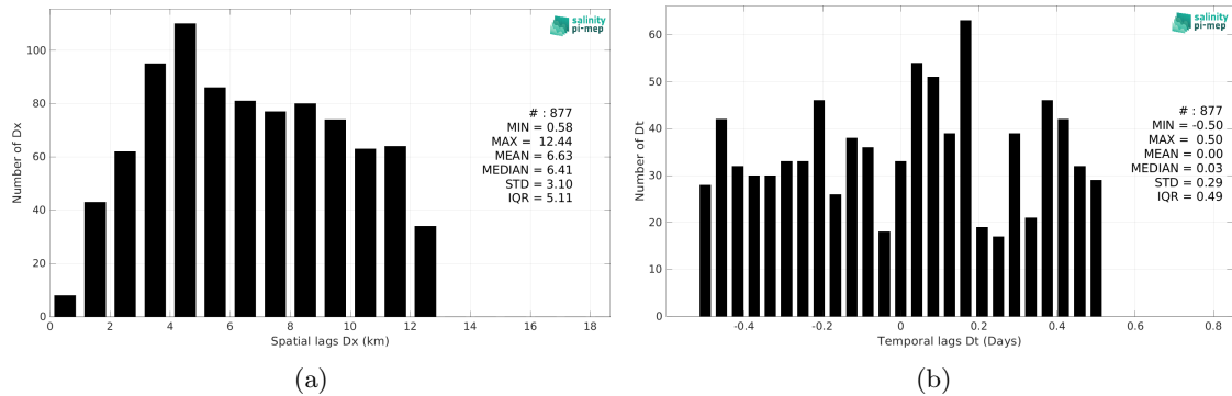
Figure 6: Histograms of the spatial (a) and temporal (b) lags between the location/time of the TSG (Lauge-Koch) measurement and the date of the corresponding SMOS SSS L2Q v331 - With FLAG (CMEMS-CATDS-CPDC) SSS pixel.
