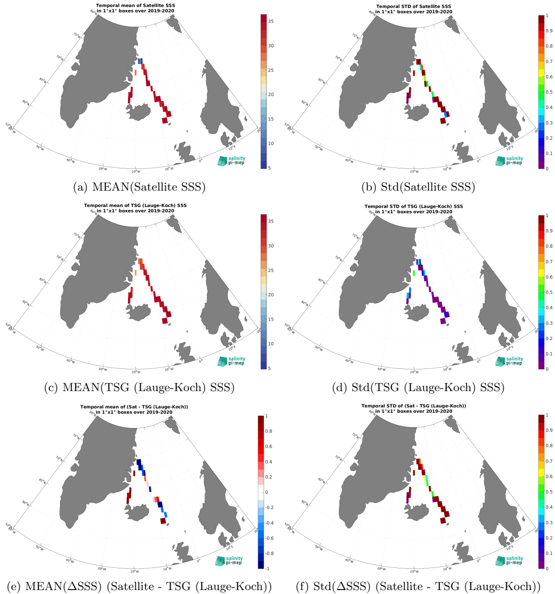
Figure 7: Temporal mean (left) and Std (right) of SSS from SMOS SSS L2Q v331 - With FLAG (CMEMS-CATDS-CPDC) (top), TSG (Lauge-Koch) (middle), and of \Delta SSS (Satellite - TSG (Lauge-Koch)). Only match-up pairs are used to generate these maps.
