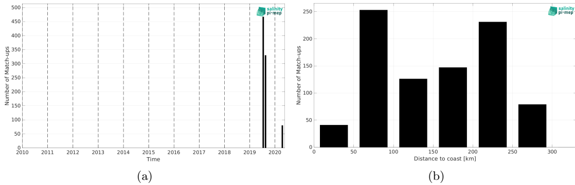
Figure 2: Number of match-ups between TSG (Lauge-Koch) and SMOS SSS L2Q v331 - With FLAG (CMEMS-CATDS-CPDC) SSS as a function of time (a) and as function of the distance to coast (b) over the Arctic Ocean Pi-MEP region and for the full satellite product period.
