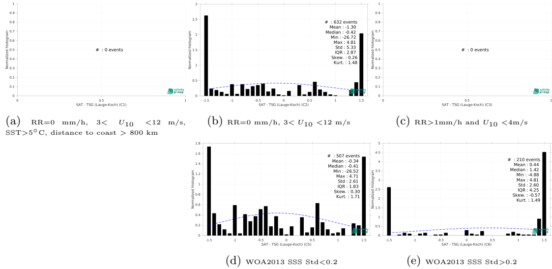
Figure 15: Normalized histogram of \Delta SSS (SMOS SSS L2Q v331 - With FLAG (CMEMS-CATDS-CPDC) - TSG (Lauge-Koch)) for 5 different subdatasets corresponding to: RR=0 mm/h, 3 < U_{10} < 12 m/s, SST > 5°C, distance to coast > 800 km (a), RR=0 mm/h, 3 < U_{10} < 12 m/s (b), RR > 1mm/h and U_{10} < 4 m/s (c), WOA2013 SSS Std < 0.2 (d), WOA2013 SSS Std > 0.2 (e).
