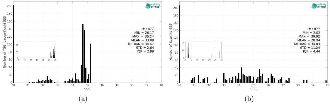
Figure 3: Histograms of SSS from TSG (Lauge-Koch) (a) and SMOS SSS L2Q v331 - With FLAG (CMEMS-CATDS-CPDC) (b) considering all match-up pairs per bins of 0.1 over the Arctic Ocean Pi-MEP region and for the full satellite product period.
