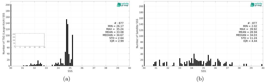
Figure 2: Histograms of SSS from TSG (Lauge-Koch) (a) and SMOS SSS L2Q v331 - With FLAG (CMEMS-CATDS-CPDC) (b) considering all match-up pairs per bins of 0.1 over the Arctic Ocean Pi-MEP region and for the full satellite product period.
