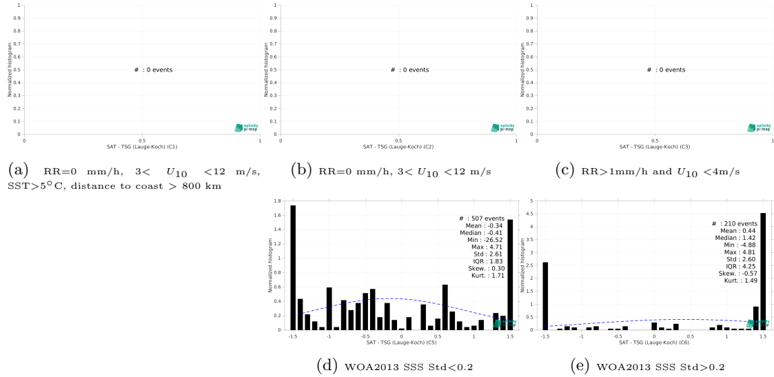
Figure 13: Normalized histogram of \Delta SSS (SMOS SSS L2Q v331 - With FLAG (CMEMS-CATDS-CPDC) - TSG (Laue-Koch)) for 5 different subdatasets corresponding to: RR=0 mm/h, 3 < U_{10} < 12 m/s, SST > 5°C, distance to coast > 800 km (a), RR=0 mm/h, 3 < U_{10} < 12 m/s (b), RR > 1mm/h and U_{10} < 4 m/s (c), WOA2013 SSS Std < 0.2 (d), WOA2013 SSS Std > 0.2 (e).
