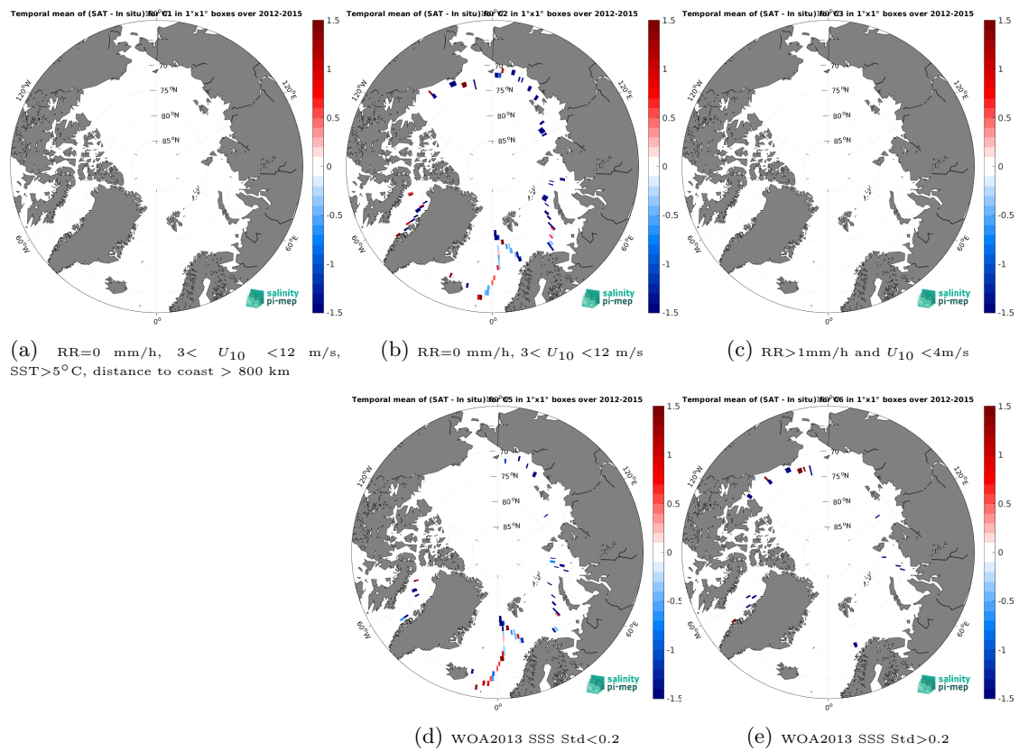
Figure 14: Temporal mean gridded over spatial boxes of size 1^\circ \times 1^\circ of \Delta SSS (SMOS SSS L2Q v331 - With FLAG (CMEMS-CATDS-CPDC) - TSG (GOSUD-Sailing-ship)) for 5 different subdatasets corresponding to:RR=0 mm/h, 3 < U_{10} < 12 m/s, SST>5°C, distance to coast > 800 km (a), RR=0 mm/h, 3 < U_{10} < 12 m/s (b), RR>1mm/h and U_{10} < 4 m/s (c), WOA2013 SSS Std<0.2 (d), WOA2013 SSS Std>0.2 (e).
