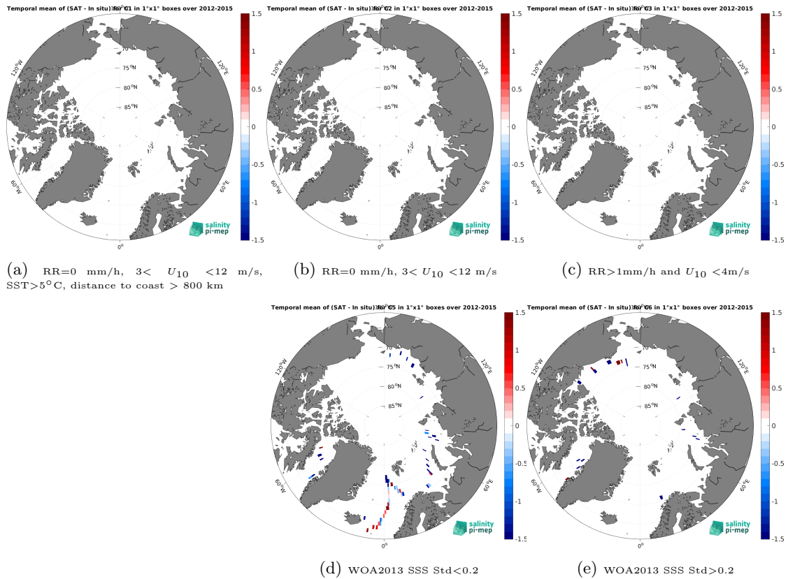
Figure 12: Temporal mean gridded over spatial boxes of size 1^\circ \times 1^\circ of \Delta SSS (SMOS SSS L2Q v331 - With FLAG (CMEMS-CATDS-CPDC) - TSG (GOSUD-Sailing-ship)) for 5 different subdatasets corresponding to: RR=0 mm/h, 3 < U_{10} < 12 m/s, SST>5°C, distance to coast > 800 km (a), RR=0 mm/h, 3 < U_{10} < 12 m/s (b), RR>1mm/h and U_{10} < 4 m/s (c), WOA2013 SSS Std<0.2 (d), WOA2013 SSS Std>0.2 (e).
