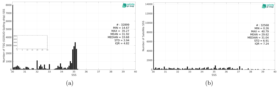
Figure 2: Histograms of SSS from TSG (GOSUD-Sailing-ship) (a) and SMOS SSS L2Q v331 - With FLAG (CMEMS-CATDS-CPDC) (b) considering all match-up pairs per bins of 0.1 over the Arctic Ocean Pi-MEP region and for the full satellite product period.
