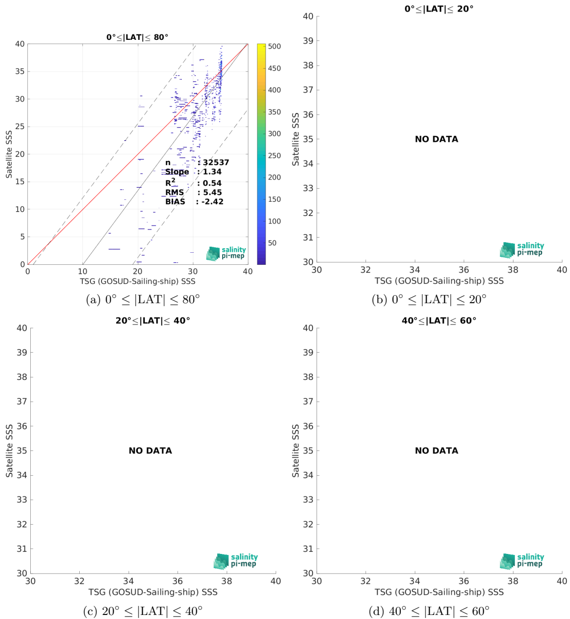
Figure 9: Contour maps of the concentration of SMOS SSS L2Q v331 - With FLAG (CMEMS-CATDS-CPDC) SSS (y-axis) versus TSG (GOSUD-Sailing-ship) SSS (x-axis) at match-up pairs for different latitude bands. For each plot, the red line shows x=y . The black thin and dashed lines indicate a linear fit through the data cloud and the \pm 95\% confidence levels, respectively. The number match-up pairs n , the slope and R^2 coefficient of the linear fit, the root mean square (RMS) and the mean bias between satellite and in situ data are indicated for each latitude band in each plots.
