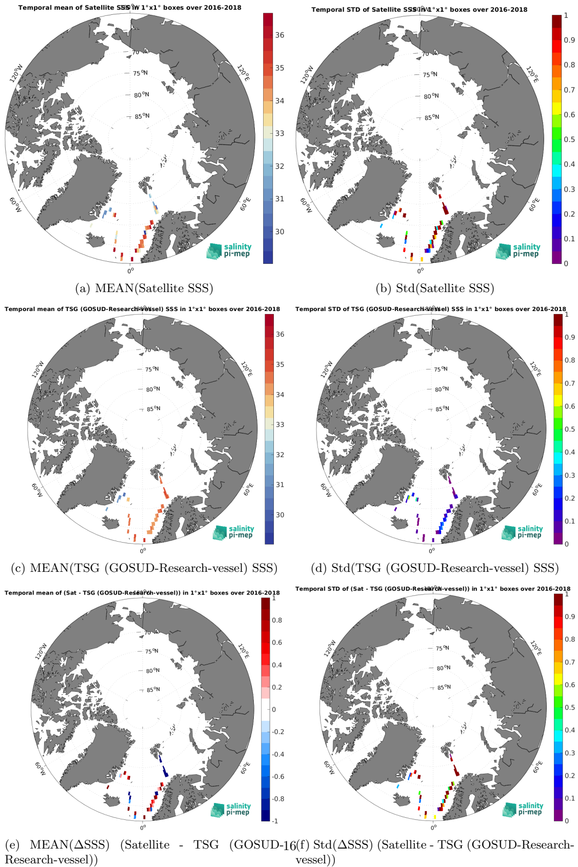
Figure 7: Temporal mean (left) and Std (right) of SSS from SMOS SSS L2Q v331 - With FLAG (CMEMS-CATDS-CPDC) (top), TSG (GOSUD-Research-vessel) (middle), and of \Delta SSS (Satellite - TSG (GOSUD-Research-vessel)). Only match-up pairs are used to generate these maps.
