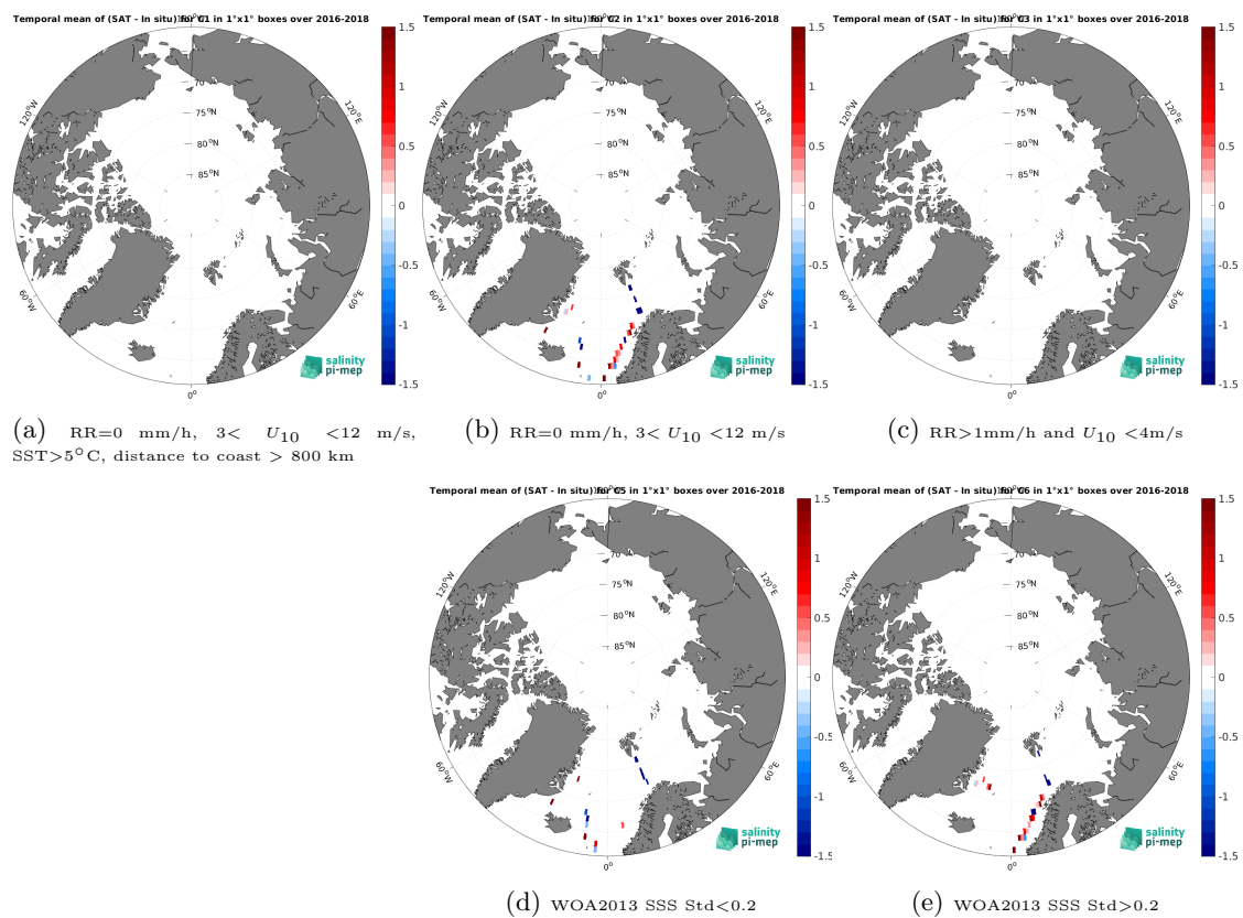
Figure 14: Temporal mean gridded over spatial boxes of size 1^\circ \times 1^\circ of \Delta\text{SSS} (SMOS SSS L2Q v331 - With FLAG (CMEMS-CATDS-CPDC) - TSG (GOSUD-Research-vessel)) for 5 different subdatasets corresponding to:RR=0 mm/h, 3 < U_{10} < 12 m/s, SST>5°C, distance to coast > 800 km (a), RR=0 mm/h, 3 < U_{10} < 12 m/s (b), RR>1mm/h and U_{10} < 4 m/s (c), WOA2013 SSS Std<0.2 (d), WOA2013 SSS Std>0.2 (e).
