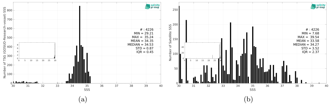
Figure 3: Histograms of SSS from TSG (GOSUD-Research-vessel) (a) and SMOS SSS L2Q v331 - With FLAG (CMEMS-CATDS-CPDC) (b) considering all match-up pairs per bins of 0.1 over the Arctic Ocean Pi-MEP region and for the full satellite product period.
