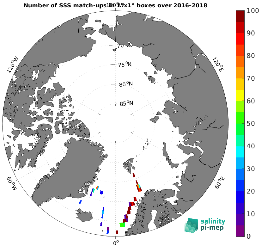
Figure 5: Number of SSS match-ups between TSG (GOSUD-Research-vessel) SSS and the SMOS SSS L2Q v331 - With FLAG (CMEMS-CATDS-CPDC) SSS product for the Arctic Ocean Pi-MEP region over 1^\circ \times 1^\circ boxes and for the full satellite product period.
