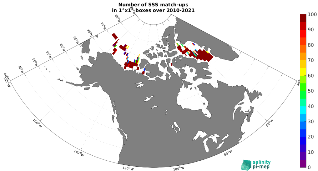
Figure 5: Number of SSS match-ups between TSG (Amundsen) SSS and the SMOS SSS L2Q v331 - With FLAG (CMEMS-CATDS-CPDC) SSS product for the Arctic Ocean Pi-MEP region over 1^\circ \times 1^\circ boxes and for the full satellite product period.
