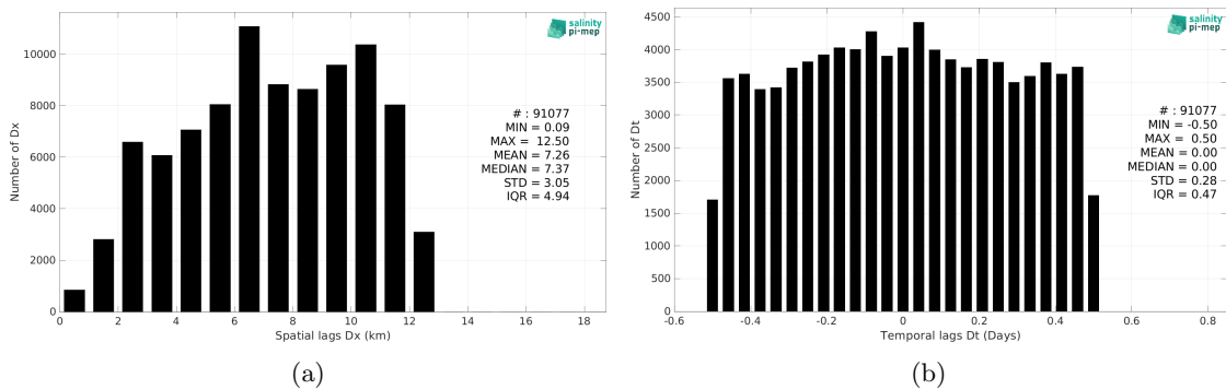
Figure 6: Histograms of the spatial (a) and temporal (b) lags between the location/time of the TSG (Amundsen) measurement and the date of the corresponding SMOS SSS L2Q v331 - With FLAG (CMEMS-CATDS-CPDC) SSS pixel.
