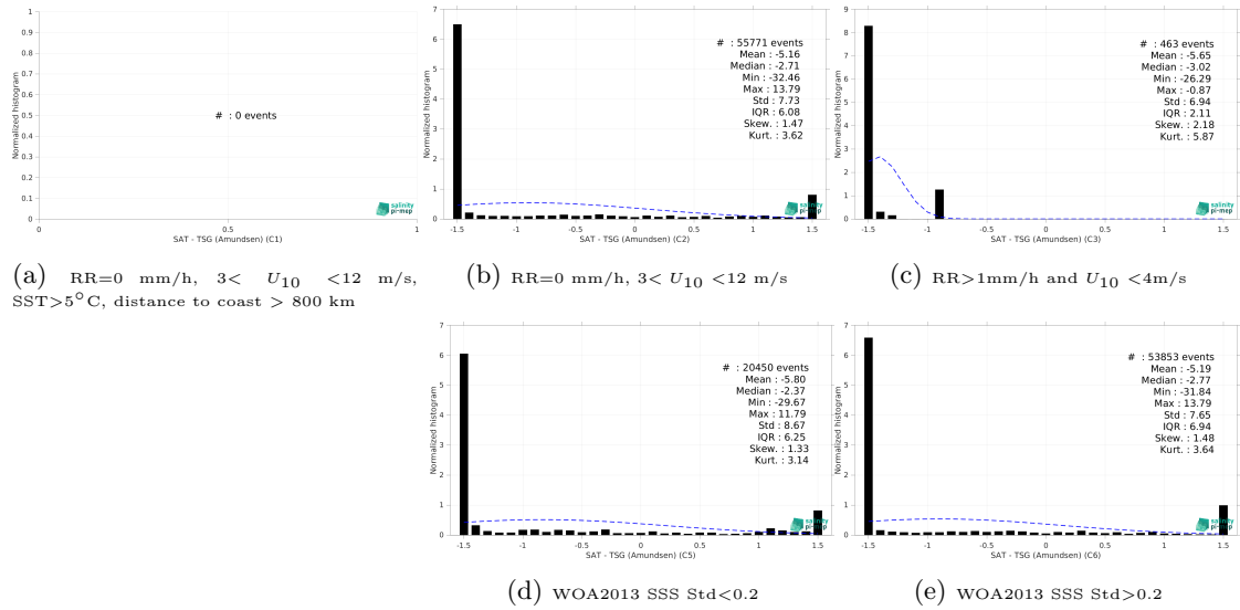
Figure 15: Normalized histogram of \Delta SSS (SMOS SSS L2Q v331 - With FLAG (CMEMS-CATDS-CPDC) - TSG (Amundsen)) for 5 different subdatasets corresponding to: RR=0 mm/h, 3 < U_{10} < 12 m/s, SST > 5°C, distance to coast > 800 km (a), RR=0 mm/h, 3 < U_{10} < 12 m/s (b), RR > 1mm/h and U_{10} < 4 m/s (c), WOA2013 SSS Std < 0.2 (d), WOA2013 SSS Std > 0.2 (e).
