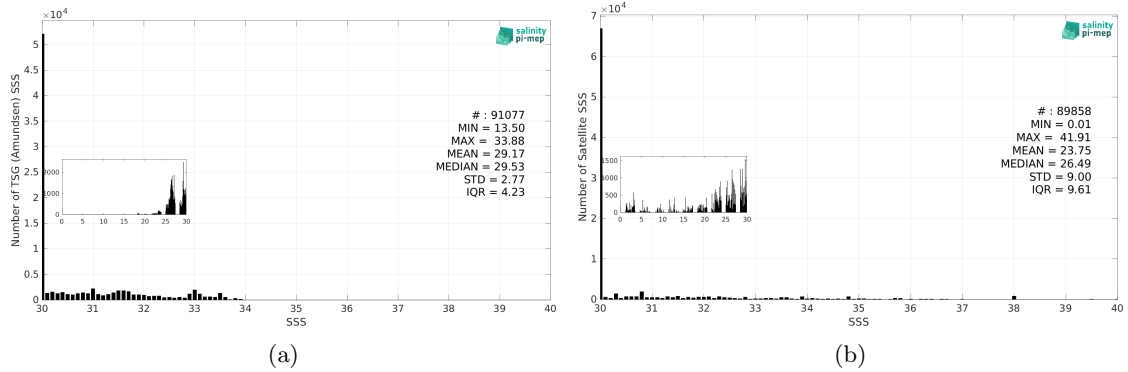
Figure 3: Histograms of SSS from TSG (Amundsen) (a) and SMOS SSS L2Q v331 - With FLAG (CMEMS-CATDS-CPDC) (b) considering all match-up pairs per bins of 0.1 over the Arctic Ocean Pi-MEP region and for the full satellite product period.
