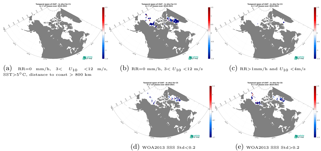
Figure 14: Temporal mean gridded over spatial boxes of size 1^\circ \times 1^\circ of \Delta SSS (SMOS SSS L2Q v331 - With FLAG (CMEMS-CATDS-CPDC) - TSG (Amundsen)) for 5 different subdatasets corresponding to:RR=0 mm/h, 3 < U_{10} < 12 m/s, SST > 5^\circ\text{C} , distance to coast > 800 km (a), RR=0 mm/h, 3 < U_{10} < 12 m/s (b), RR > 1 mm/h and U_{10} < 4 m/s (c), WOA2013 SSS Std < 0.2 (d), WOA2013 SSS Std > 0.2 (e).
