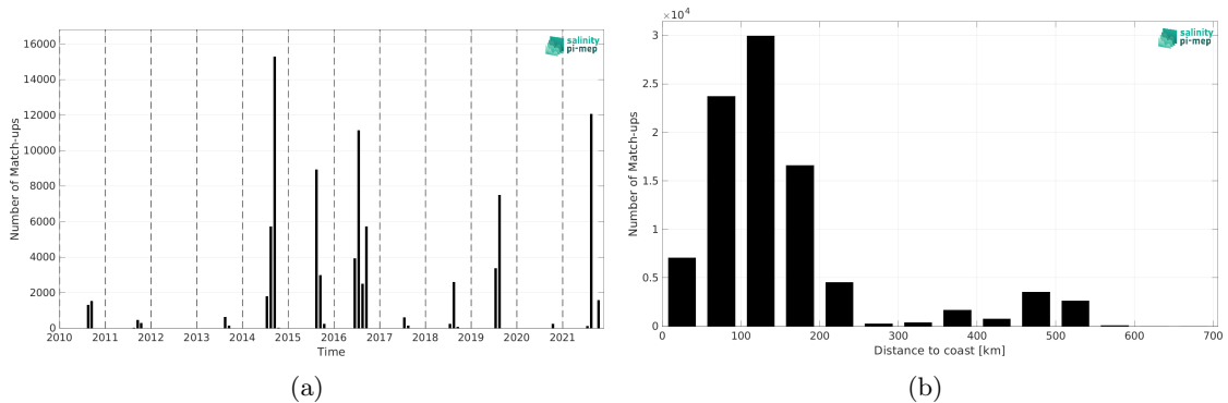
Figure 2: Number of match-ups between TSG (Amundsen) and SMOS SSS L2Q v331 - With FLAG (CMEMS-CATDS-CPDC) SSS as a function of time (a) and as function of the distance to coast (b) over the Arctic Ocean Pi-MEP region and for the full satellite product period.
