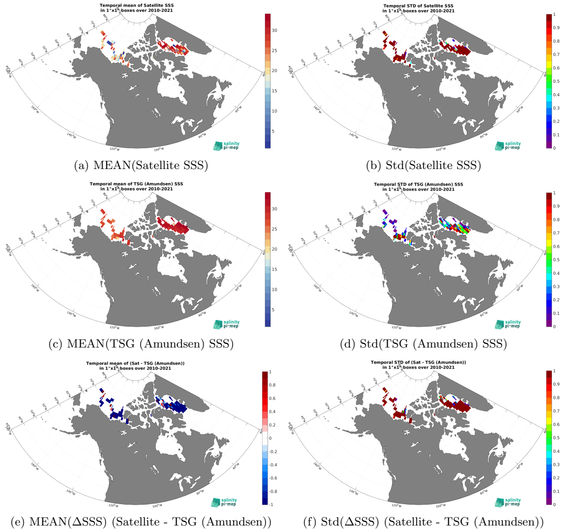
Figure 7: Temporal mean (left) and Std (right) of SSS from SMOS SSS L2Q v331 - With FLAG (CMEMS-CATDS-CPDC) (top), TSG (Amundsen) (middle), and of \Delta SSS (Satellite - TSG (Amundsen)). Only match-up pairs are used to generate these maps.
