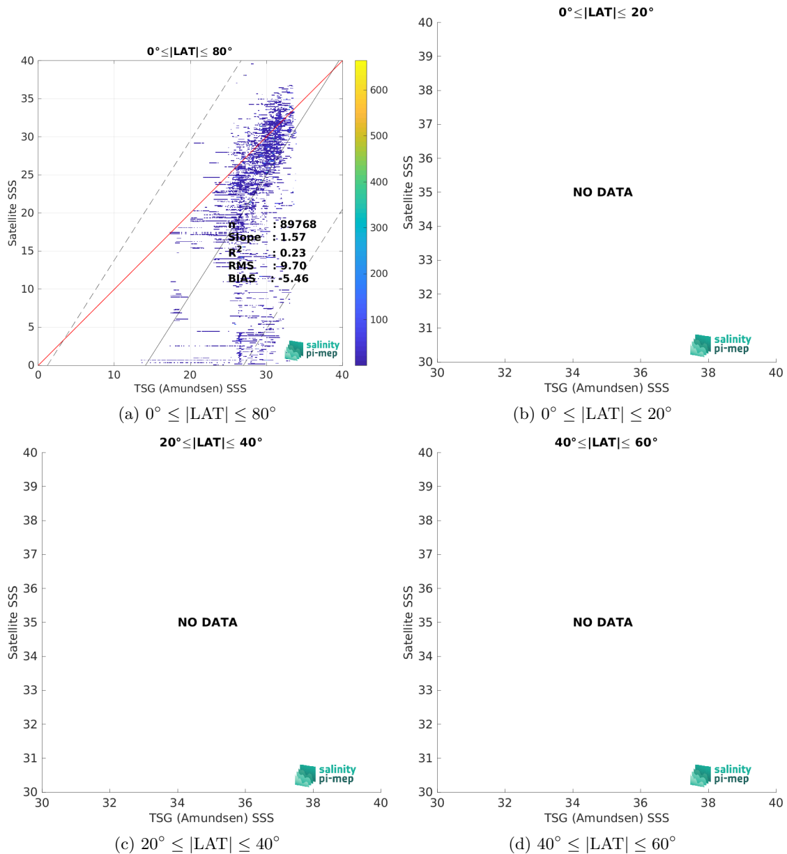
Figure 10: Contour maps of the concentration of SMOS SSS L2Q v331 - With FLAG (CMEMS-CATDS-CPDC) SSS (y-axis) versus TSG (Amundsen) SSS (x-axis) at match-up pairs for different latitude bands. For each plot, the red line shows x=y . The black thin and dashed lines indicate a linear fit through the data cloud and the \pm 95\% confidence levels, respectively. The number match-up pairs n , the slope and R^2 coefficient of the linear fit, the root mean square (RMS) and the mean bias between satellite and in situ data are indicated for each latitude band in each plots.
